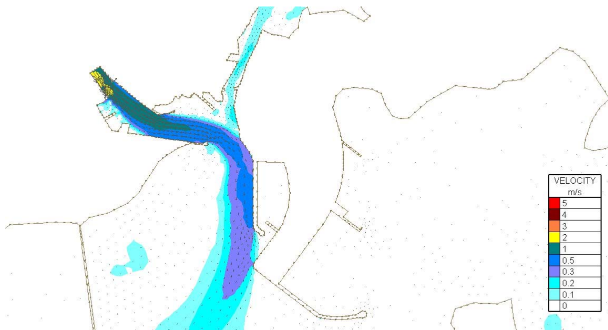
Figure Error! No text of specified style in document..160 Velocity Magnitudes at highwater for Flood Simulation 1– 100 year river flow and mean spring tide – Proposed Harbour Extension Case
