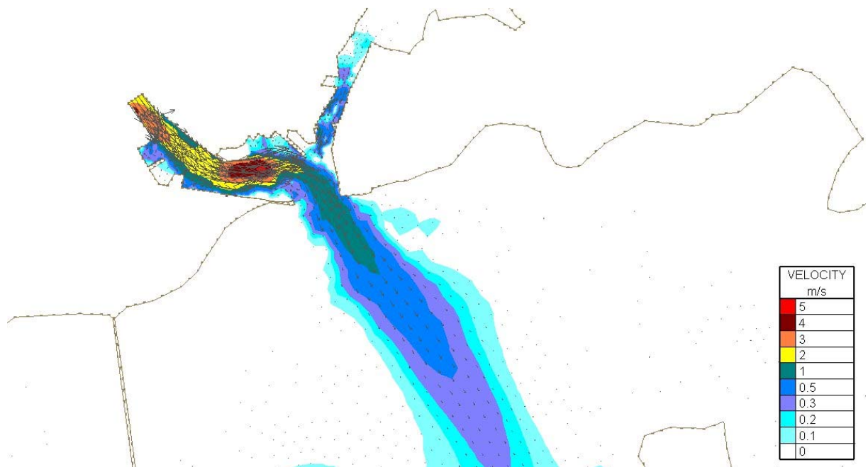
Figure Error! No text of specified style in document..155 Velocity Magnitudes at Low Water (6.2hrs after highwater Tide) for Flood Simulation 1- 100 year river flow and mean spring tide – Existing Case
