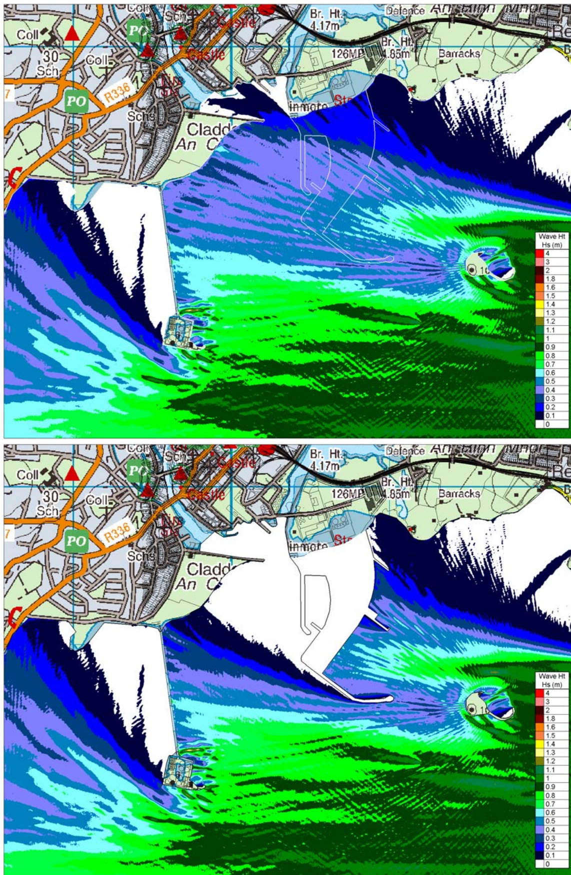
Figure Error! No text of specified style in document..140 ARTEMIS Significant Wave Heights for local Design Storm Waves from the East for Existing and Proposed Case
