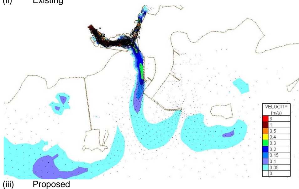
Figure Error! No text of specified style in document..109 Low-Water Velocities – Spring Tide Median Flow
