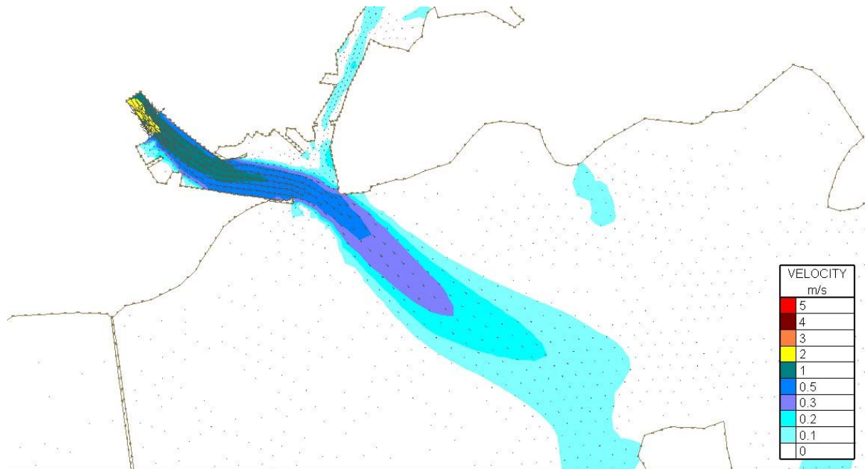
Figure Error! No text of specified style in document..159 Velocity Magnitudes at highwater for Flood Simulation 1 – 100 year river flow and mean spring tide – Existing Case
