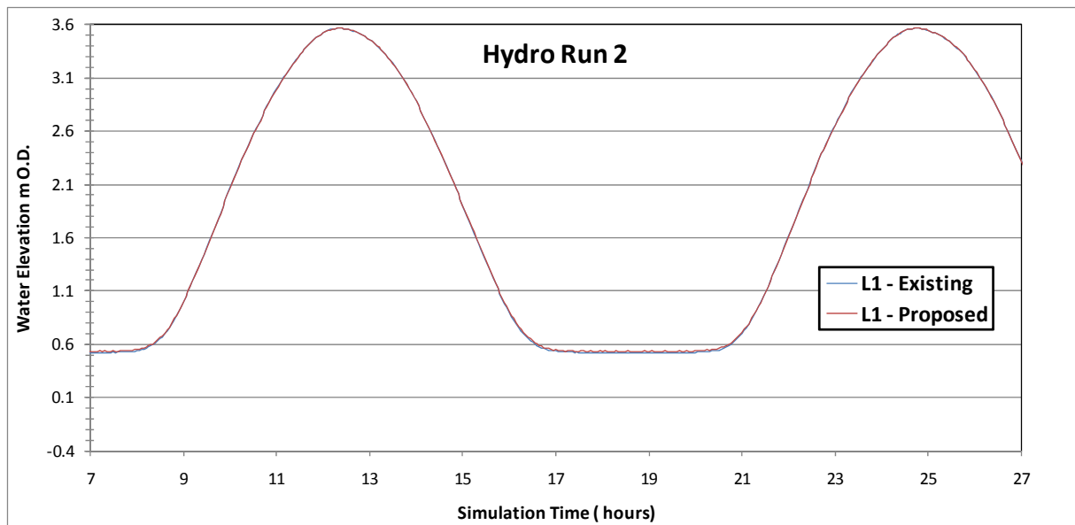
Figure Error! No text of specified style in document..192 Flood level comparison between existing and proposed for Hydrodynamic Simulation No. 2 at reference site 1 in Claddagh Basin adjacent to Spanish Arch
