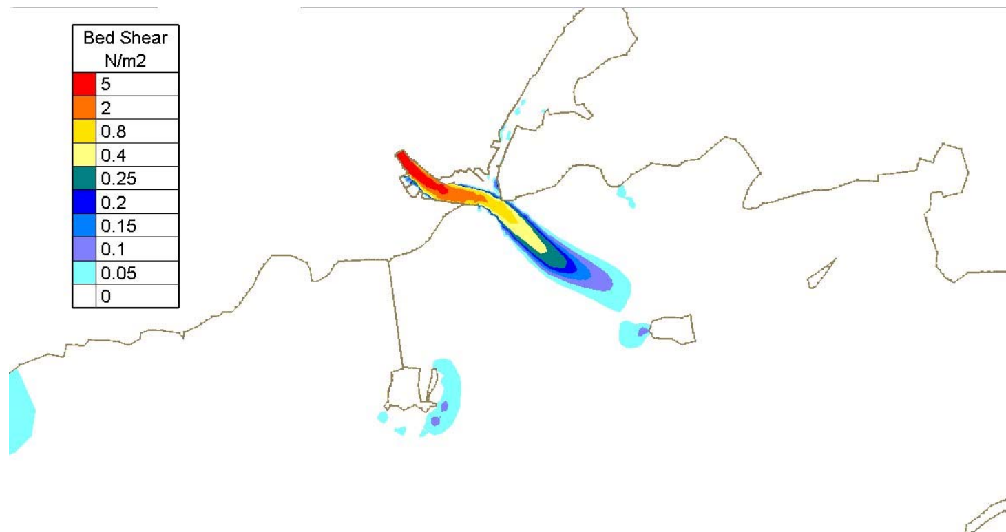
Figure Error! No text of specified style in document..39 - Computed bed shear at High Water Spring Tide with 100 year Corrib Flood Flow for existing case
