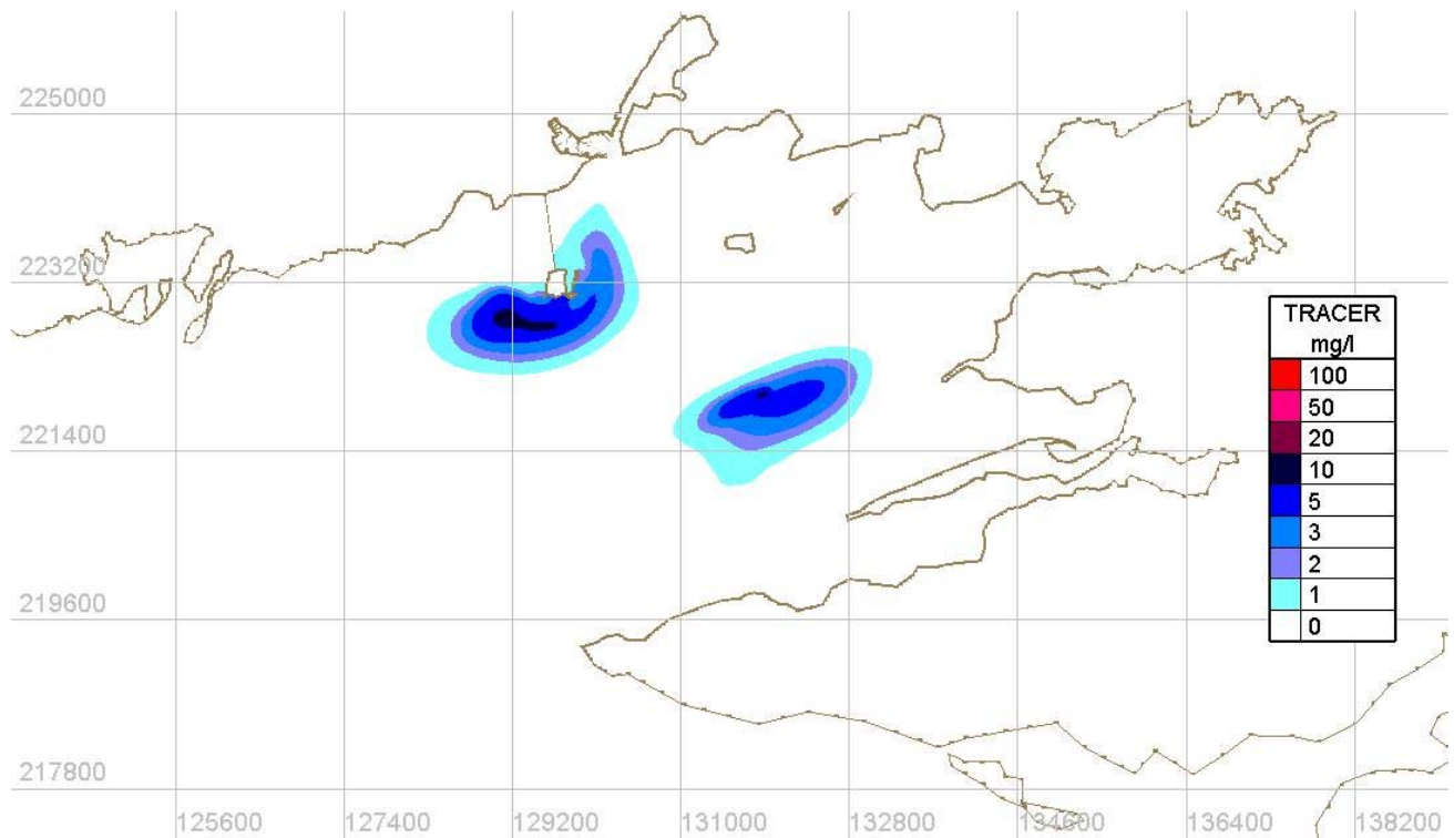
Figure Error! No text of specified style in document..100 Mid-ebb Existing Case - Neap tides
