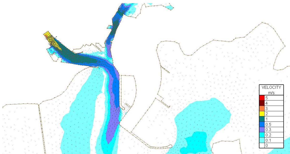
Figure Error! No text of specified style in document..166 Velocity Magnitudes at Mid Flood (3.1hrs before highwater Tide) for Flood Simulation 2 – 100 year river flow and a 3.49m tide – Proposed Harbour Extension Case
