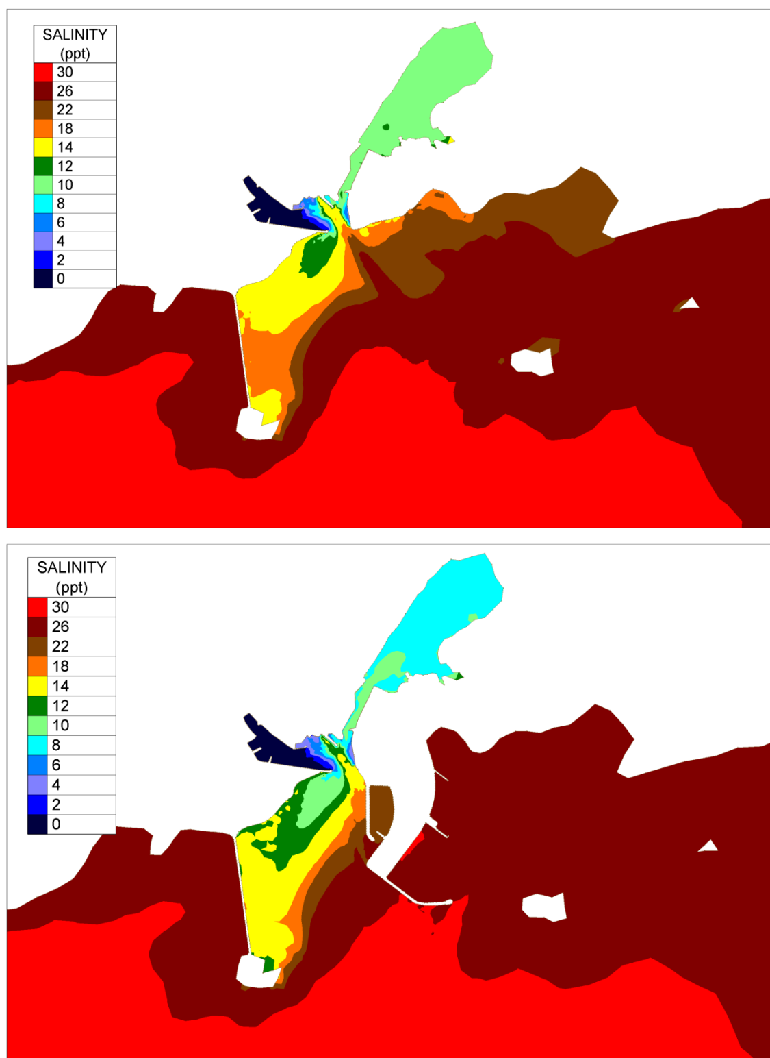
Figure Error! No text of specified style in document..84 Mean Salinity concentration in mid-depth layer for existing and proposed cases under 50-percentile Corrib Flow (82 cumec)
