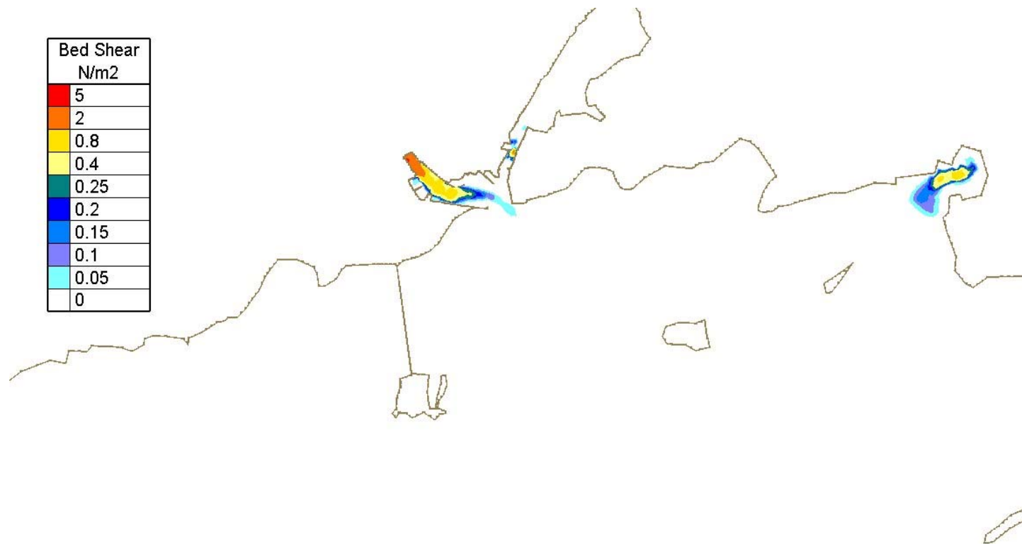
Figure Error! No text of specified style in document..29 - Computed bed shear at mid-flood for existing case without development – Neap Tide and Median River Corrib Flow (82 m 3 /s)
