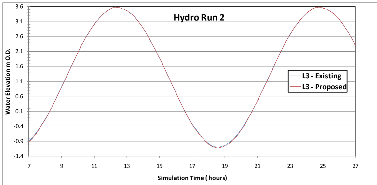
Figure Error! No text of specified style in document..194 Flood level comparison between existing and proposed for Hydrodynamic Simulation No. 2 at reference site 3 in estuary inside Nimmo's Pier
