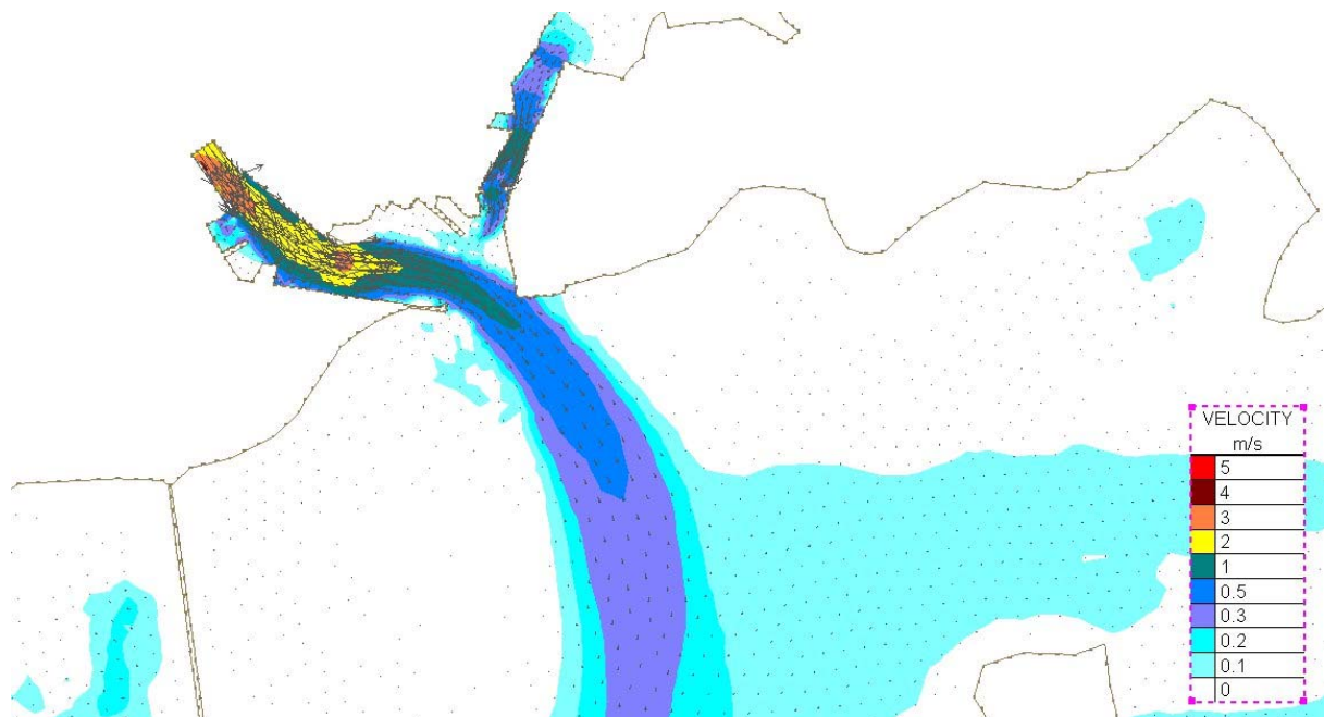
Figure Error! No text of specified style in document..153 Velocity Magnitudes at Mid-ebb (3.1hrs after highwater ) for Flood Simulation 1- 100 year river flow and mean spring tide– Existing Case
