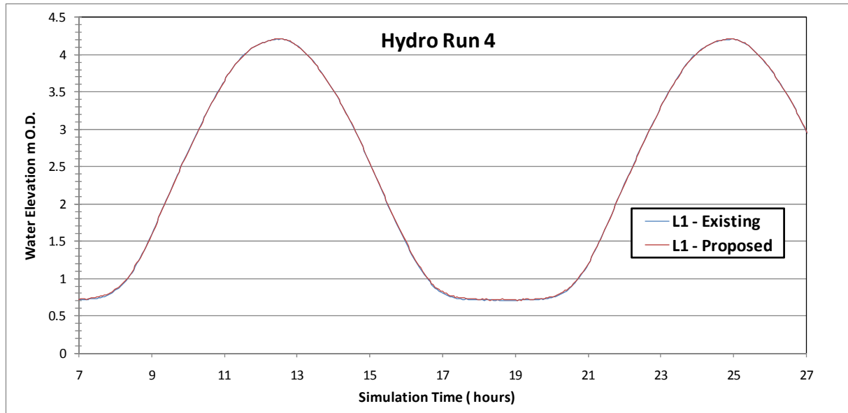
Figure Error! No text of specified style in document..204 Flood level comparison between existing and proposed for Hydrodynamic Simulation No. 4 at reference site 1 in Claddagh Basin adjacent to Spanish Arch
