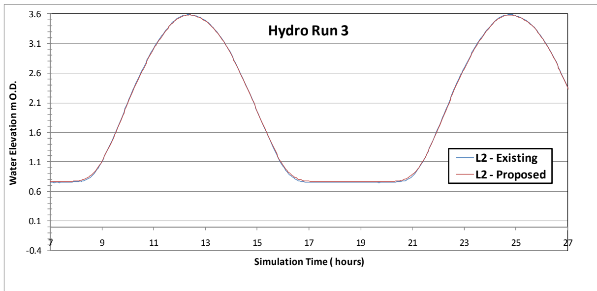
Figure Error! No text of specified style in document..199 Flood level comparison between existing and proposed for Hydrodynamic Simulation No. 3 at reference site 2 in Claddagh Basin
