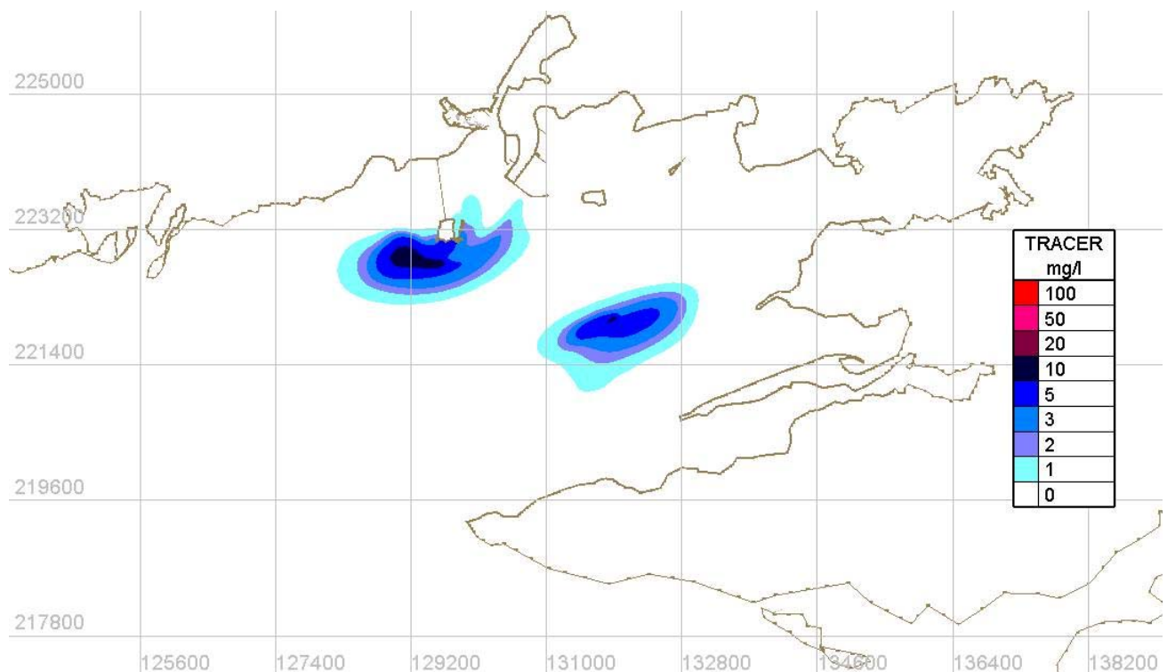
Figure Error! No text of specified style in document..101 Mid-ebb Proposed Case - Neap tides
