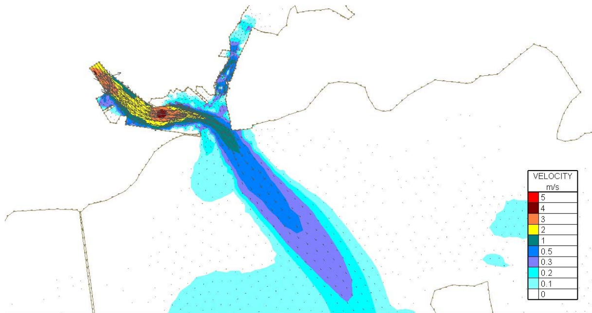
Figure Error! No text of specified style in document..163 Velocity Magnitudes at Low Water (6.2hrs after highwater Tide) for Flood Simulation 2- 100 year river flow and a 3.49m tide – Existing Case
