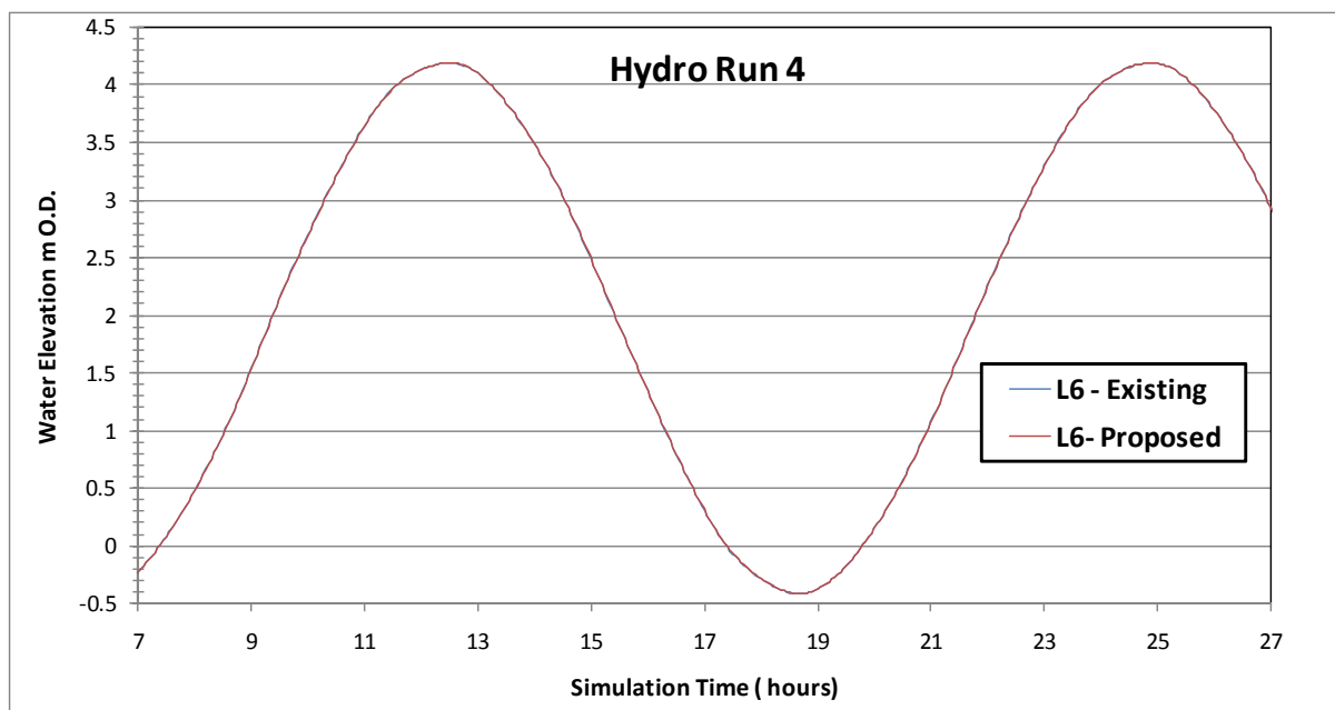
Figure Error! No text of specified style in document..209 Flood level comparison between existing and proposed for Hydrodynamic Simulation No. 4 at reference site 6 – new dredge channel south of Marina entrance
