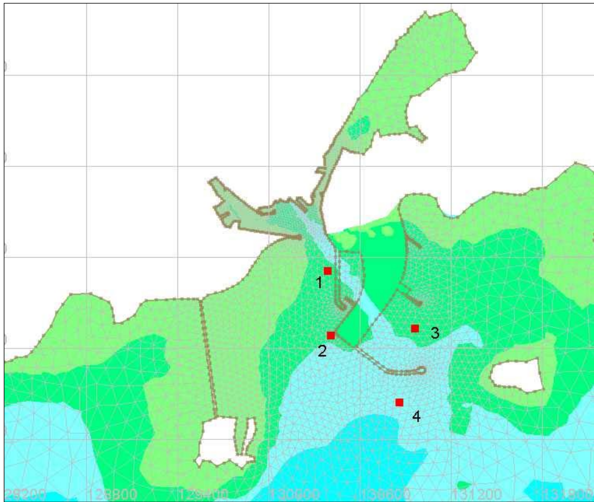
Figure Error! No text of specified style in document..42 - Dredging locations for sediment plume simulations
