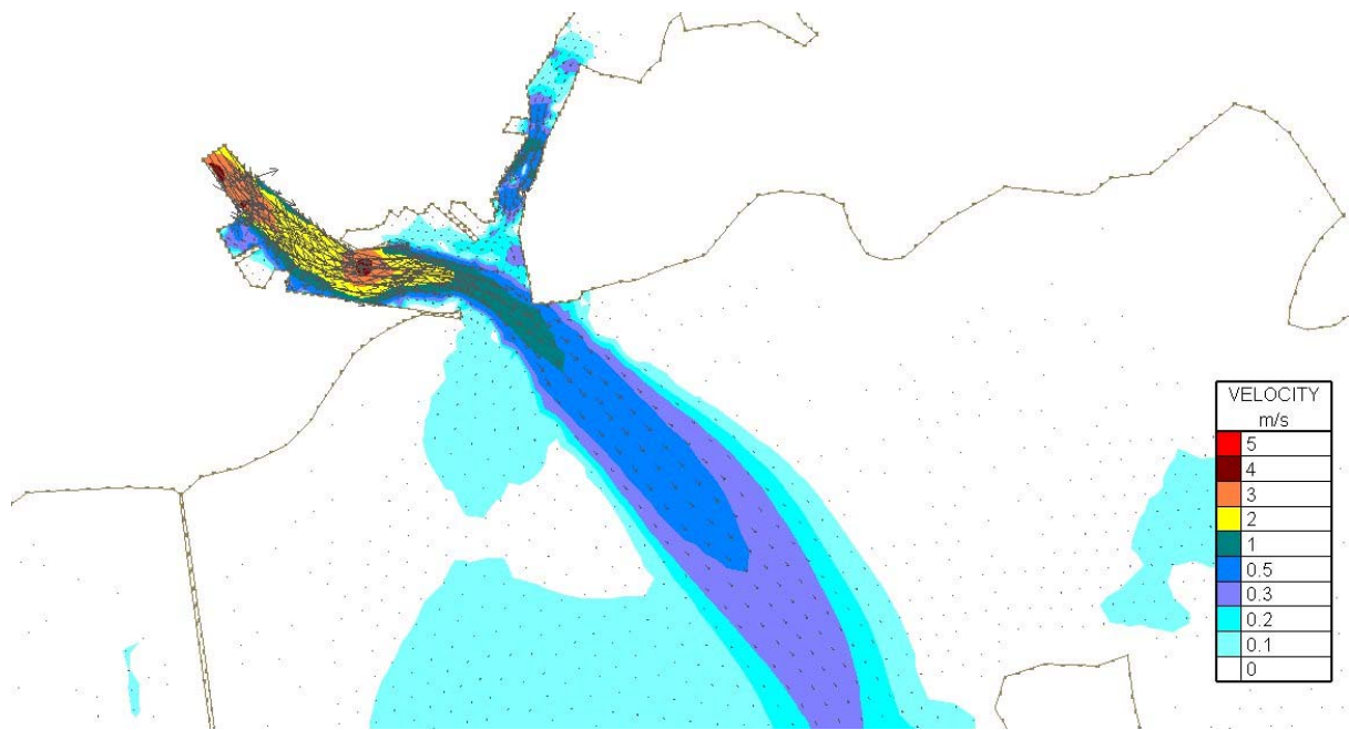
Figure Error! No text of specified style in document..179 Velocity Magnitudes at Low Water (6.2hrs after highwater Tide) for Flood Simulation 4– 100 year river flow and a tide of 4.146m (200 year tide) – Existing Case
