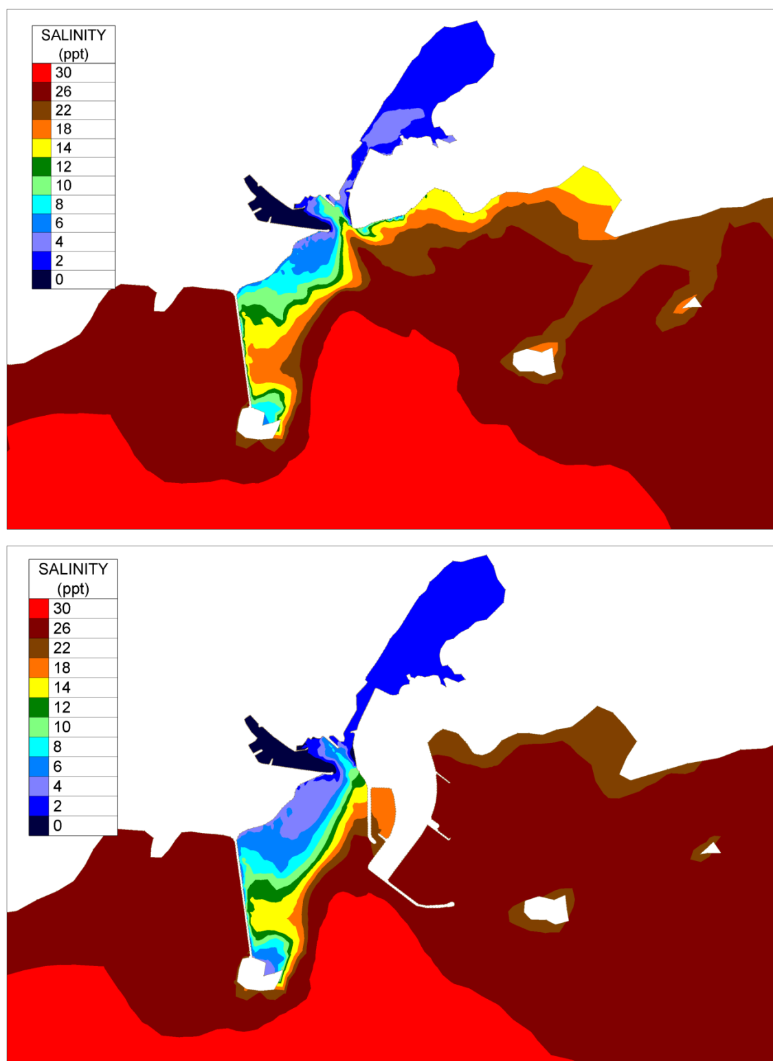
Figure Error! No text of specified style in document..86 Mean Salinity concentration in bottom layer for existing and proposed cases under 10-percentile Corrib Flow (200cumec)
