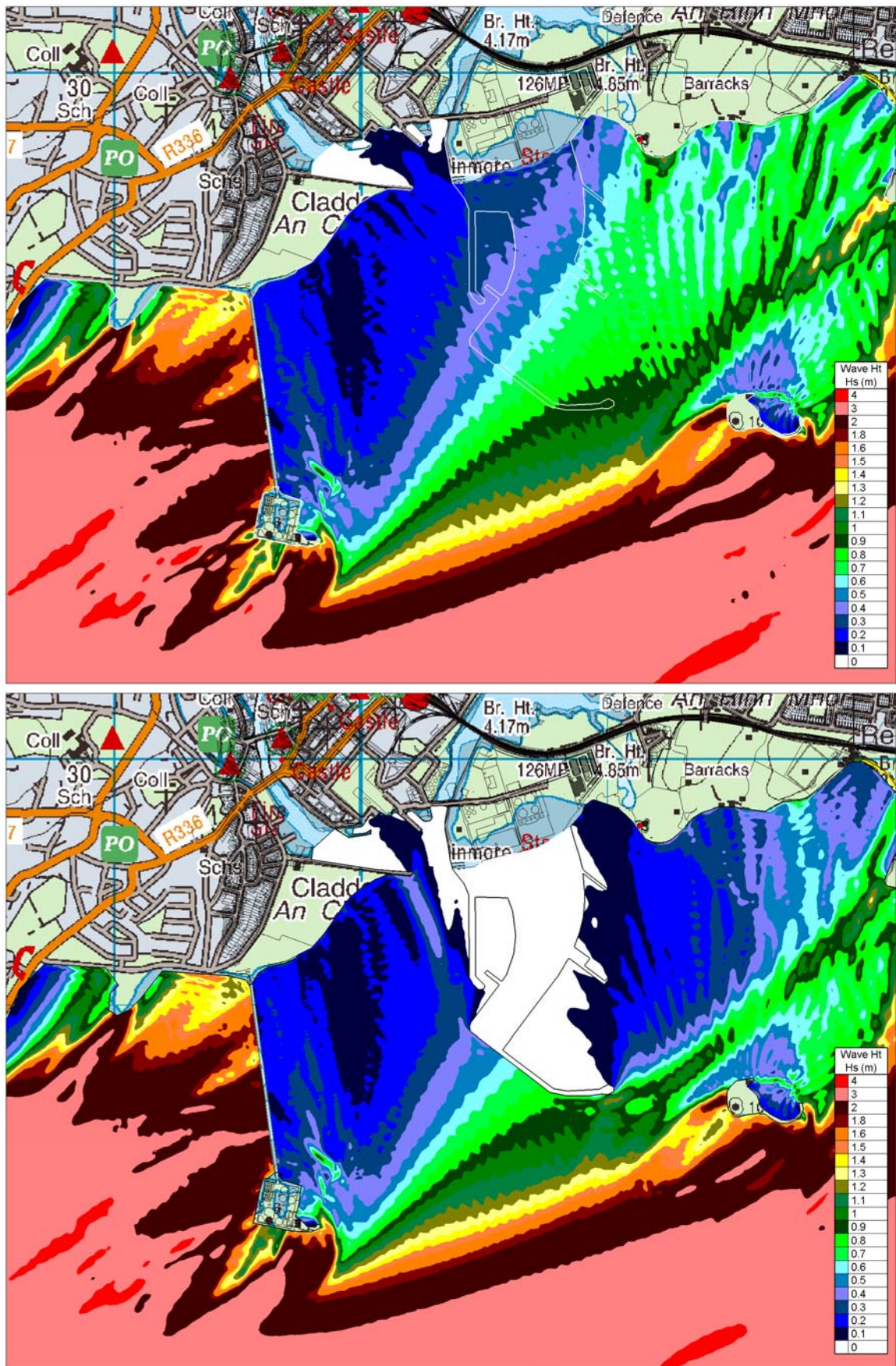
Figure Error! No text of specified style in document..133 ARTEMIS Significant Wave Heights for Atlantic Storm from the West-South-West for Existing and Proposed Case
