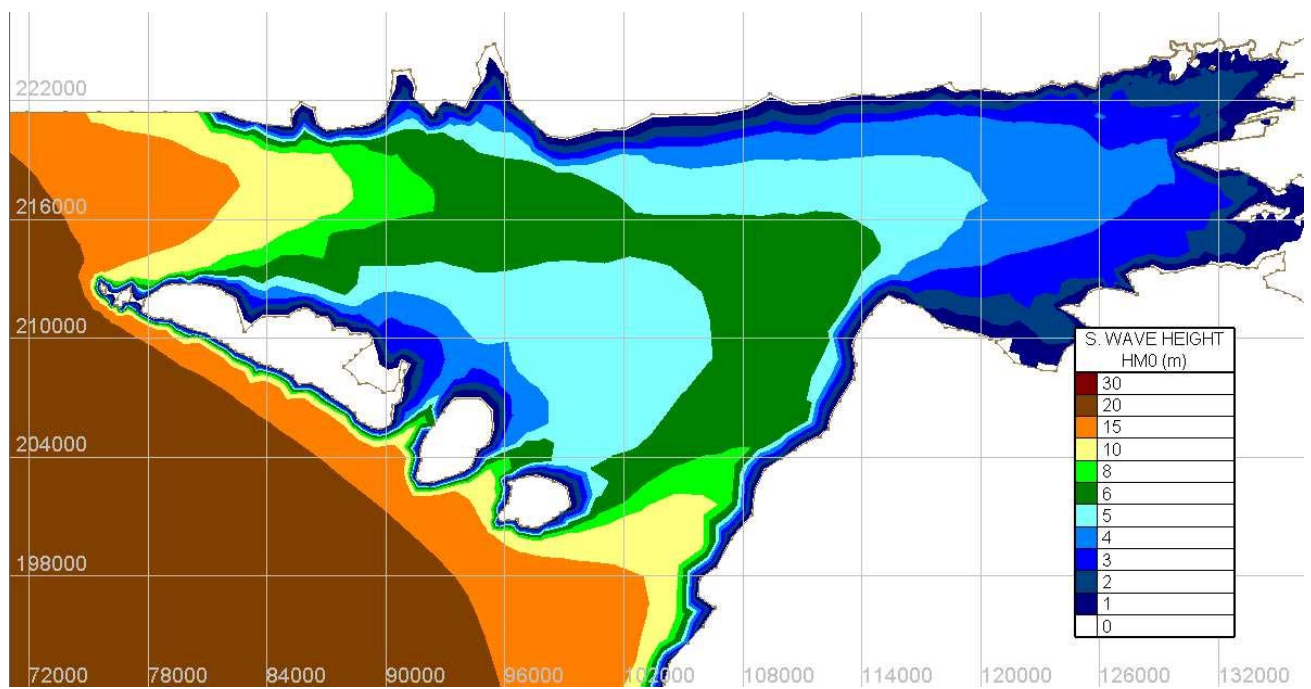
Figure Error! No text of specified style in document..132 Wave climate under 50year Westerly wind conditions
