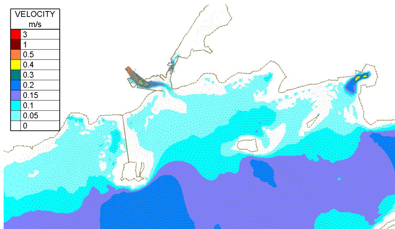
Figure Error! No text of specified style in document..7 - Depth averaged velocities Mid-flood Spring tide Median Corrib Flow
