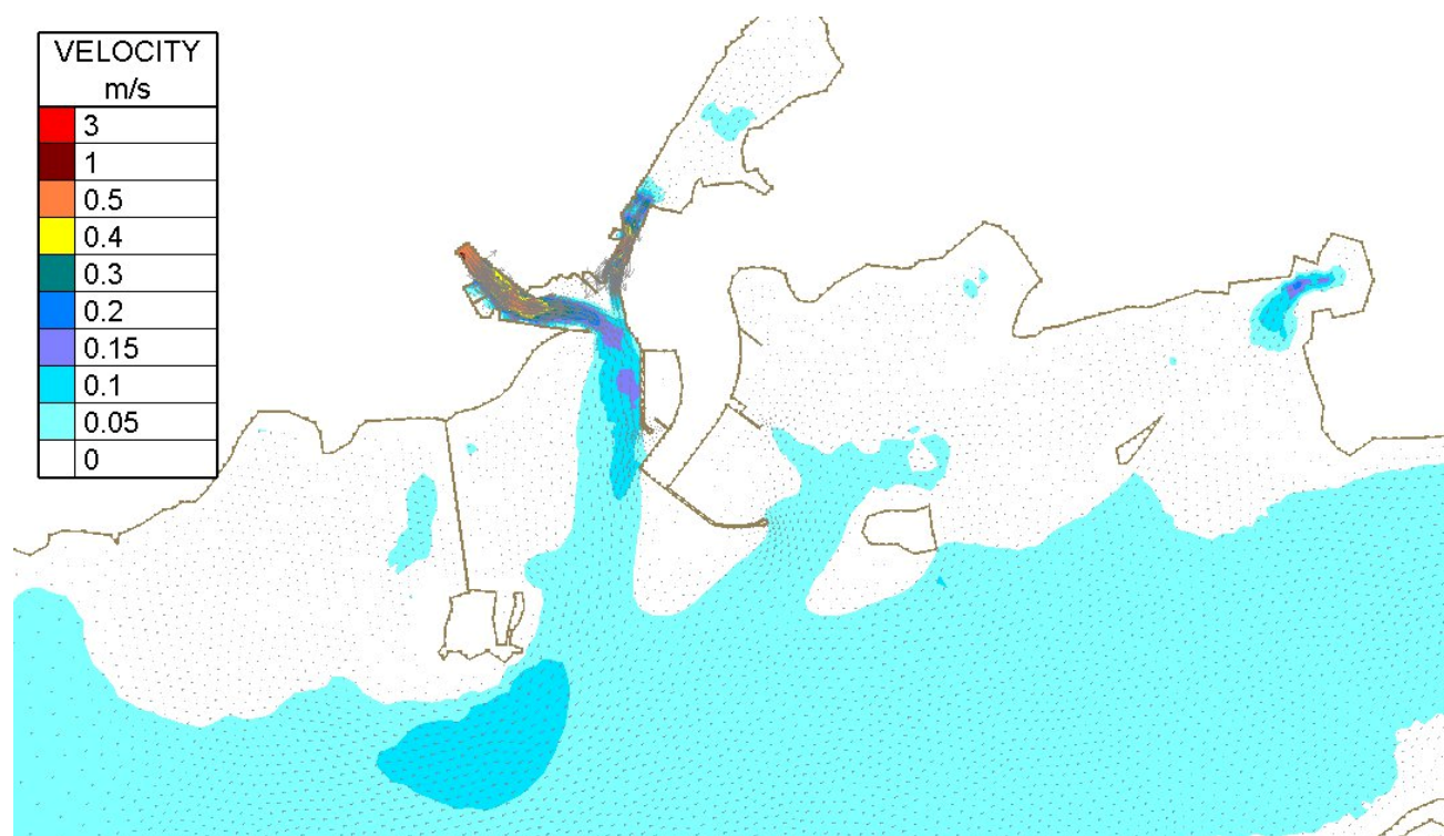
Figure Error! No text of specified style in document..10 - Depth averaged velocities Mid-ebb Neap tide Median Corrib Flow with new development
