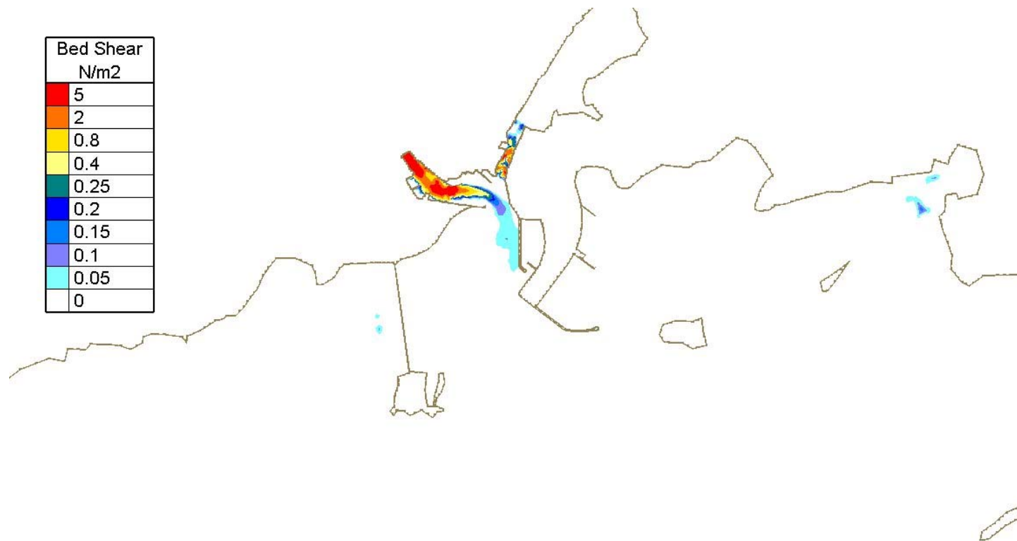
Figure Error! No text of specified style in document...28 - Computed bed shear at low water with new harbour extension development – Neap Tide and Median River Corrib Flow (82 m 3 /s)
