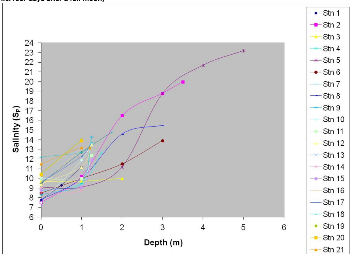
Figure Error! No text of specified style in document..72 Salinity profiles of Lough Atalia 16/04/2012 (carried out approximately three-quarters of an hour either side of high tide, occurring two days after the peak of a Neap tide)
