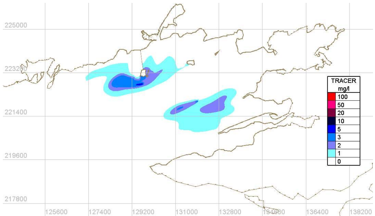
Figure Error! No text of specified style in document..92 Mid-ebb Existing Case - Spring tides
