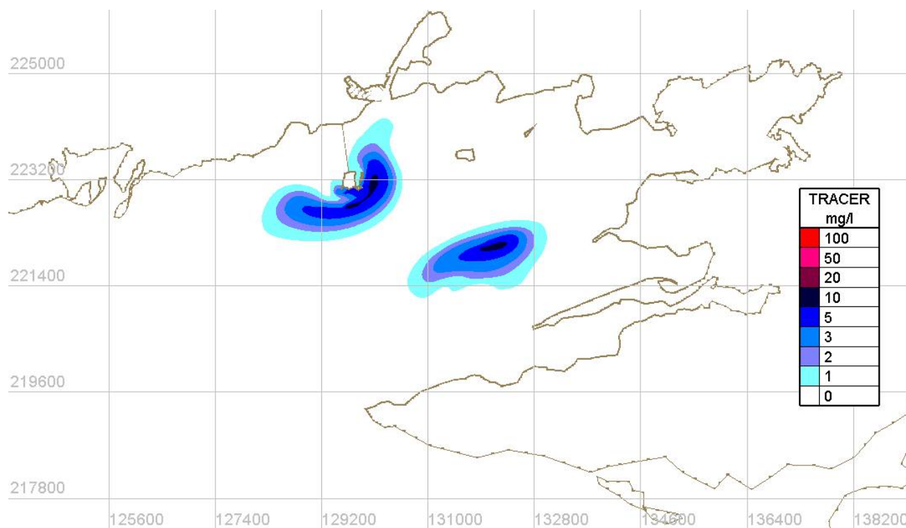
Figure Error! No text of specified style in document..104 Mid Flood - Existing Case - Neap tides
