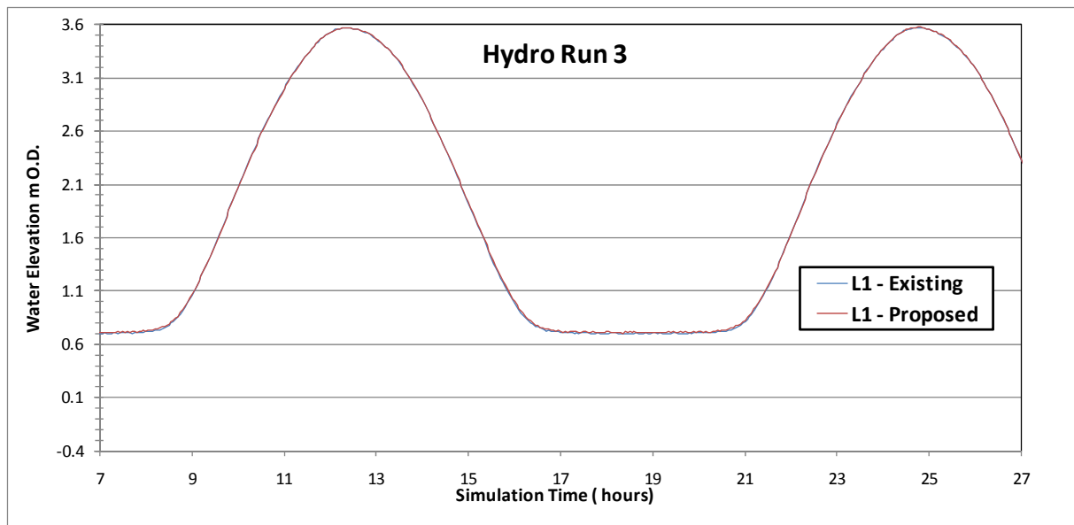
Figure Error! No text of specified style in document..198 Flood level comparison between existing and proposed for Hydrodynamic Simulation No. 3 at reference site 1 in Claddagh Basin adjacent to Spanish Arch
