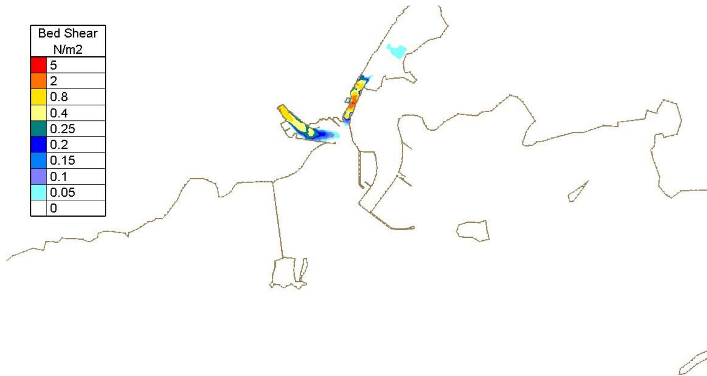
Figure Error! No text of specified style in document..32 - Computed bed shear at mid flood high tide with new harbour extension development – Neap Tide and Median River Corrib Flow (82 m 3 /s)
