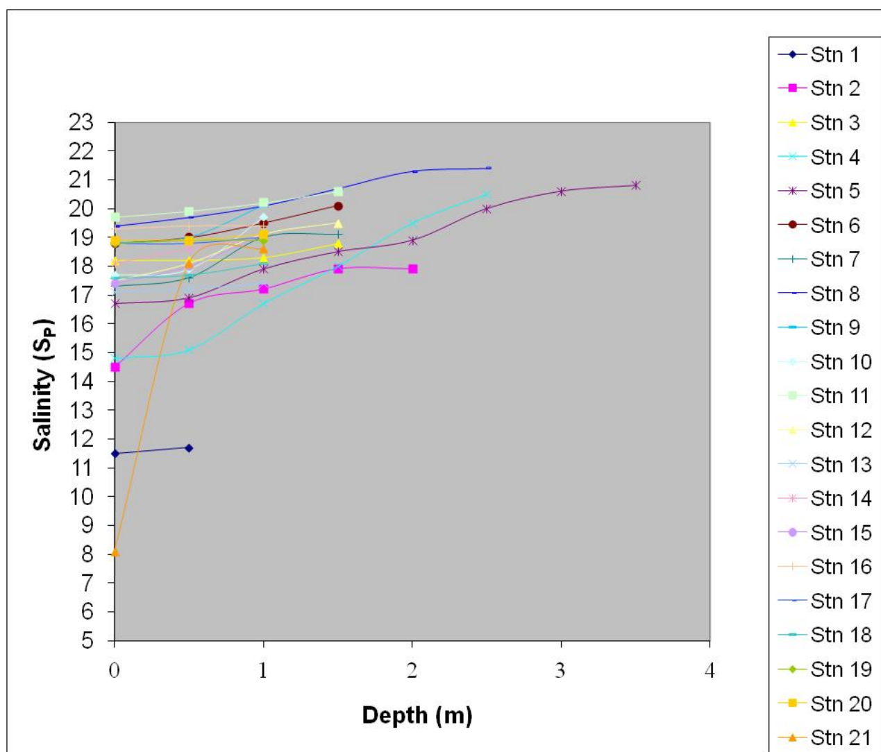
Figure Error! No text of specified style in document..70 Salinity profiles of Lough Atalia 04/04/2012 (carried out in the two hours preceding high tide, three days prior to Spring tide) Locations shown on Figure 8.4.62
