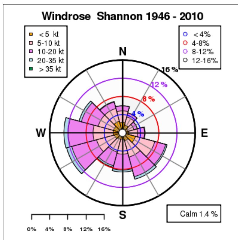
Figure Error! No text of specified style in document..124 Long-term Wind Roses for Belmullet (1957 to 2010), Valentia(1940 to 2010) and Shannon Airport (1946 to 2010)
