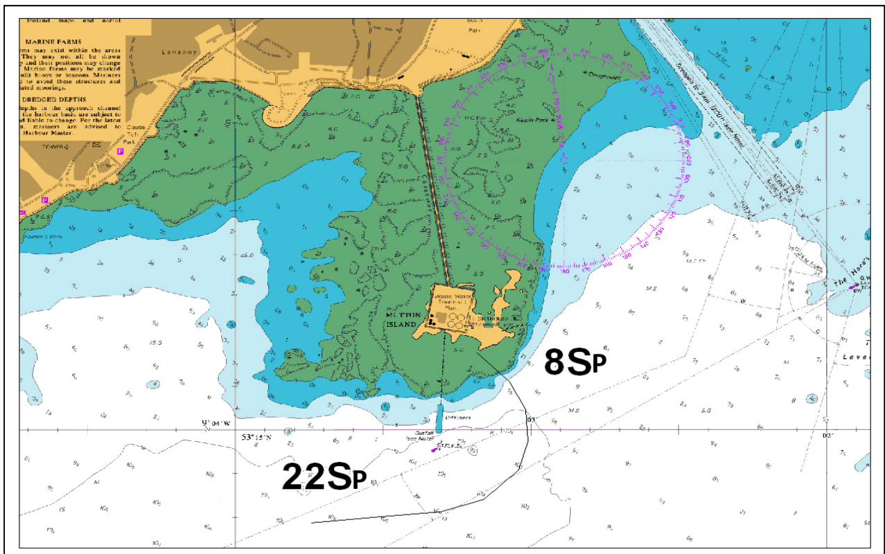
Figure Error! No text of specified style in document..67 The black line indicates a portion of a saltwater/freshwater front recorded at Mutton Island during 1988
