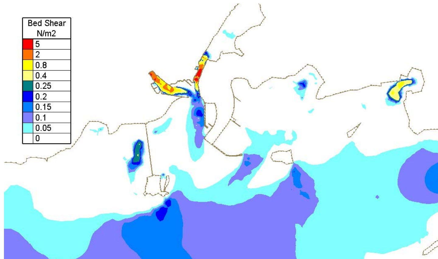
Figure Error! No text of specified style in document..18 - Computed bed shear at mid-ebb with new harbour extension development case – Spring Tide and Median River Corrib Flow (82 m³/s)
