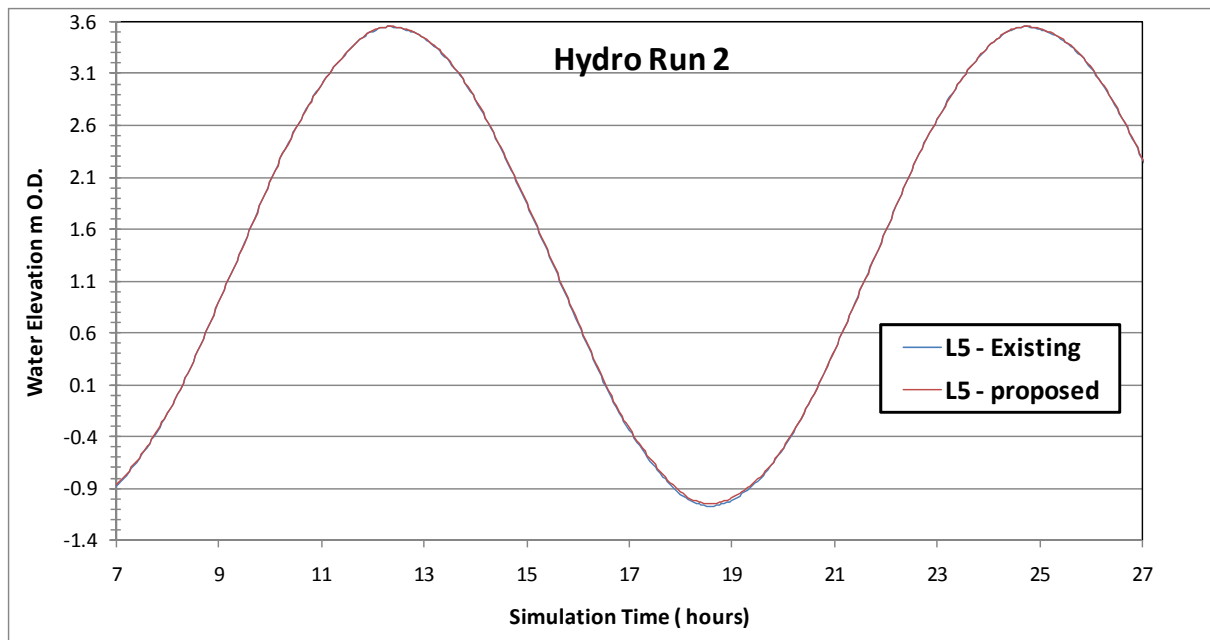
Figure Error! No text of specified style in document..196 Flood level comparison between existing and proposed for Hydrodynamic Simulation No. 2 at reference site 5 – new dredge channel at Marina Breakwater
