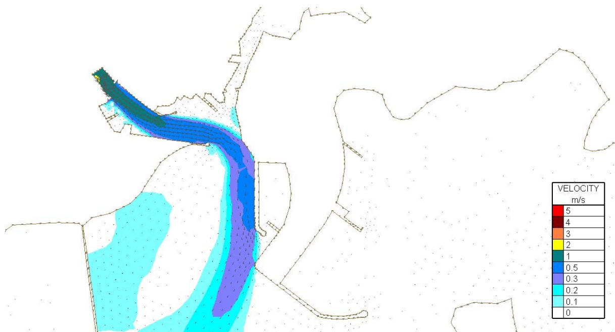
Figure Error! No text of specified style in document..182 Velocity Magnitudes at Mid Flood (3.1hrs before highwater Tide) for Flood Simulation 4 – 100 year river flow and a tide of 4.146m (200 year tide) – Proposed Harbour Extension Case
