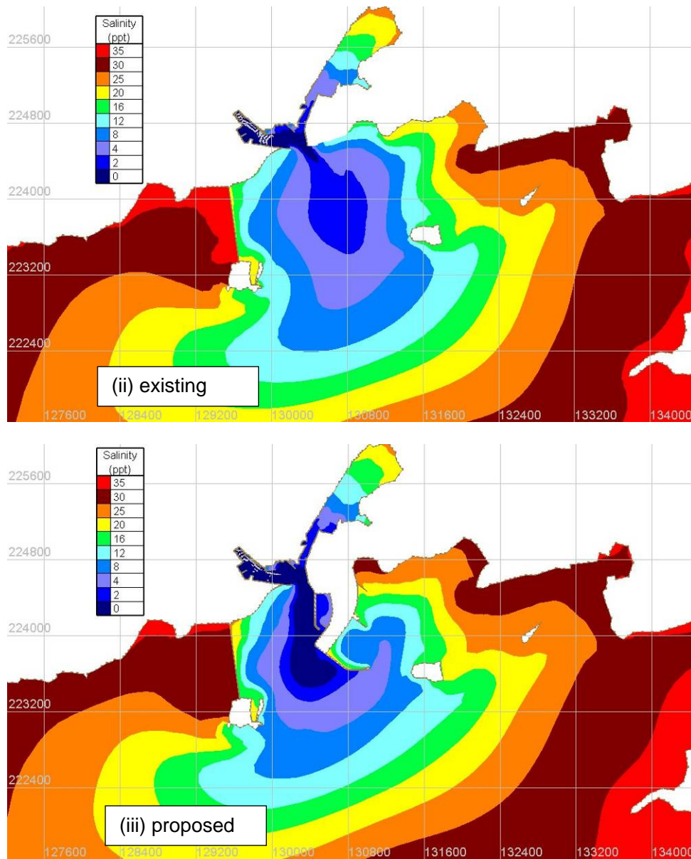
Figure Error! No text of specified style in document..123 Tidal Average Salinity –Neap Tides – median Corrib Flow
