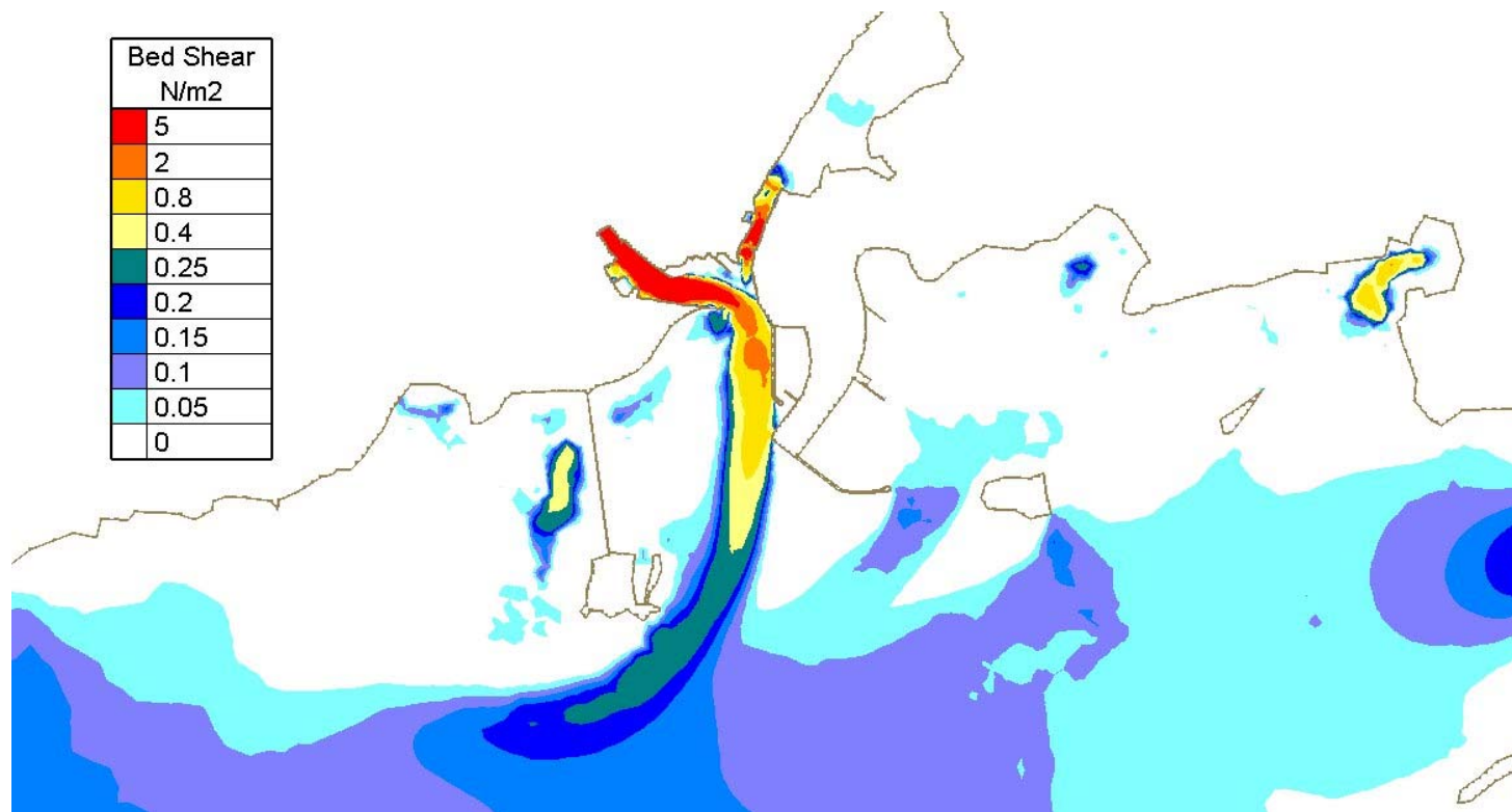
Figure Error! No text of specified style in document..34 - Computed bed shear at mid-ebb Spring Tide with 100 year Corrib Flood Flow with new harbour extension development
