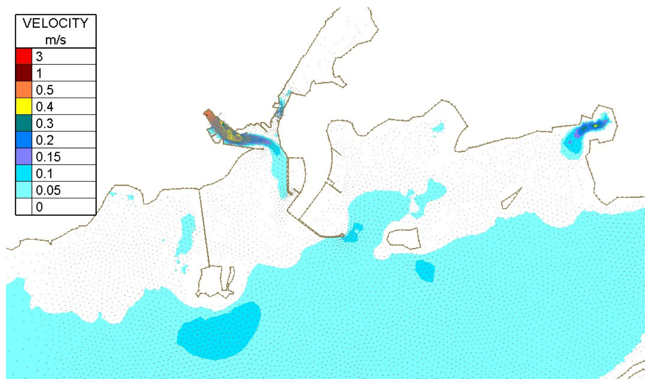
Figure Error! No text of specified style in document..12 - Depth averaged velocities Mid-Flood Neap tide Median Corrib Flow with new development
