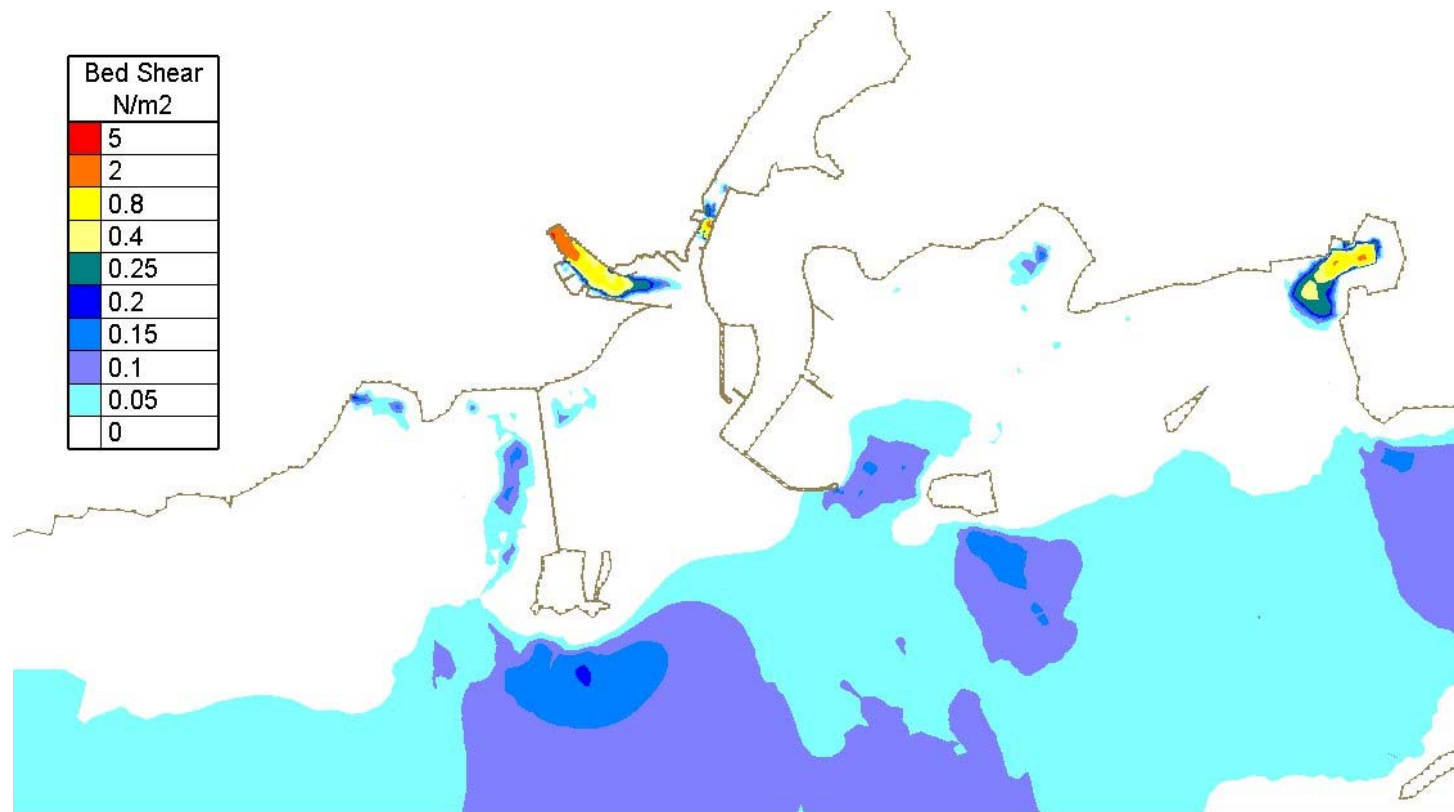
Figure Error! No text of specified style in document..22 - Computed bed shear at mid-flood with new harbour extension development – Spring Tide and Median River Corrib Flow (82 m 3 /s)
