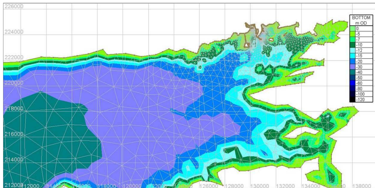
Figure Error! No text of specified style in document..128 View of Inner Galway Bay as represented in the TOMAWAC Model
