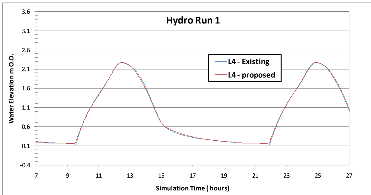
Figure Error! No text of specified style in document..189 Flood level comparison between existing and proposed for Hydrodynamic Simulation No. 1 at reference site 4 – entrance channel to Lough Atalia
