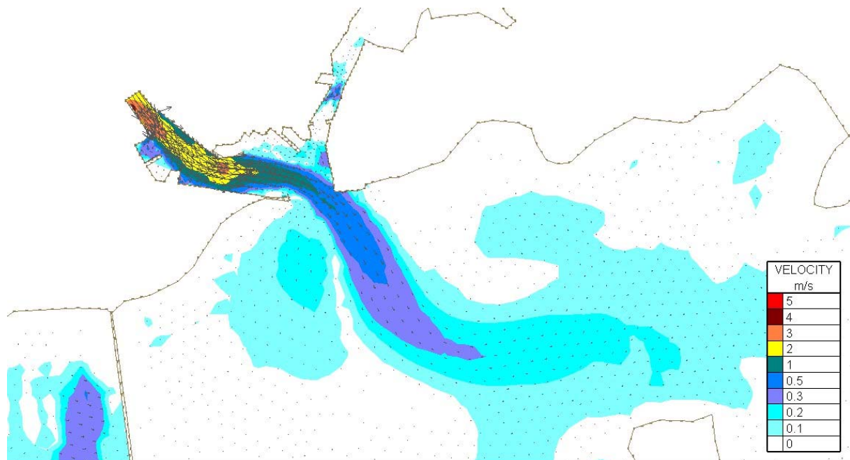
Figure Error! No text of specified style in document..157 Velocity Magnitudes at Mid Flood (3.1hrs before highwater Tide) for Flood Simulation 1 - 100 year river flow and mean spring tide – Existing Case
