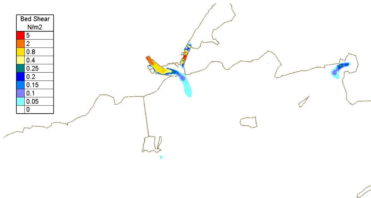
Figure Error! No text of specified style in document..25 - Computed bed shear at mid-ebb existing case without new harbour extension development – Neap Tide and Median River Corrib Flow (82 m 3 /s)
