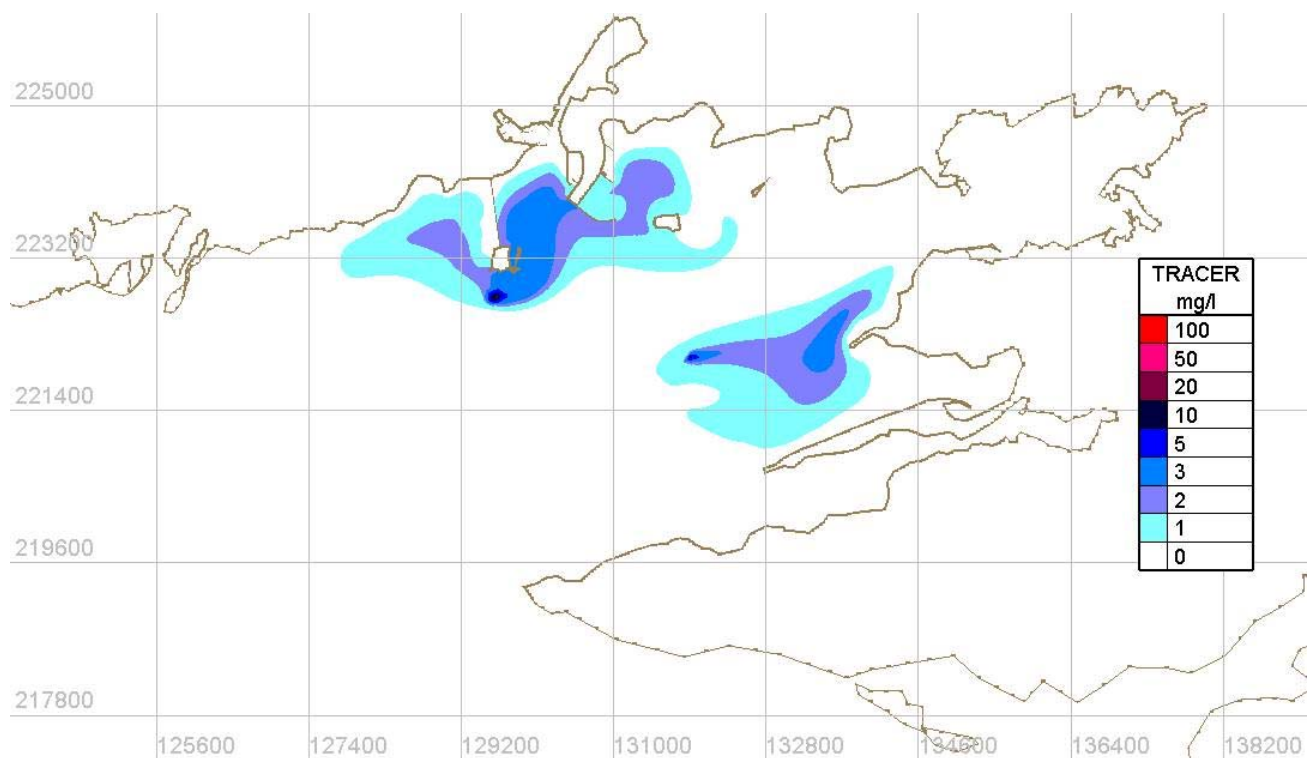
Figure Error! No text of specified style in document..99 High Water - Proposed Case - Spring tides
