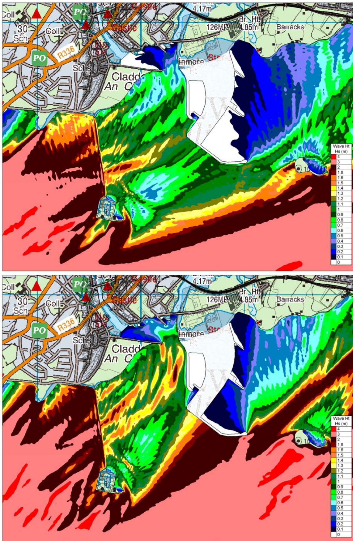
Figure Error! No text of specified style in document..143 West-South-West Design Wave at extreme highwater of 4.635 m O.D. Malin to examine the ability of Mutton Island Causeway to protect the Harbour and Marina area from West-South-West and south-west deepwater design waves
