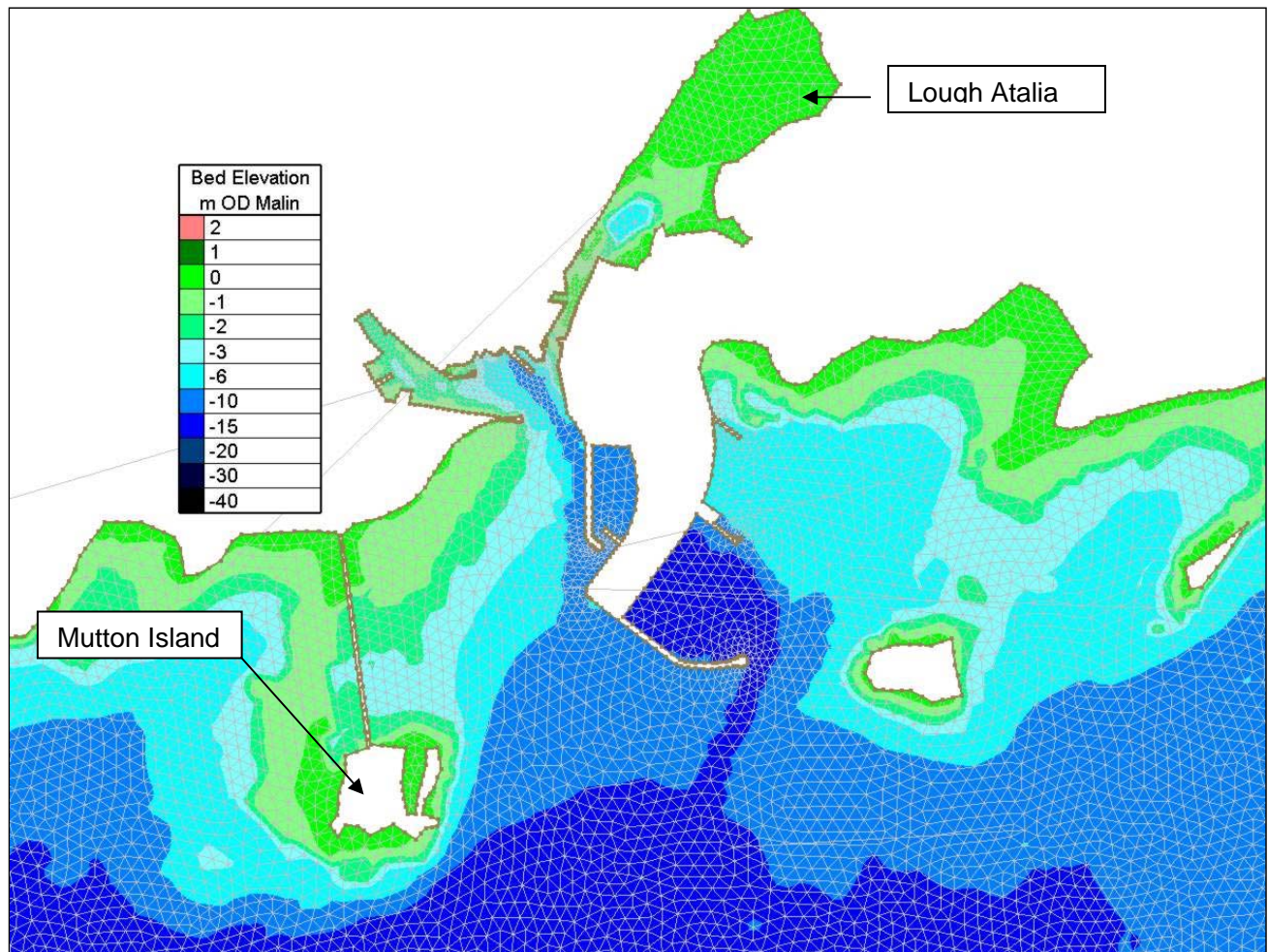
Figure Error! No text of specified style in document..4 - View of Hydrodynamic model mesh for proposed case in the vicinity of the proposed harbour extension
