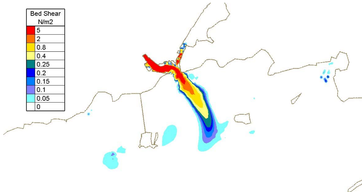
Figure Error! No text of specified style in document..35 - Computed bed shear at Low Water Spring Tide with 100 year Corrib Flood Flow for existing case
