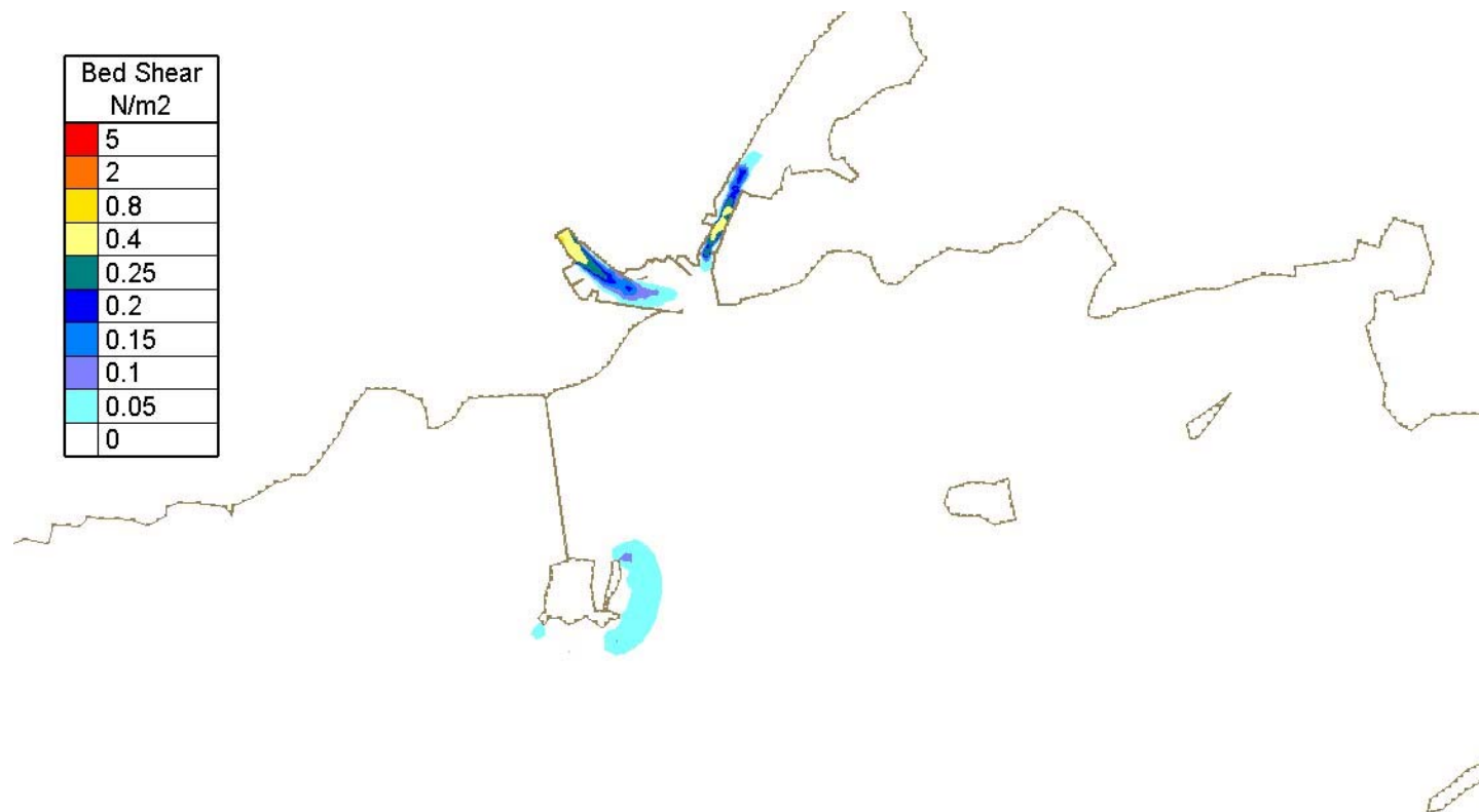
Figure Error! No text of specified style in document..23 - Computed bed shear at Highwater for existing case without development – Spring Tide and Median River Corrib Flow (82 m 3 /s)
