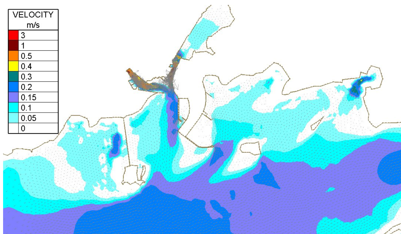
Figure Error! No text of specified style in document..6 - Depth averaged velocities Mid-ebb Spring tide Median Corrib Flow with new development
