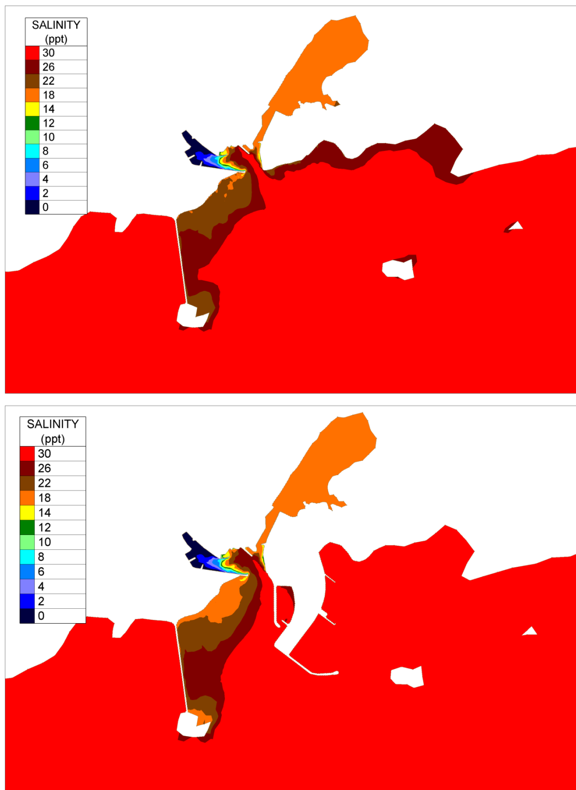
Figure Error! No text of specified style in document..80 Mean Salinity concentration in bottom layer for existing and proposed cases under 90-percentile Corrib Flow (28.5cumecc)
