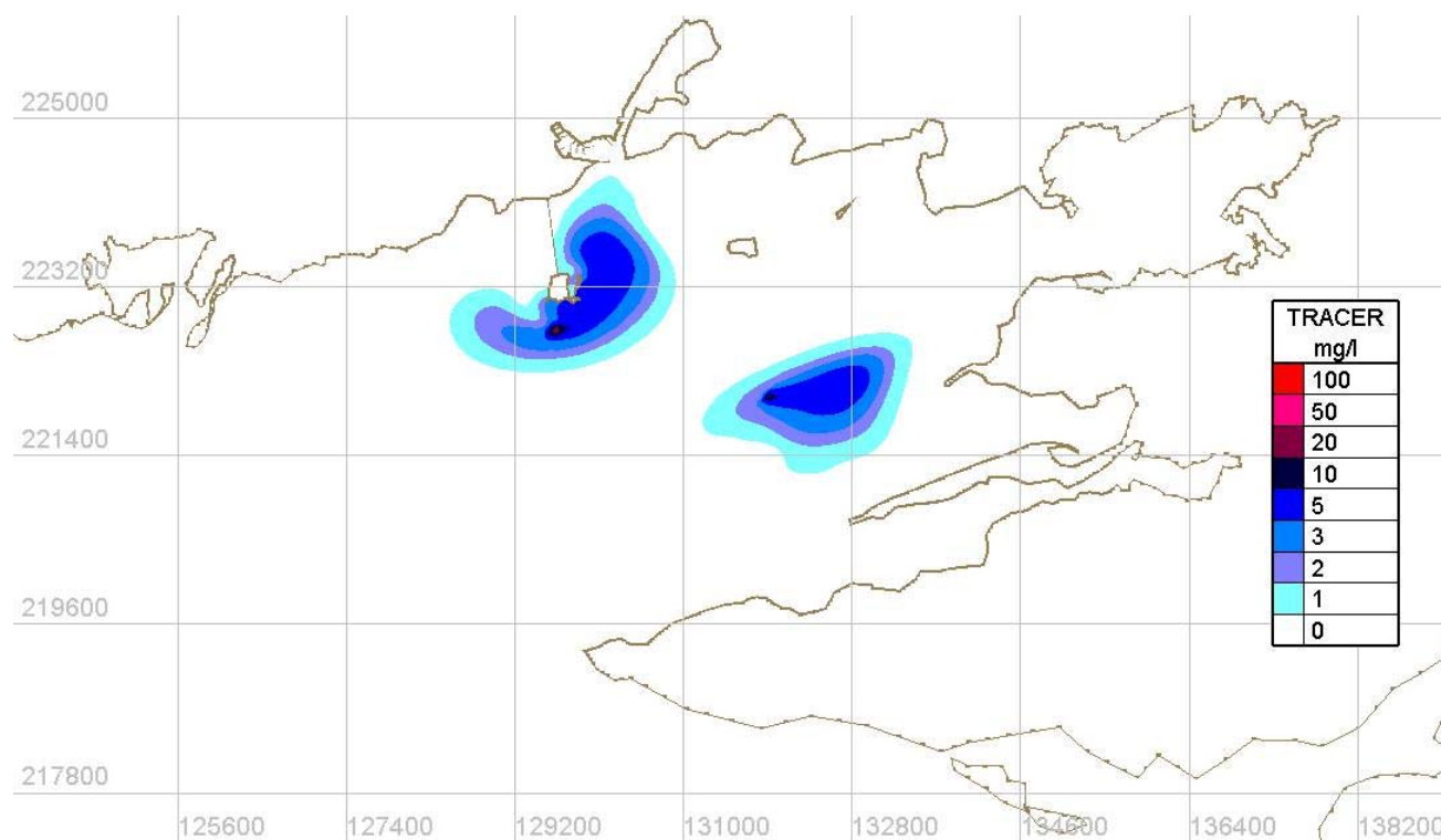
Figure Error! No text of specified style in document..106 High Water - Existing Case - Neap tides
