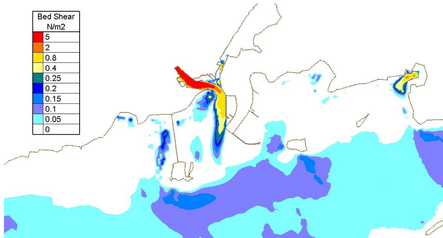
Figure Error! No text of specified style in document..38 - Computed bed shear at mid-flood Spring Tide with 100 year Corrib Flood Flow with new harbour extension development
