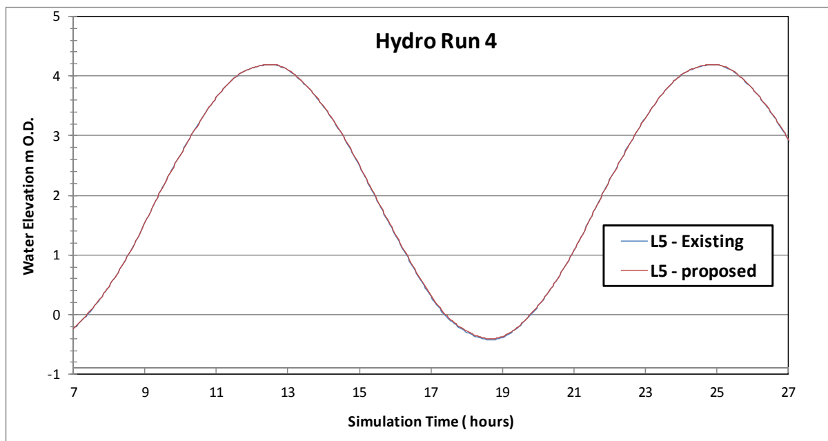
Figure Error! No text of specified style in document..208 Flood level comparison between existing and proposed for Hydrodynamic Simulation No. 4at reference site 5 – new dredge channel at Marina Breakwater
