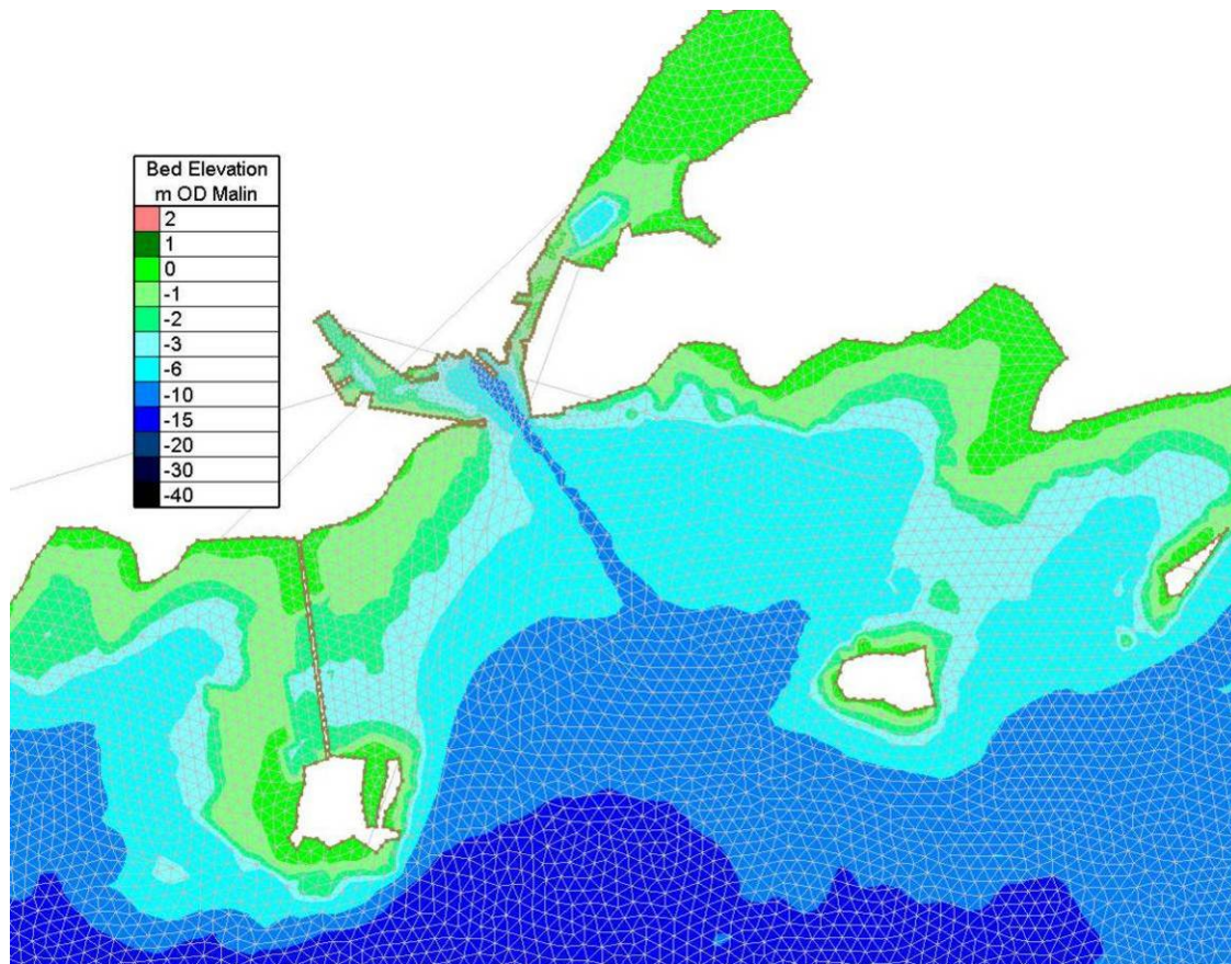
Figure Error! No text of specified style in document..151 Close-up view of model refinement in the vicinity of the proposed harbour development
