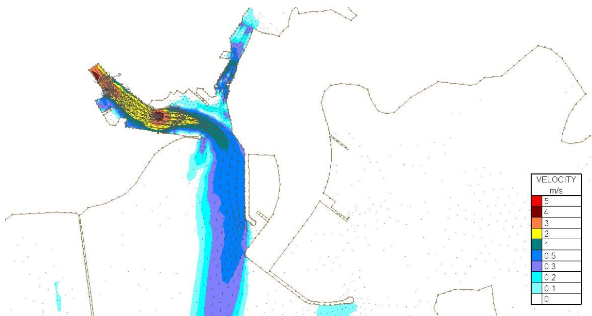
Figure Error! No text of specified style in document..180 Velocity Magnitudes at Low Water (6.2hrs after highwater Tide) for Flood Simulation 4– 100 year river flow and a tide of 4.146m (200 year tide) – Proposed Harbour Extension Case
