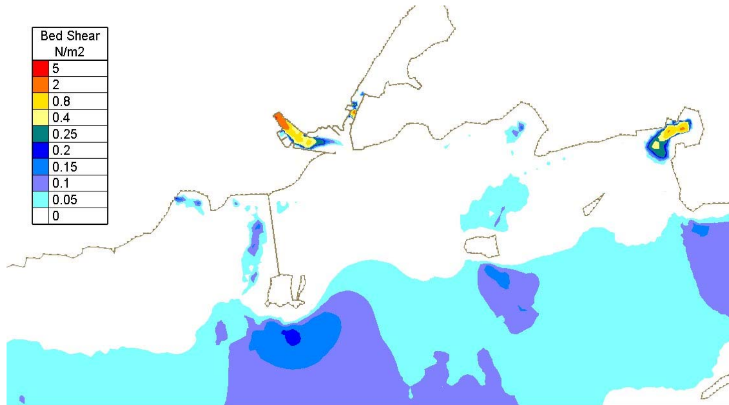
Figure Error! No text of specified style in document..21 - Computed bed shear at mid-flood for existing case without development – Spring Tide and Median River Corrib Flow (82 m 3 /s)
