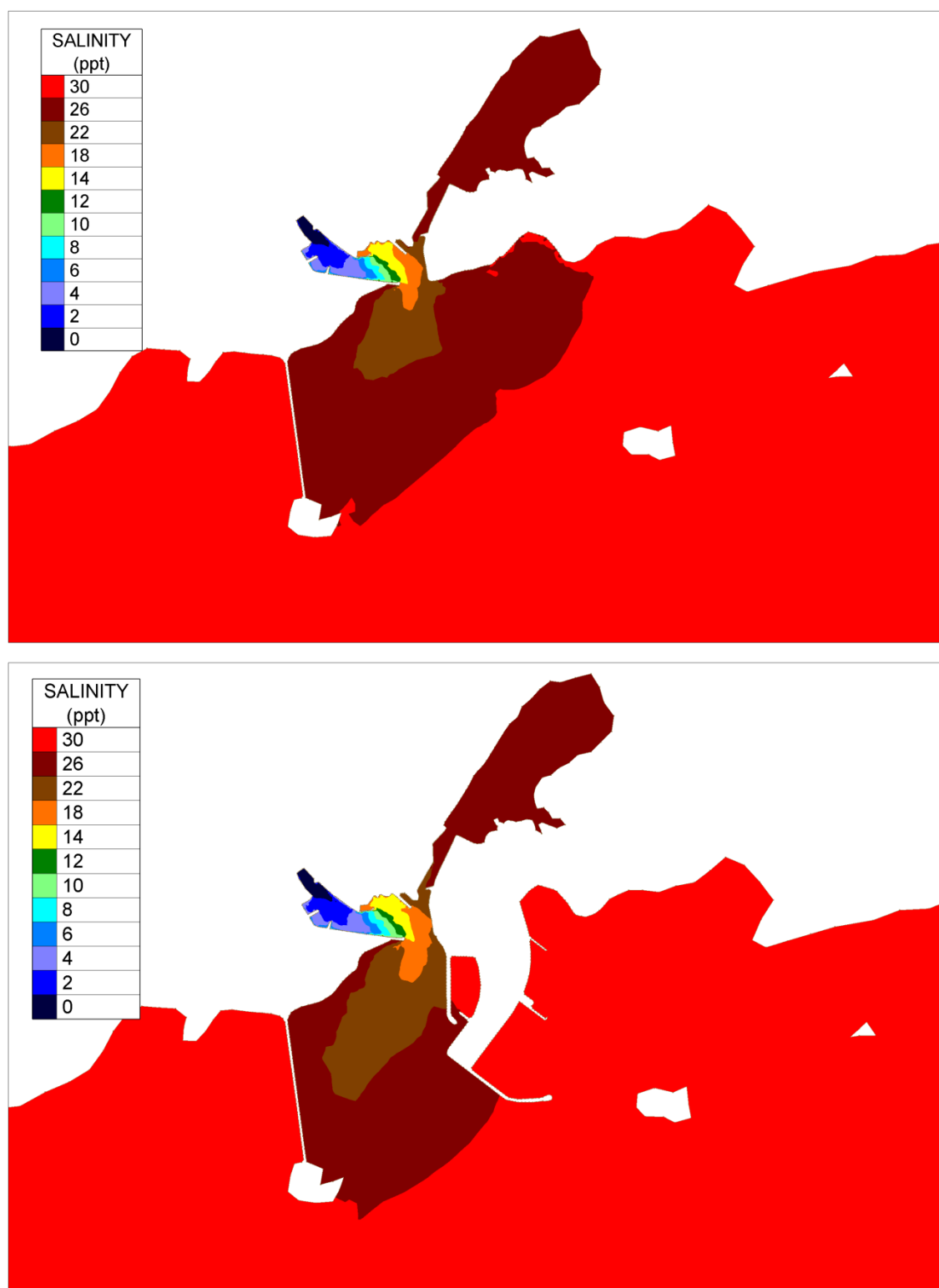
Figure Error! No text of specified style in document..79 Mean Salinity concentration in surface layer for existing and proposed cases under 99-percentile Corrib Low Flow (9.1 cumec)
