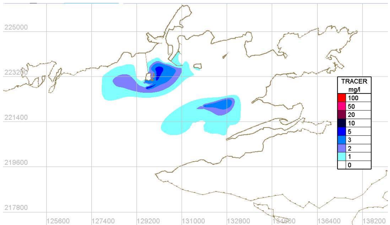
Figure Error! No text of specified style in document..97 Mid Flood - Proposed Case - Spring tides
