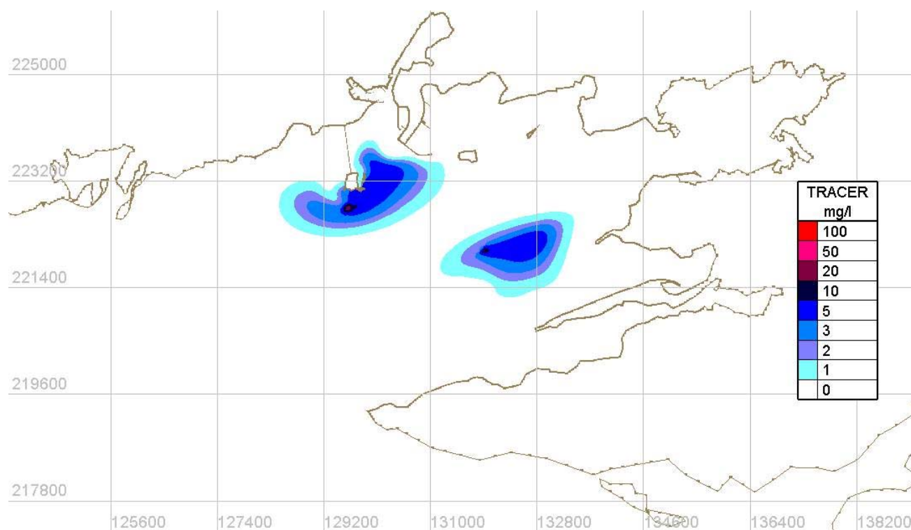
Figure Error! No text of specified style in document..107 High Water - Proposed Case - Neap tides
