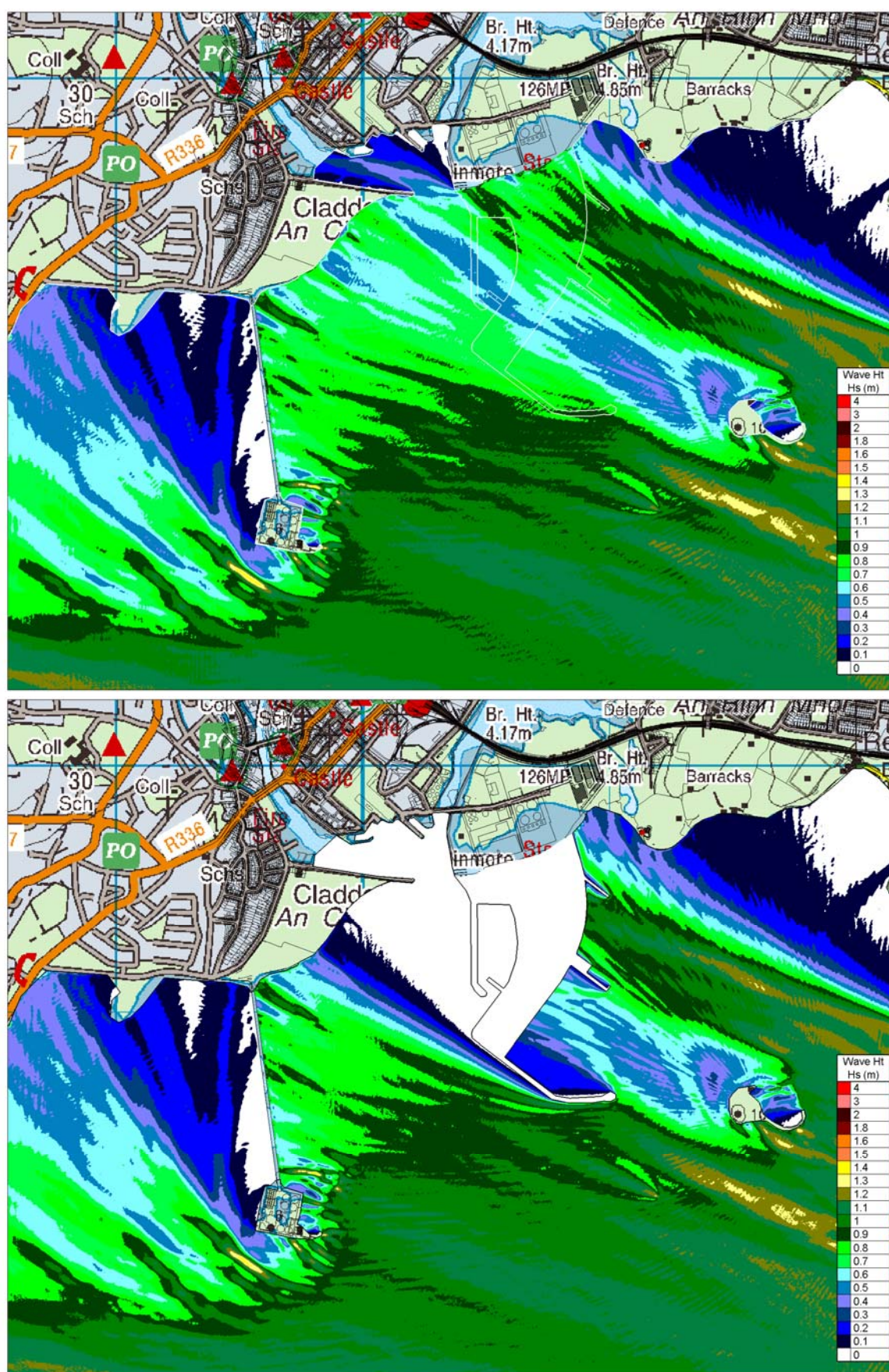
Figure Error! No text of specified style in document..139 ARTEMIS Significant Wave Heights for local Design Storm Waves from the East-South-East for Existing and Proposed Case
