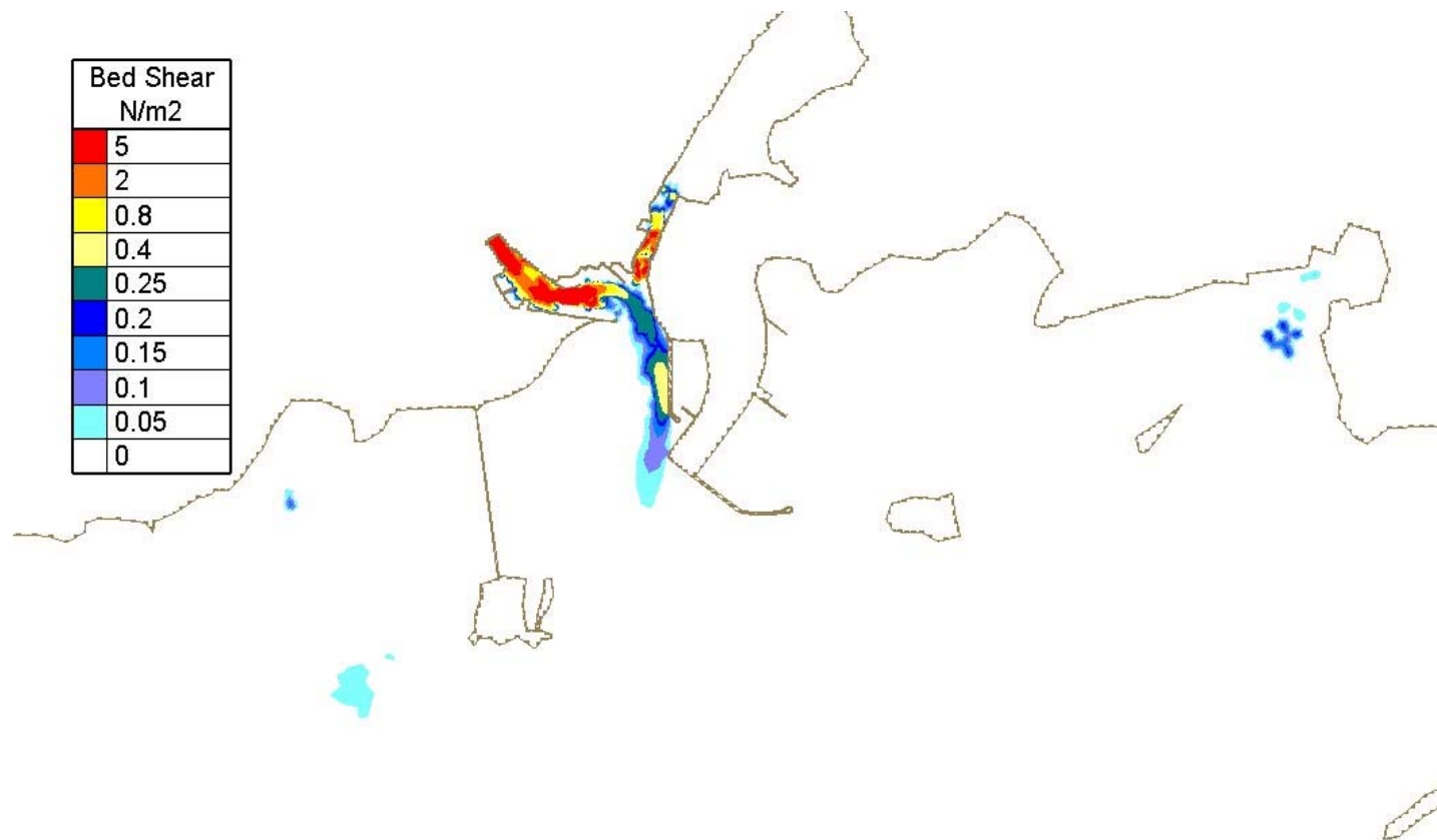
Figure Error! No text of specified style in document..20 - Computed bed shear at low water with new harbour extension development case – Spring Tide and Median River Corrib Flow (82 m 3 /s)
