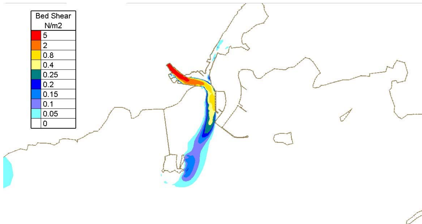
Figure Error! No text of specified style in document..40 - Computed bed shear at High Water Spring Tide with 100 year Corrib Flood Flow with new harbour extension development
