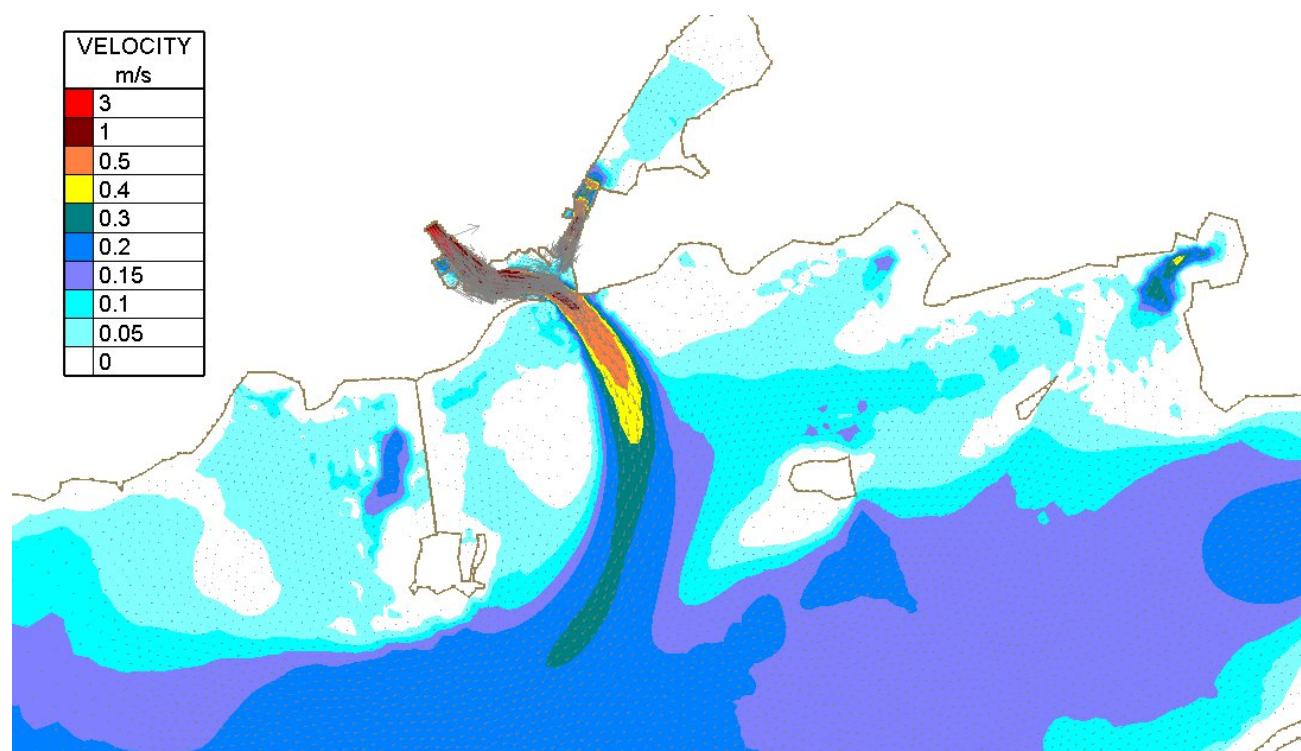
Figure Error! No text of specified style in document..13 - Depth averaged velocities Mid-ebb Spring Tide and 100 year Corrib Flow
