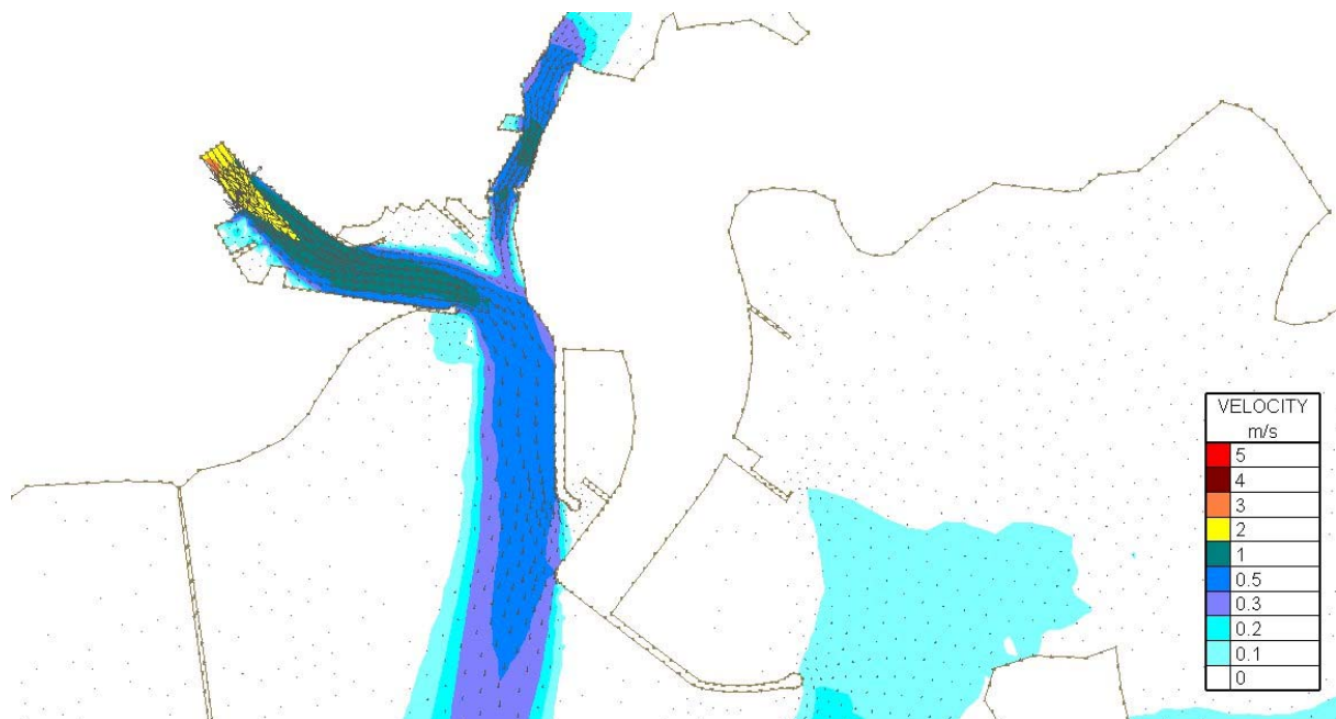
Figure Error! No text of specified style in document..178 Velocity Magnitudes at Mid-ebb (3.1hrs after highwater ) for Flood Simulation 4– 100 year river flow and a tide of 4.146m (200 year tide) – Proposed Harbour Extension Case
