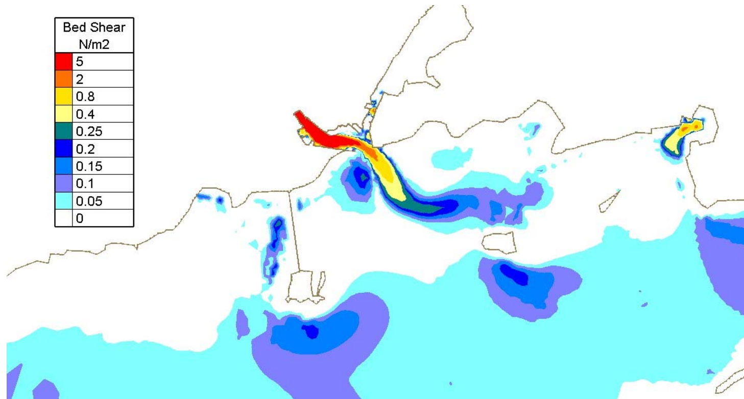
Figure Error! No text of specified style in document..37 - Computed bed shear at mid-flood Spring Tide with 100 year Corrib Flood Flow for existing case
