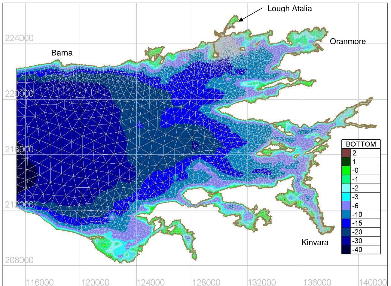
Figure Error! No text of specified style in document..2 - Hydrodynamic model finite element mesh and bathymetry for existing case. (Bottom refers to bed elevations mOD Malin)
