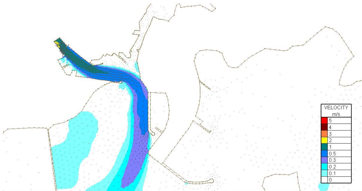
Figure Error! No text of specified style in document..176 Velocity Magnitudes at highwater for Flood Simulation 3 – river plus 20% climate change and a 3.49m tide – Proposed Harbour Extension Case
