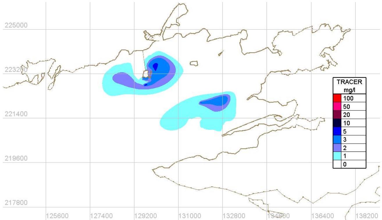
Figure Error! No text of specified style in document..96 Mid Flood - Existing Case - Spring tides
