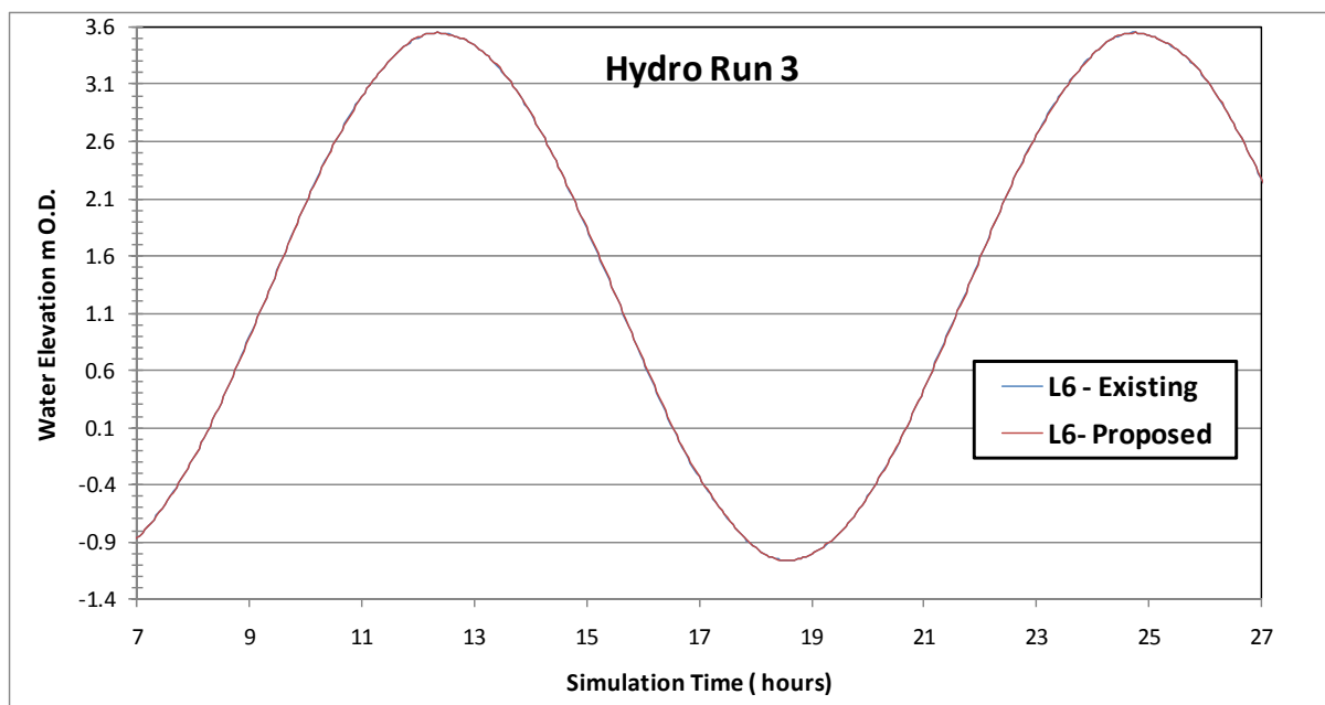
Figure Error! No text of specified style in document..203 Flood level comparison between existing and proposed for Hydrodynamic Simulation No. 3 at reference site 6 – new dredge channel south of Marina entrance
