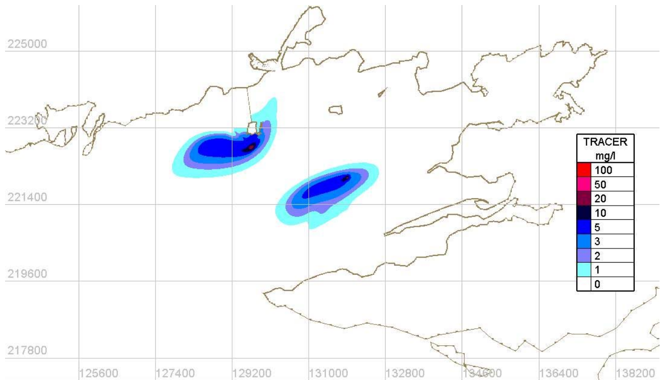
Figure Error! No text of specified style in document..102 Low water - Existing Case - Neap tides
