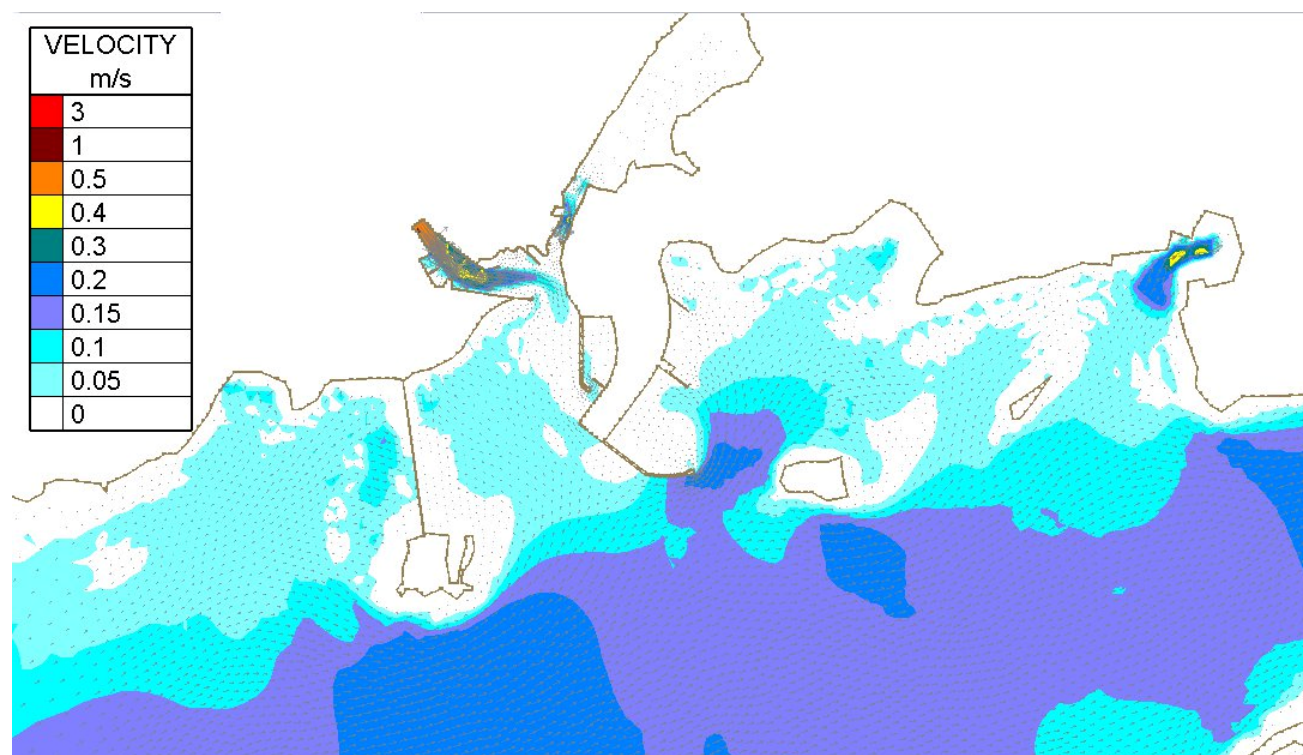
Figure Error! No text of specified style in document..8 - Depth averaged velocities Mid-Flood Spring tide Median Corrib Flow with new development
