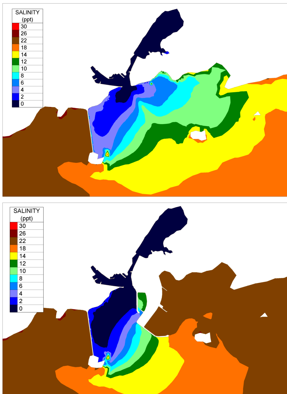
Figure Error! No text of specified style in document..91 Mean Salinity concentration in surface layer for existing and proposed cases under 1-percentile Corrib Flood Flow (272cumec)
