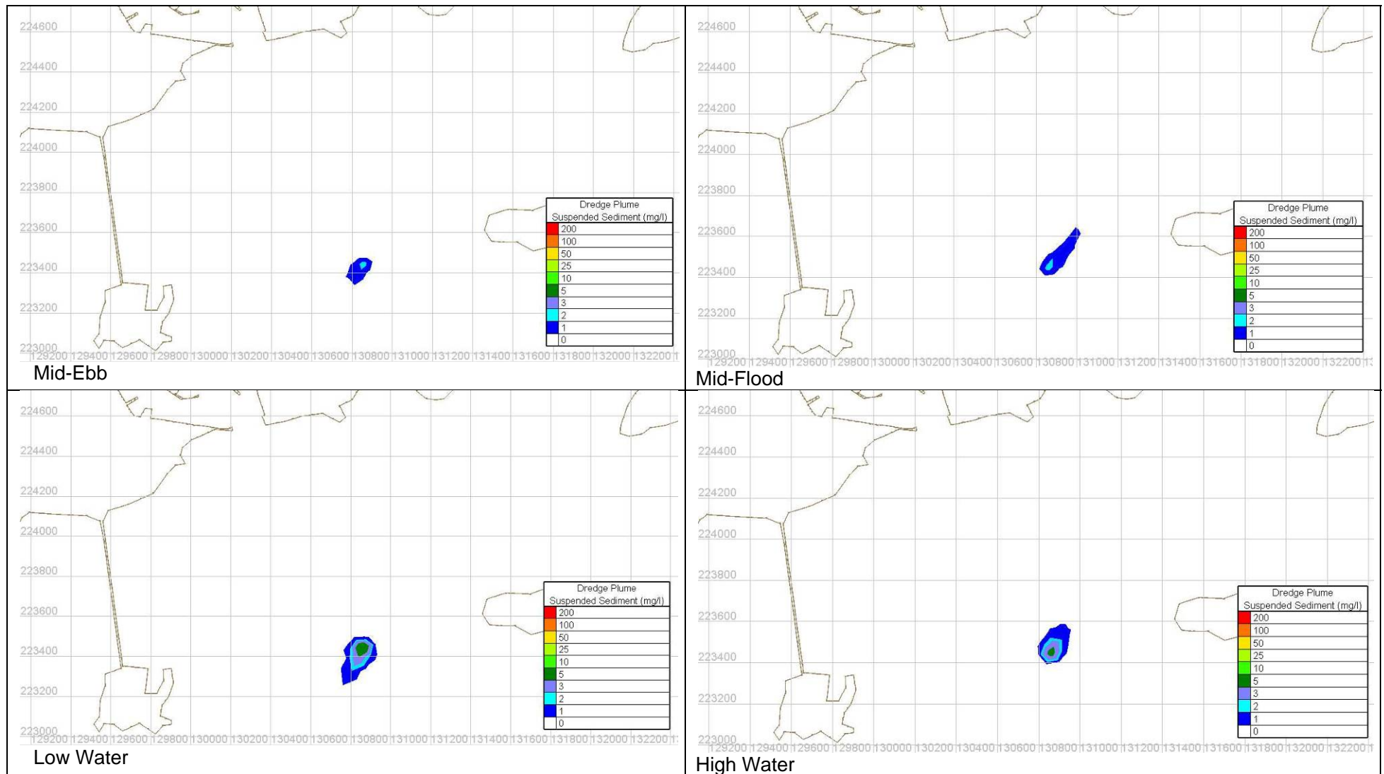
Figure Error! No text of specified style in document..49 Coarse silt suspended sediment plume simulation at dredge location 4 – Spring tide and Corrib Summer low flow
