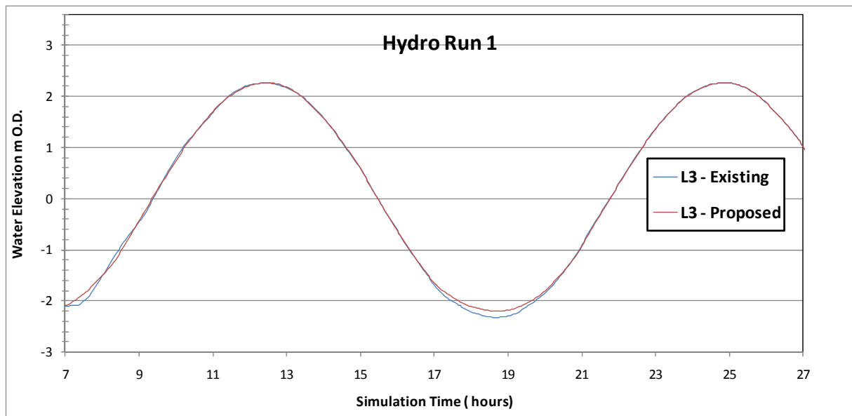
Figure Error! No text of specified style in document..188 Flood level comparison between existing and proposed for Hydrodynamic Simulation No. 1 at reference site 3 in estuary inside Nimmo's Pier
