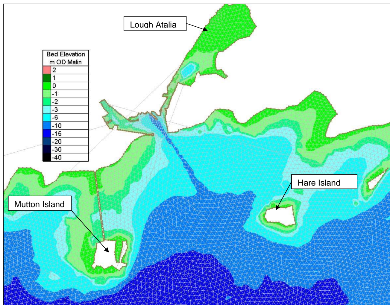
Figure Error! No text of specified style in document..3 - Close-up view of Hydrodynamic model refinement in the vicinity of the proposed harbour extension development
