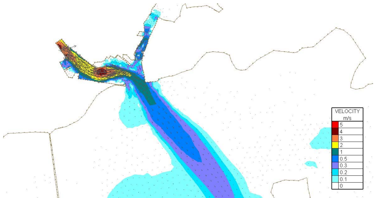
Figure Error! No text of specified style in document..171 Velocity Magnitudes at Low Water (6.2hrs after highwater Tide) for Flood Simulation 3- river plus 20% climate change and a 3.49m tide – Existing Case
