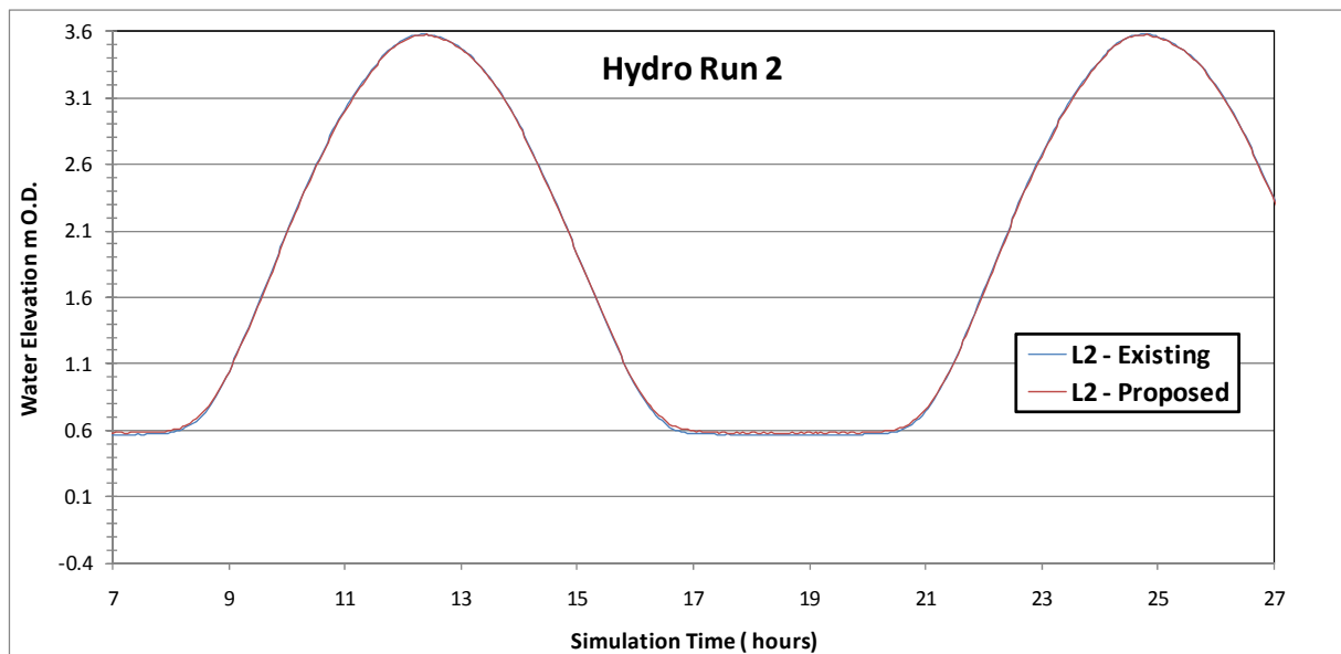
Figure Error! No text of specified style in document..193 Flood level comparison between existing and proposed for Hydrodynamic Simulation No. 2 at reference site 2 in Claddagh Basin
