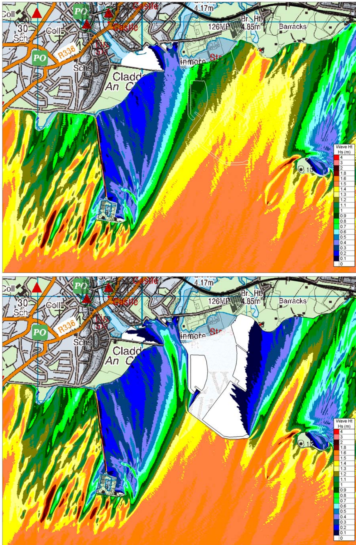
Figure Error! No text of specified style in document..135 ARTEMIS Significant Wave Heights for local Design Storm Waves from the South-South-West for Existing and Proposed Case
