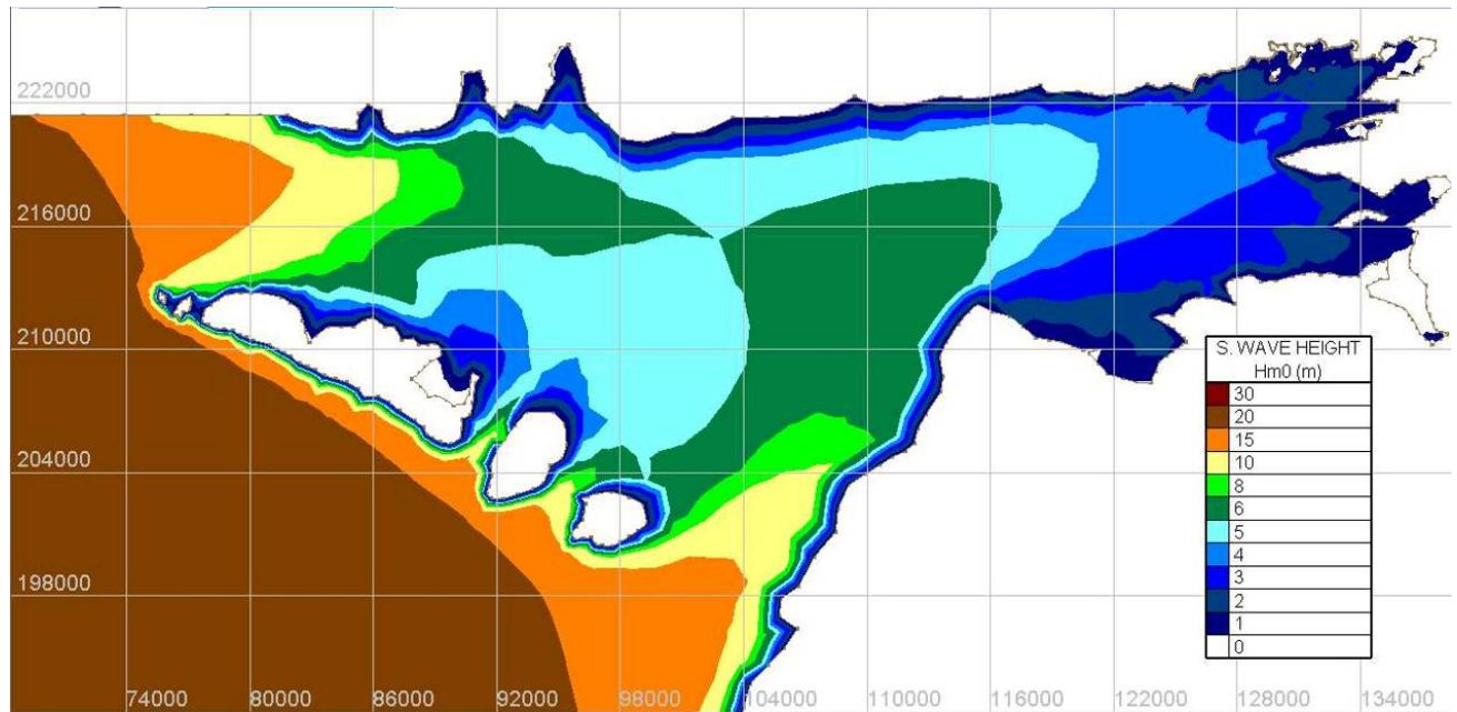
Figure Error! No text of specified style in document..131 Wave climate under 50year west southwest wind conditions
