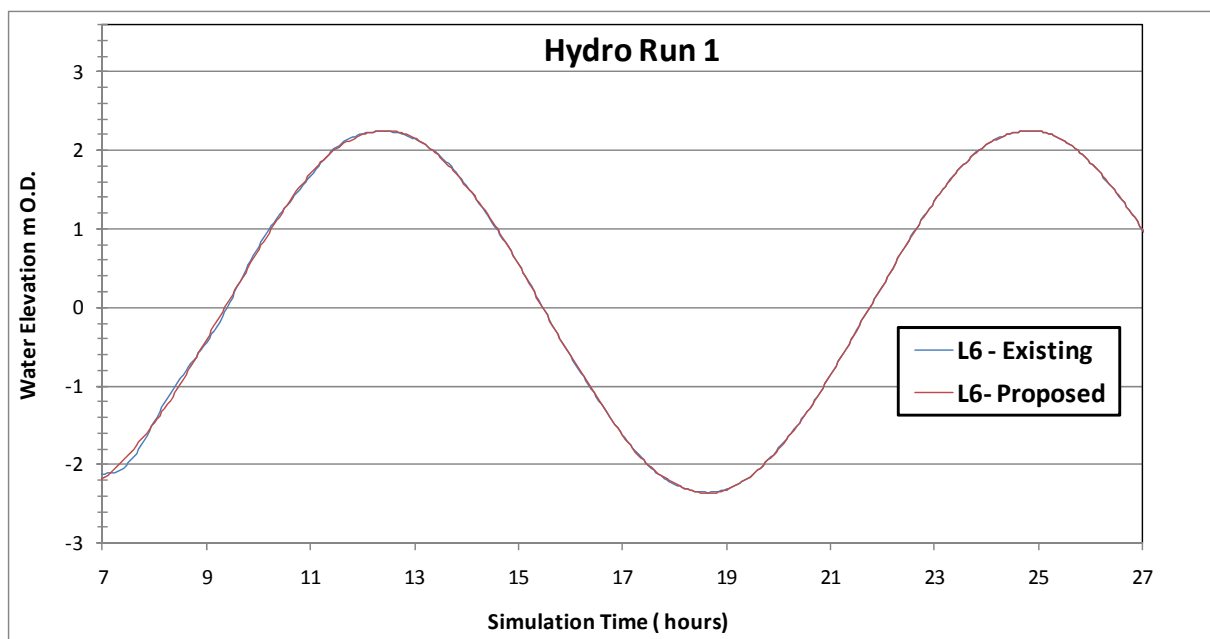
Figure Error! No text of specified style in document..191 Flood level comparison between existing and proposed for Hydrodynamic Simulation No. 1 at reference site 6 – new dredge channel south of Marina entrance
