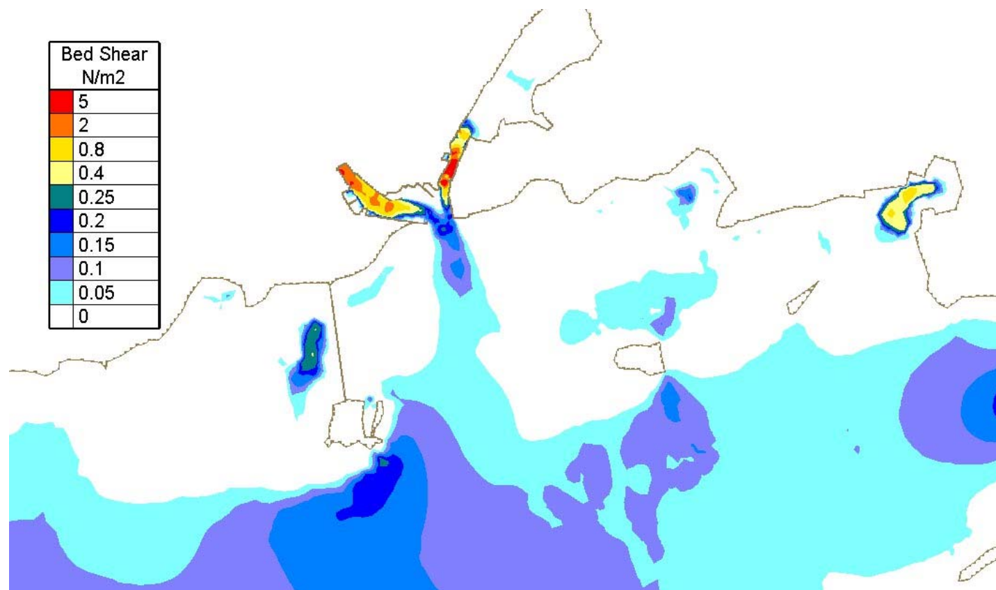
Figure Error! No text of specified style in document..17 - Computed bed shear at mid-ebb for existing case – Spring Tide and Median River Corrib Flow (82 m 3 /s)
