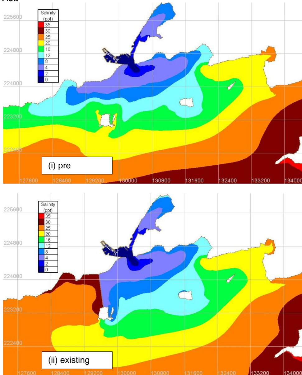
Figure Error! No text of specified style in document..120 Tidal Average Salinity –Spring Tides –Corrib Low Flow
