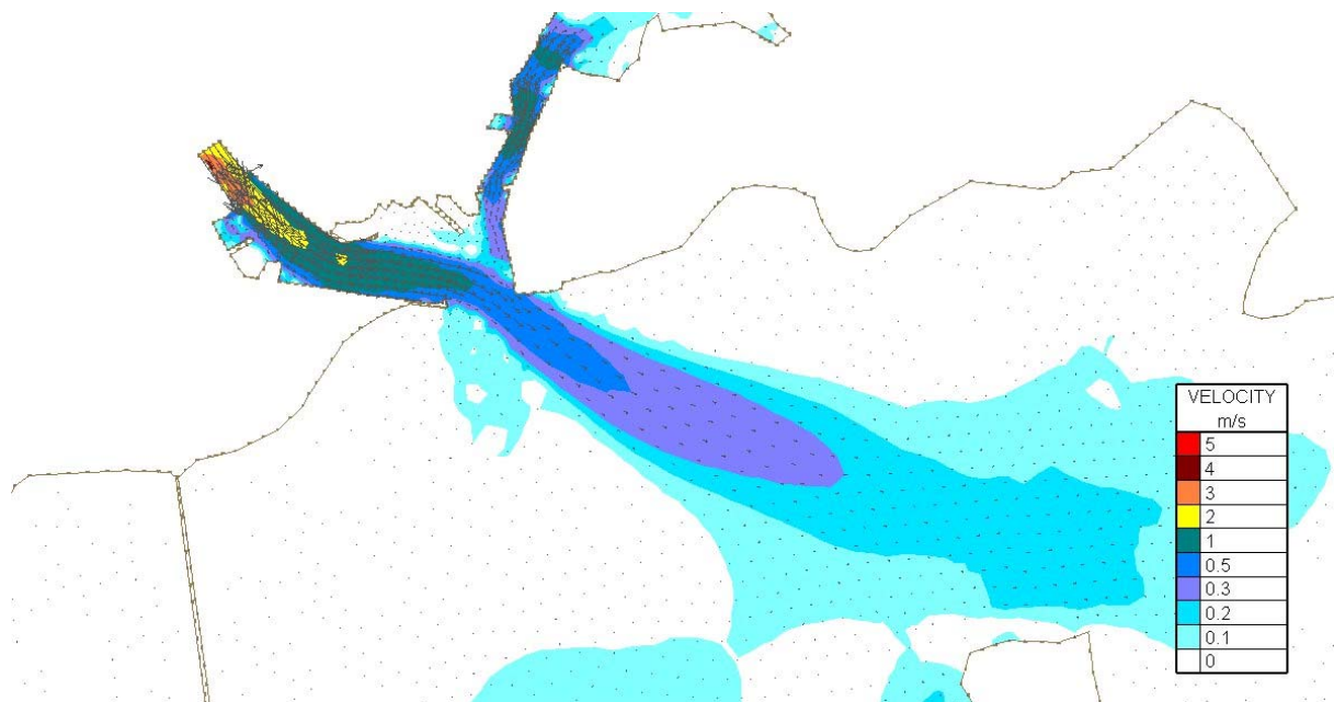
Figure Error! No text of specified style in document..173 Velocity Magnitudes at Mid Flood (3.1hrs before highwater Tide) for Flood Simulation 3 – river plus 20% climate change and a 3.49m tide – Existing Case
