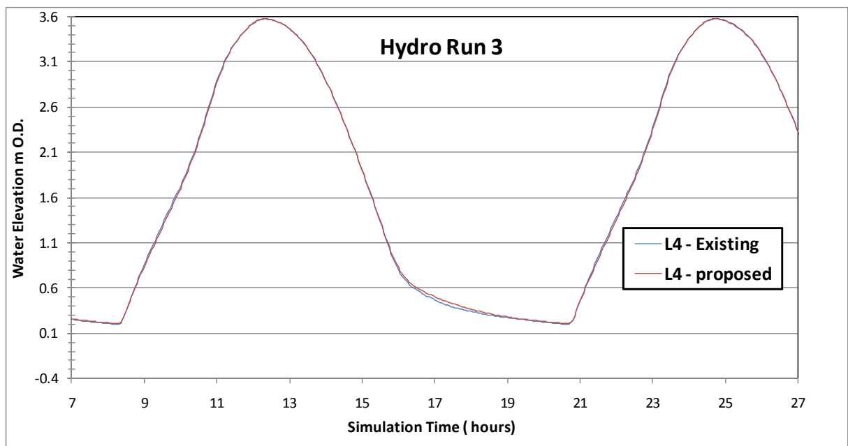
Figure Error! No text of specified style in document..201 Flood level comparison between existing and proposed for Hydrodynamic Simulation No. 3 at reference site 4 – entrance channel to Lough Atalia
