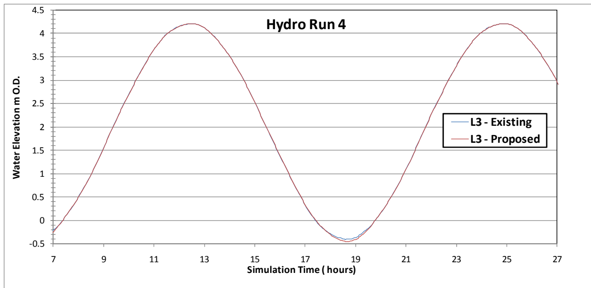
Figure Error! No text of specified style in document..206 Flood level comparison between existing and proposed for Hydrodynamic Simulation No. 4 at reference site 3 in estuary inside Nimmo's Pier
