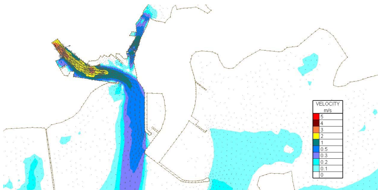
Figure Error! No text of specified style in document..154 Velocity Magnitudes at Mid-ebb (3.1hrs after highwater ) for Flood Simulation 1- 100 year river flow and mean spring tide – Proposed Harbour Extension Case
