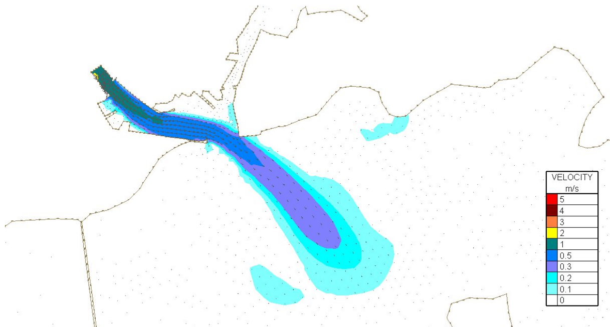
Figure Error! No text of specified style in document..183 Velocity Magnitudes at highwater for Flood Simulation 4 – 100 year river flow and a tide of 4.146m (200 year tide) – Existing Case
