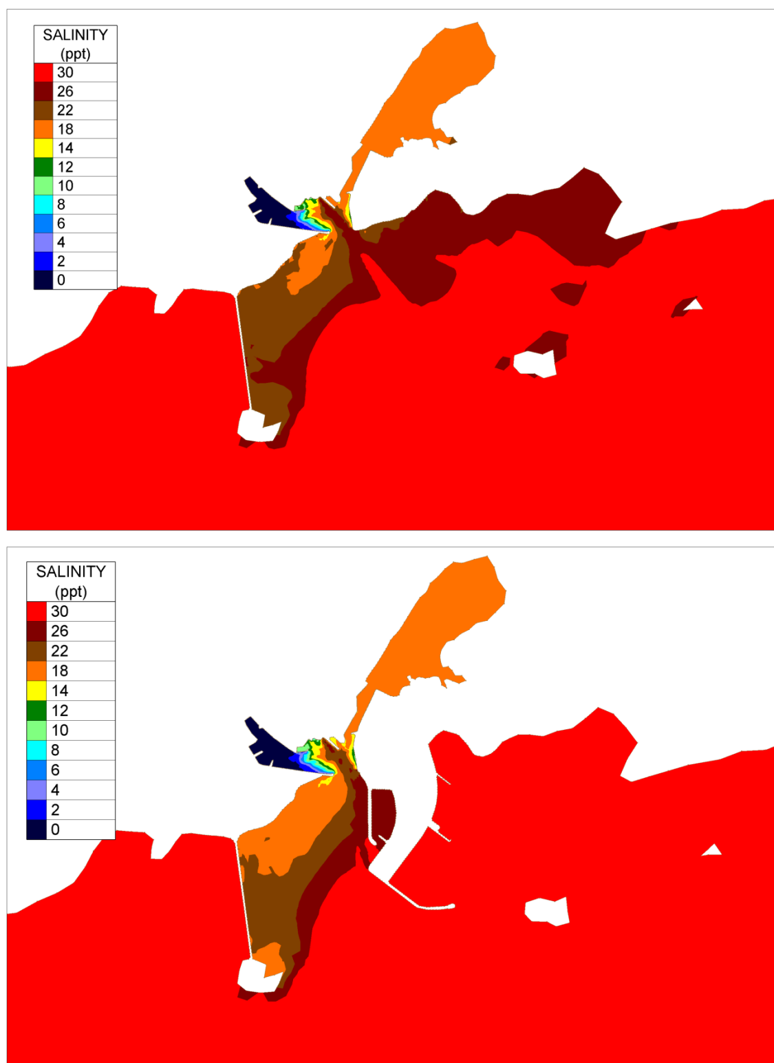
Figure Error! No text of specified style in document..81 Mean Salinity concentration in mid-depth layer for existing and proposed case under 90-percentile Corrib Flow (28.5cumec)
