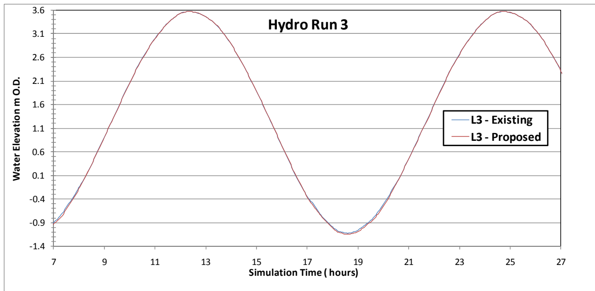
Figure Error! No text of specified style in document..200 Flood level comparison between existing and proposed for Hydrodynamic Simulation No. 3 at reference site 3 in estuary inside Nimmo's Pier
