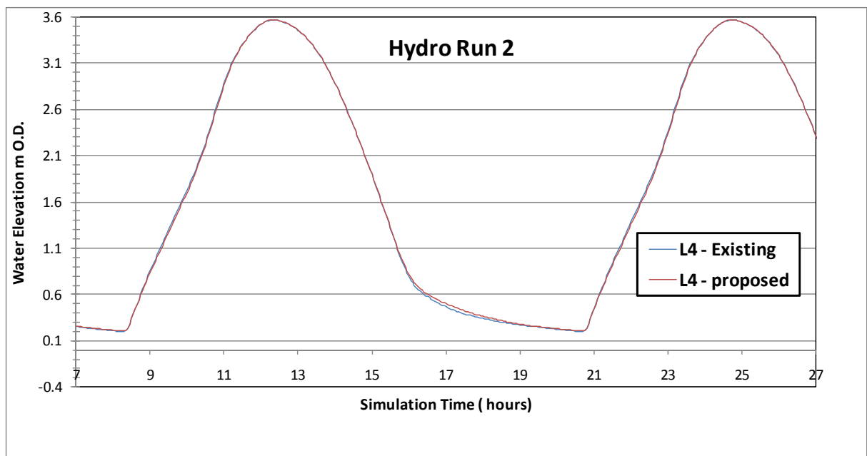
Figure Error! No text of specified style in document..195 Flood level comparison between existing and proposed for Hydrodynamic Simulation No. 2 at reference site 4 – entrance channel to Lough Atalia
