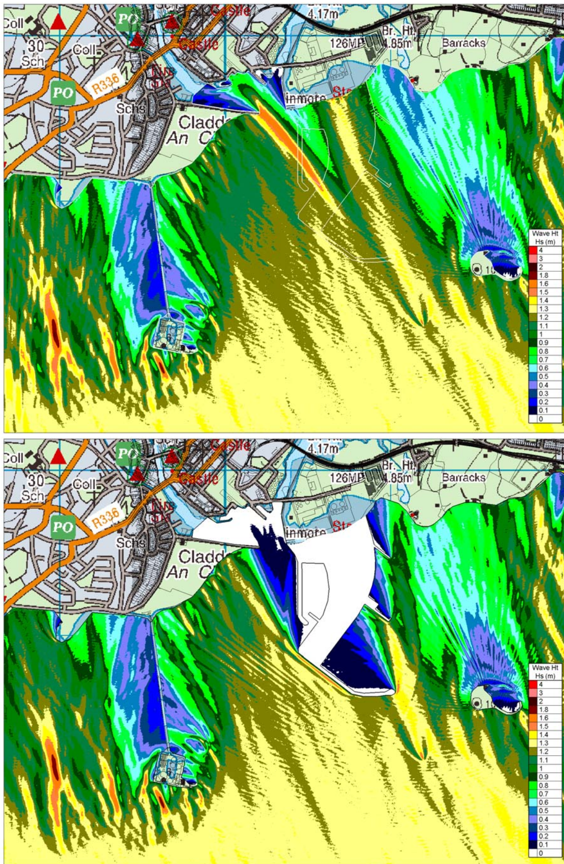
Figure Error! No text of specified style in document..137 ARTEMIS Significant Wave Heights for local Design Storm Waves from the South-South-East for Existing and Proposed Case
