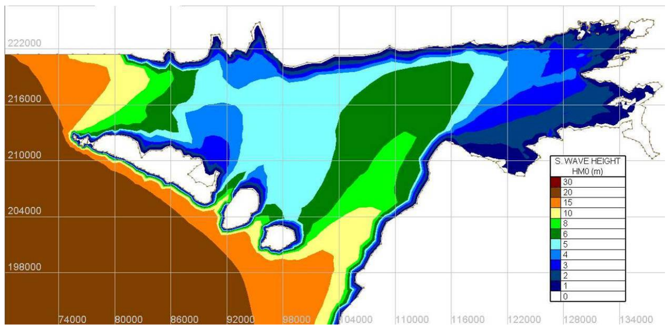
Figure Error! No text of specified style in document..130 Wave climate under 50-year southwest wind conditions
