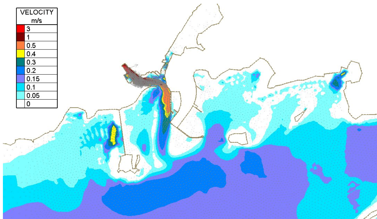
Figure Error! No text of specified style in document..16 - Depth averaged velocities Mid-Flood Spring tide and 100 year Corrib Flow with new development
