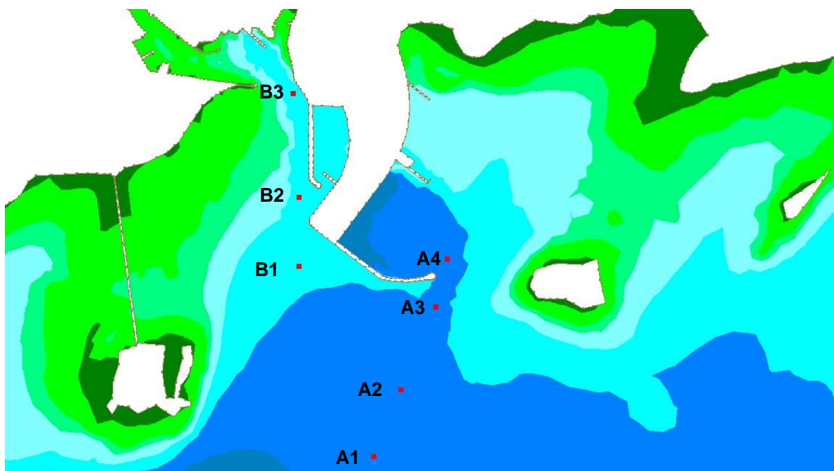
Figure Error! No text of specified style in document..51 Reference locations along approach dredged channels to old Docks and proposed commercial port to assess suspended solids plume impact maintenance dredge operations
