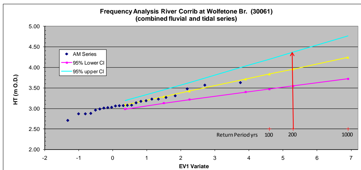
Figure Error! No text of specified style in document..148 EV1 Fit of the Corrib Estuary Gauge at Wolfe Tone Bridge Gauge AM highwater series showing upper and lower 95-percentile confidence interval
