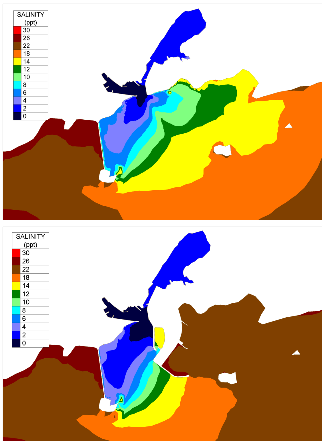
Figure Error! No text of specified style in document..88 Mean Salinity concentration in surface layer for existing and proposed cases under 10-percentile Corrib Flow (200cumec)
