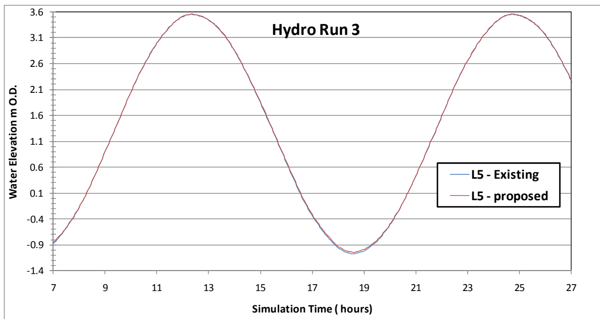
Figure Error! No text of specified style in document..202 Flood level comparison between existing and proposed for Hydrodynamic Simulation No. 3 at reference site 5 – new dredge channel at Marina Breakwater
