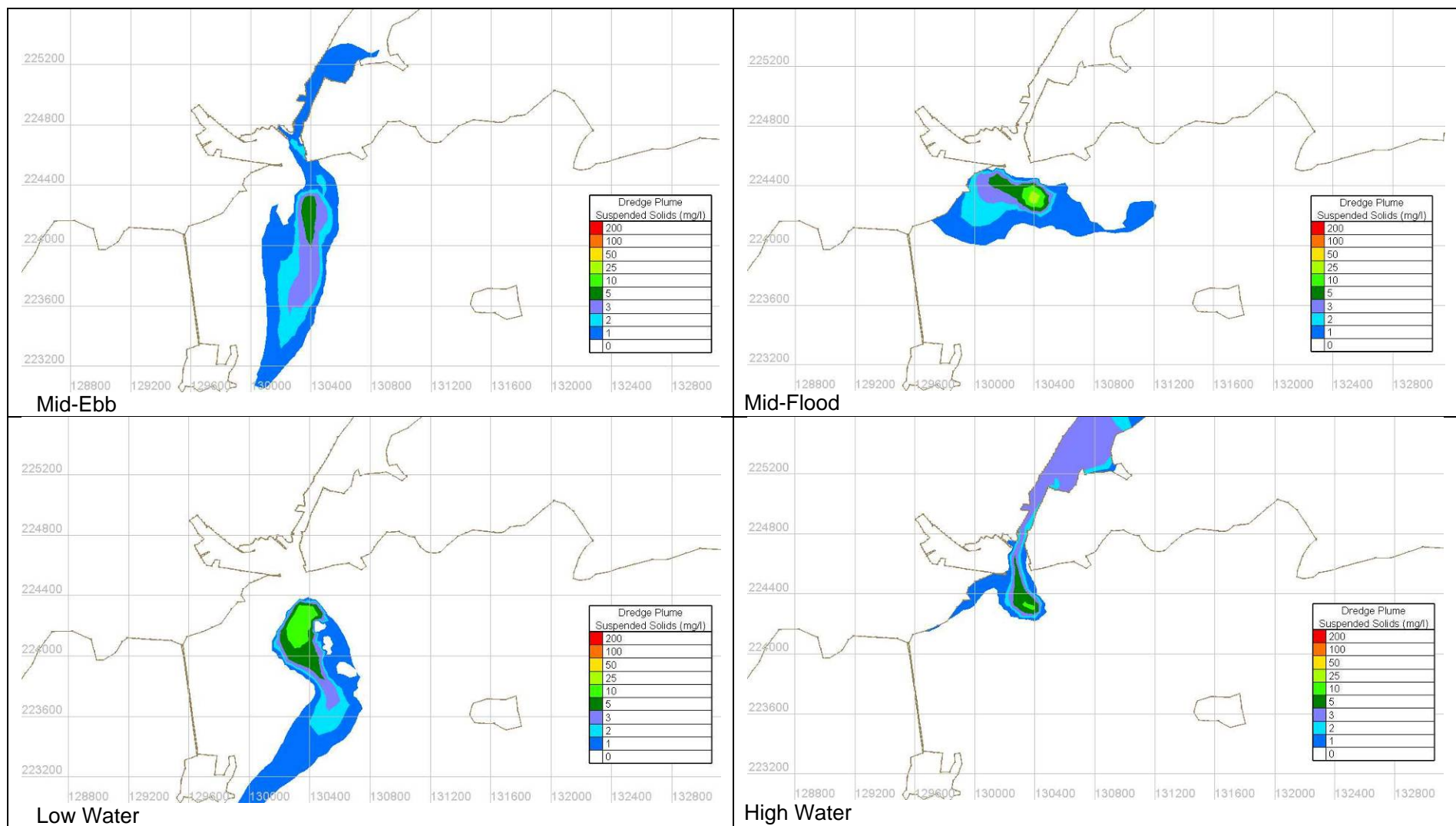
Figure Error! No text of specified style in document..44 Fine silt suspended sediment plume simulation at dredge location 1 – Spring tide and Corrib Summer low flow
