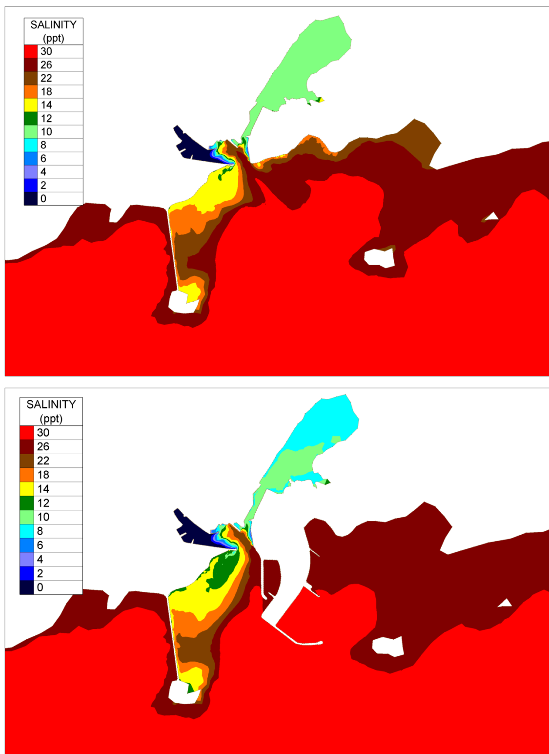
Figure Error! No text of specified style in document..83 Mean Salinity concentration in bottom layer for existing and proposed cases under 50-percentile Corrib Flow (82cumec)
