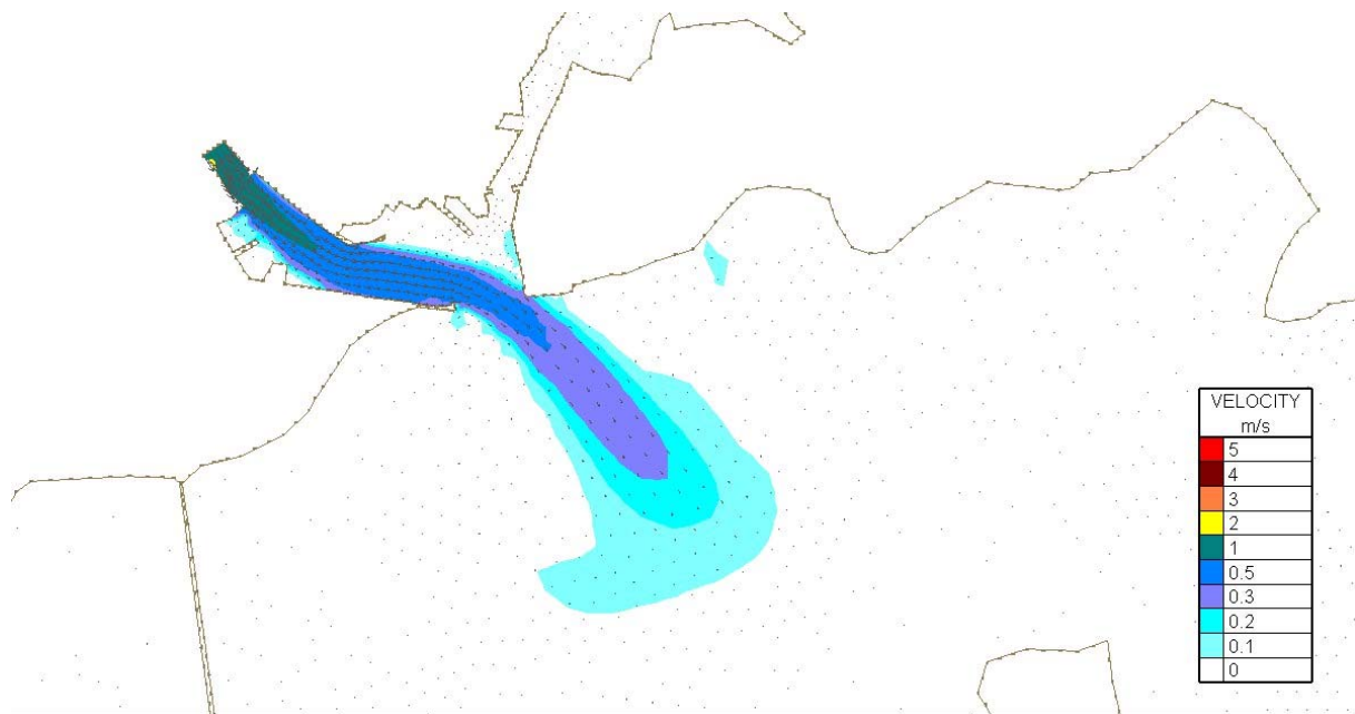
Figure Error! No text of specified style in document..167 Velocity Magnitudes at highwater for Flood Simulation 2 – 100 year river flow and a 3.49m tide – Existing Case
