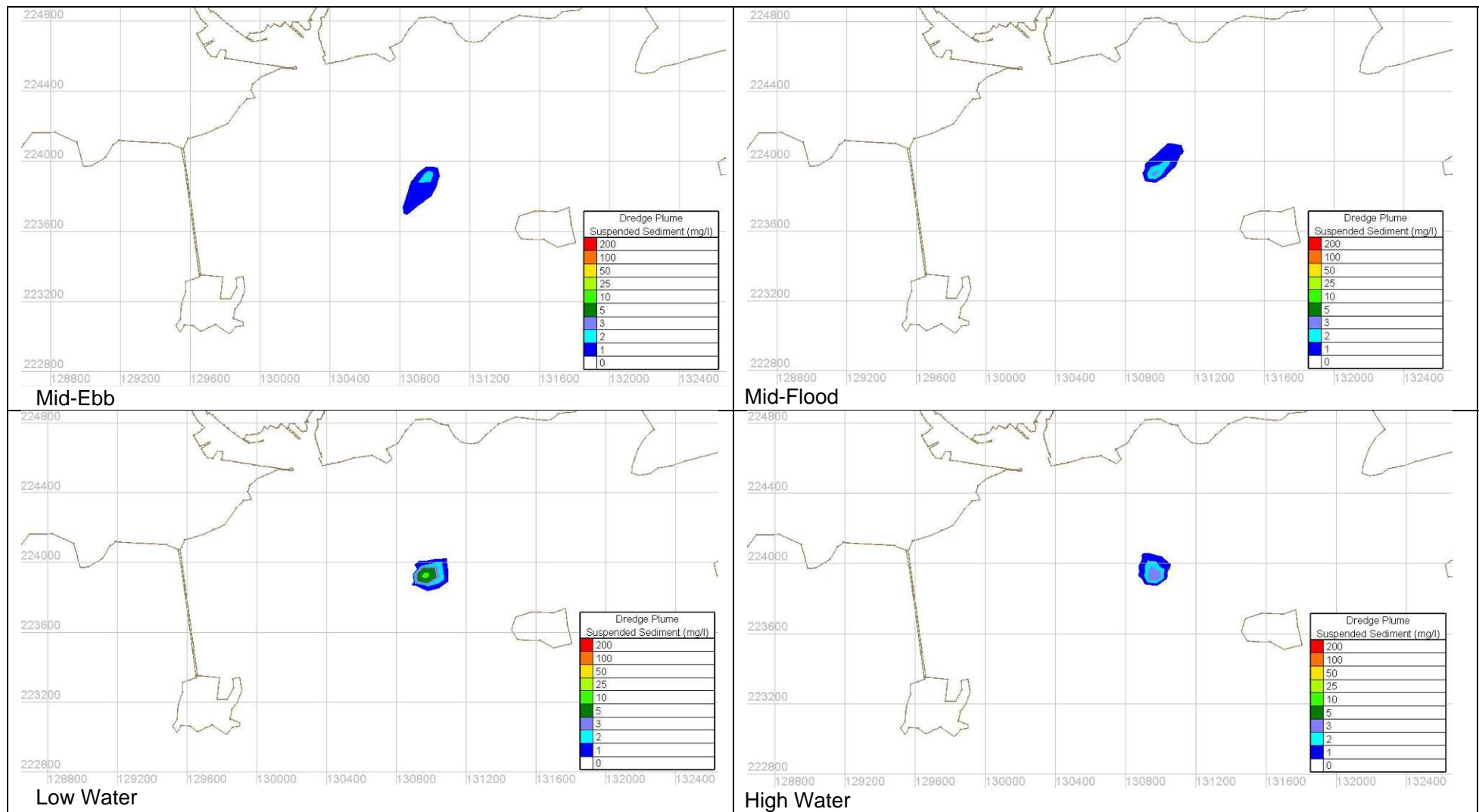
Figure Error! No text of specified style in document..47 Coarse silt suspended sediment plume simulation at dredge location 3 – Spring tide and Corrib Summer low flow
