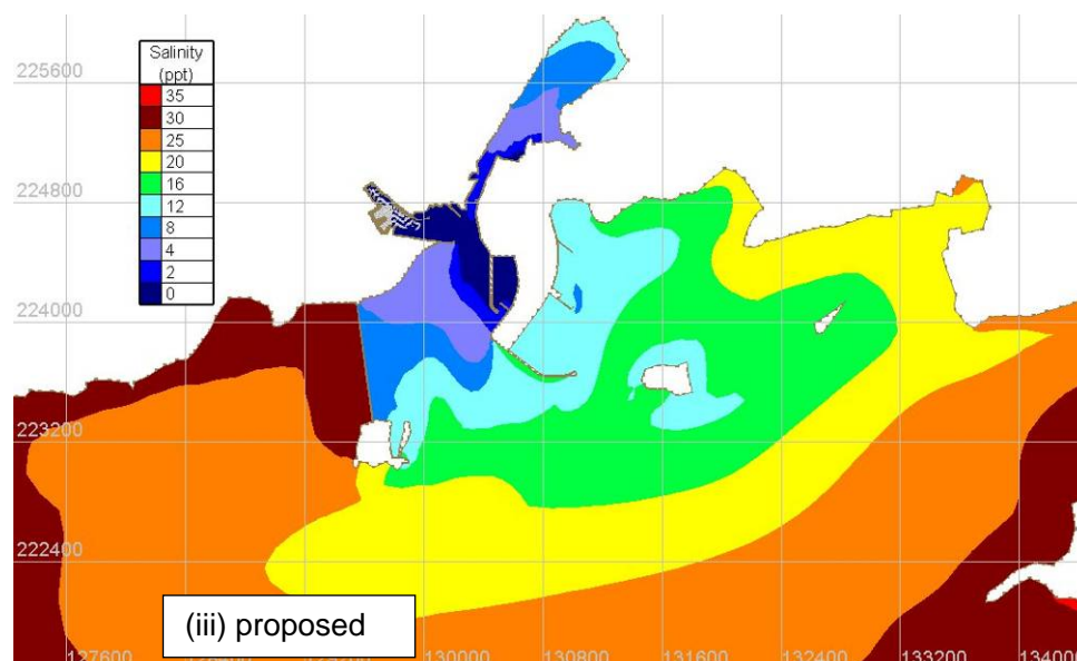
Figure Error! No text of specified style in document..121 Tidal Average Salinity –Spring Tides – median Corrib Flow
