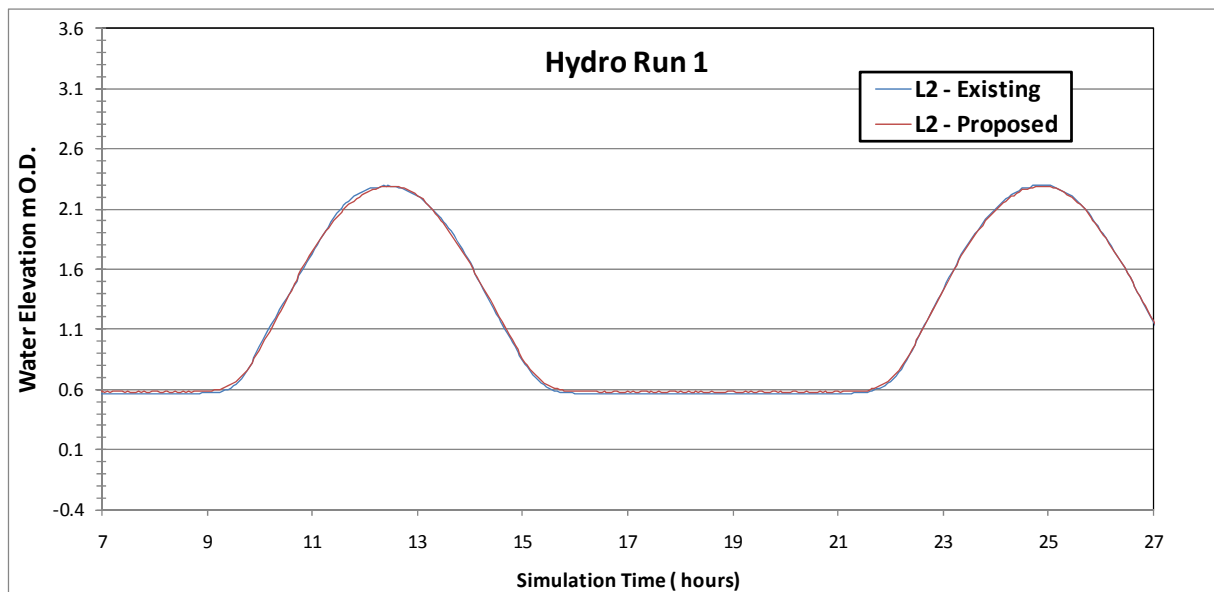
Figure Error! No text of specified style in document..187 Flood level comparison between existing and proposed for Hydrodynamic Simulation No. 1 at reference site 2 in Claddagh Basin
