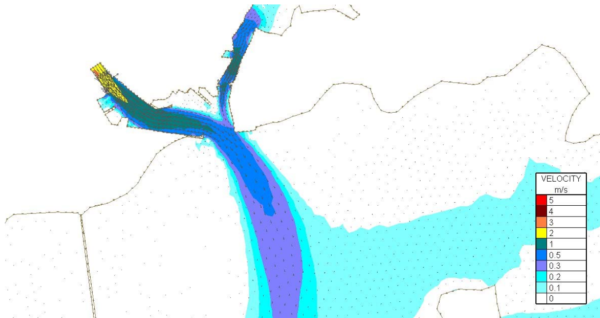
Figure Error! No text of specified style in document..161 Velocity Magnitudes at Mid-ebb (3.1hrs after highwater ) for Flood Simulation 2- 100 year river flow and a 3.44m tide – Existing Case
