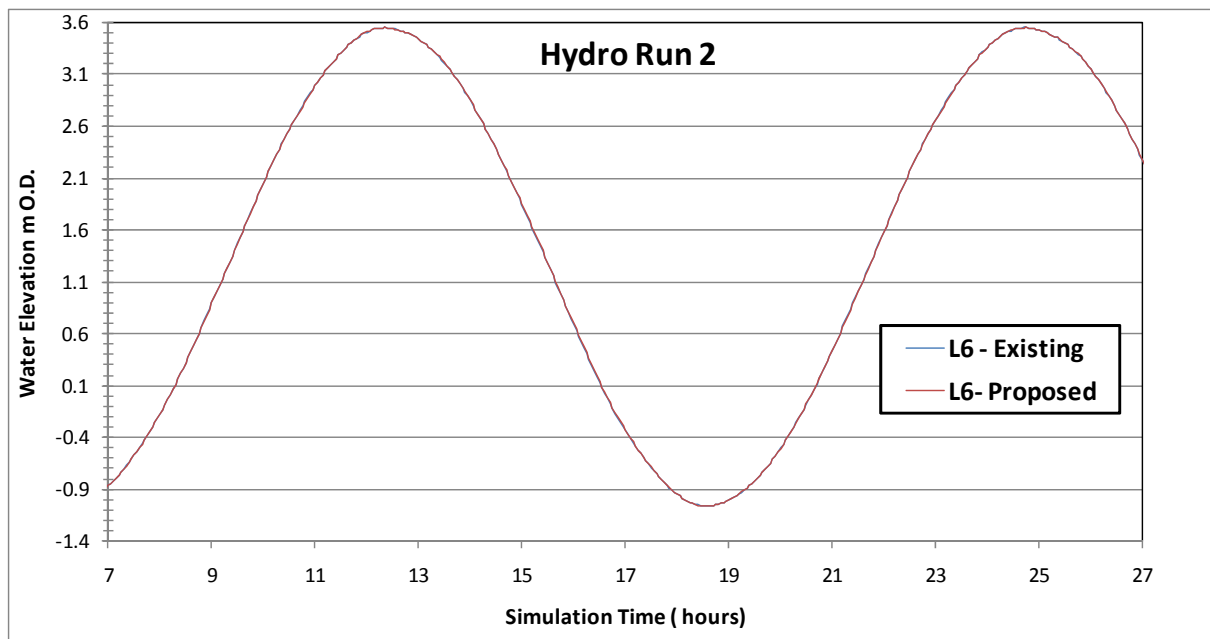
Figure Error! No text of specified style in document..197 Flood level comparison between existing and proposed for Hydrodynamic Simulation No. 2 at reference site 6 – new dredge channel south of Marina entrance
