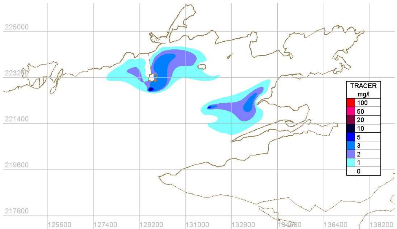
Figure Error! No text of specified style in document..98 High Water - Existing Case - Spring tides
