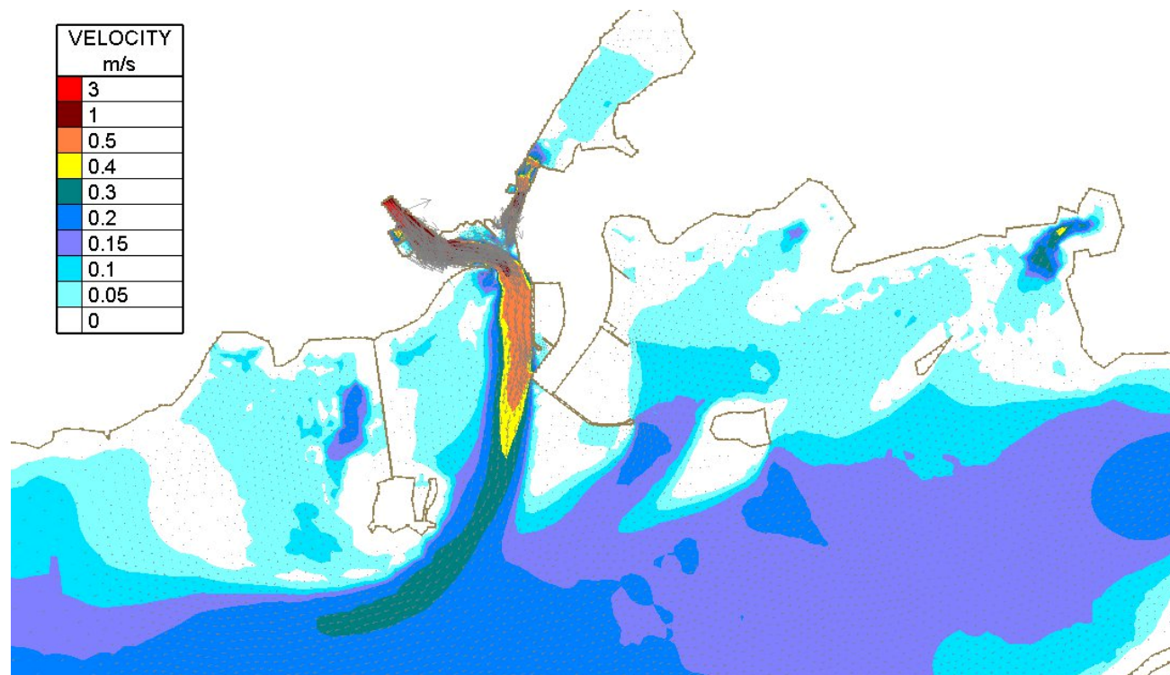
Figure Error! No text of specified style in document..14 - Depth averaged velocities Mid-ebb Spring Tide and 100 year Corrib Flow with new development
