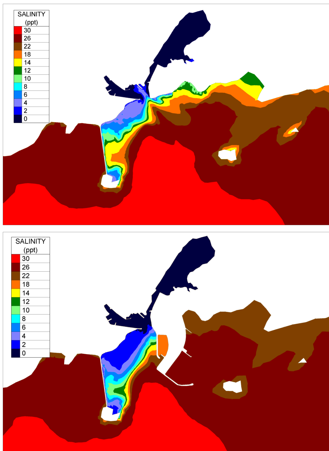
Figure Error! No text of specified style in document..89 Mean Salinity concentration in bottom layer for existing and proposed cases under 1-percentile Corrib Flood Flow (272cumec)
