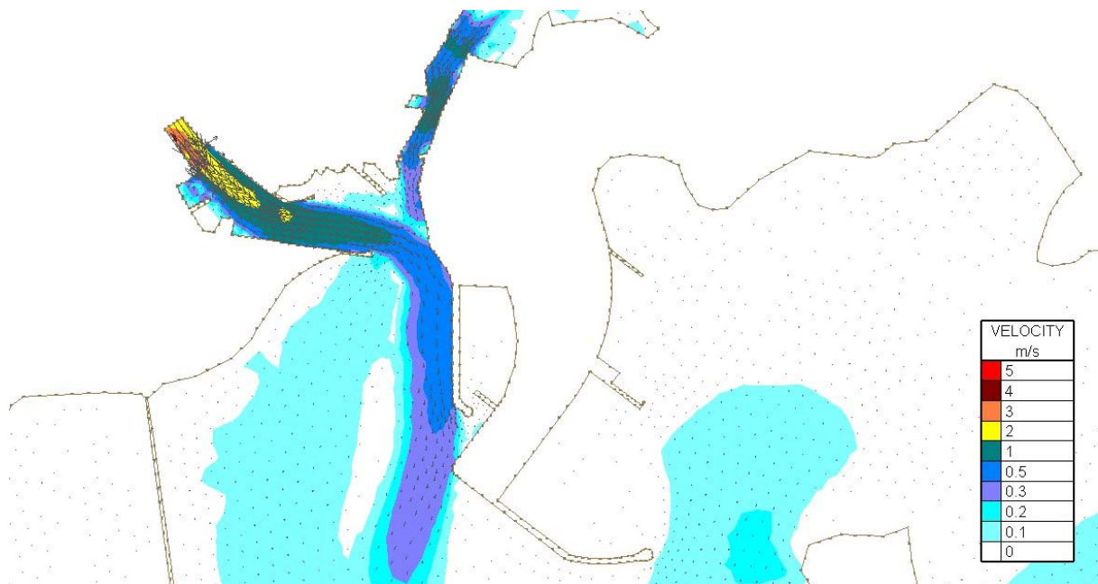
Figure Error! No text of specified style in document..174 Velocity Magnitudes at Mid Flood (3.1hrs before highwater Tide) for Flood Simulation 3 – river plus 20% climate change and a 3.49m tide – Proposed Harbour Extension Case
