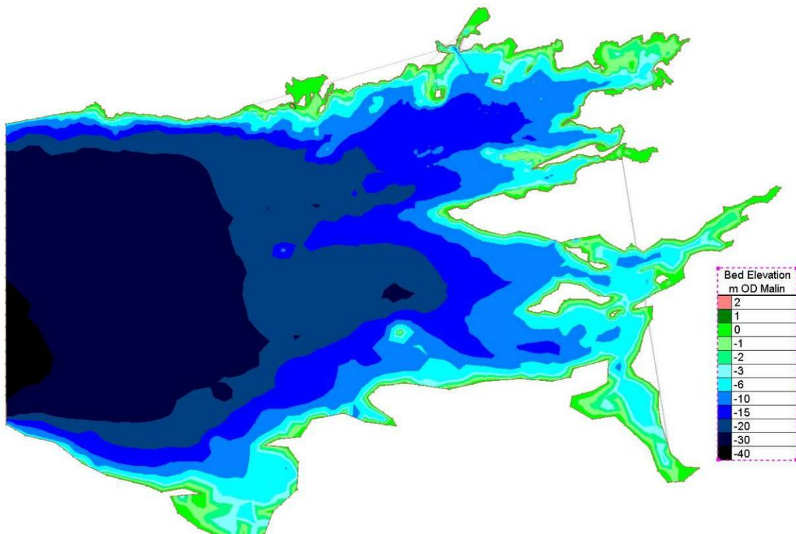
Figure Error! No text of specified style in document..150 Hydrodynamic Model Finite element domain area and bathymetry for existing case
