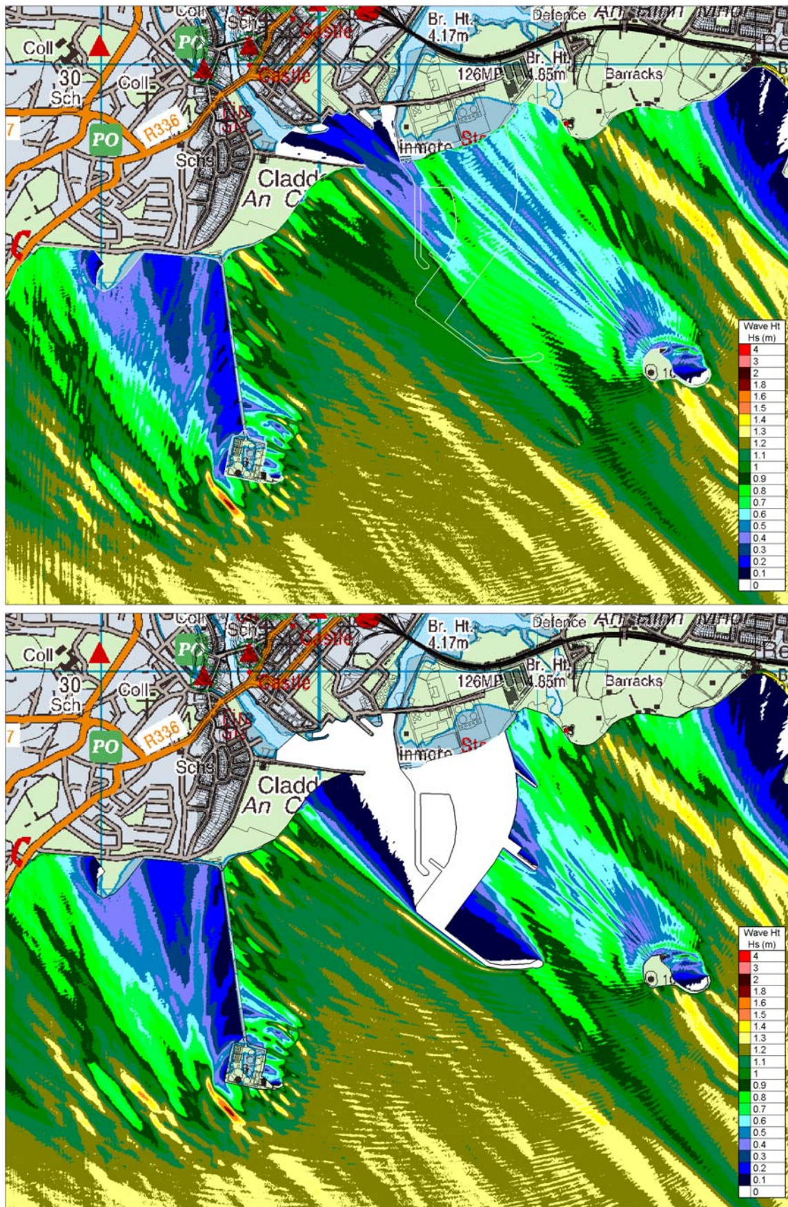
Figure Error! No text of specified style in document..138 ARTEMIS Significant Wave Heights for local Design Storm Waves from the South-East for Existing and Proposed Case
