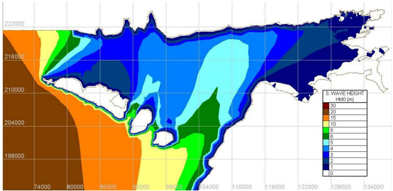
Figure Error! No text of specified style in document..129 Wave climate under 50-year southerly wind conditions
