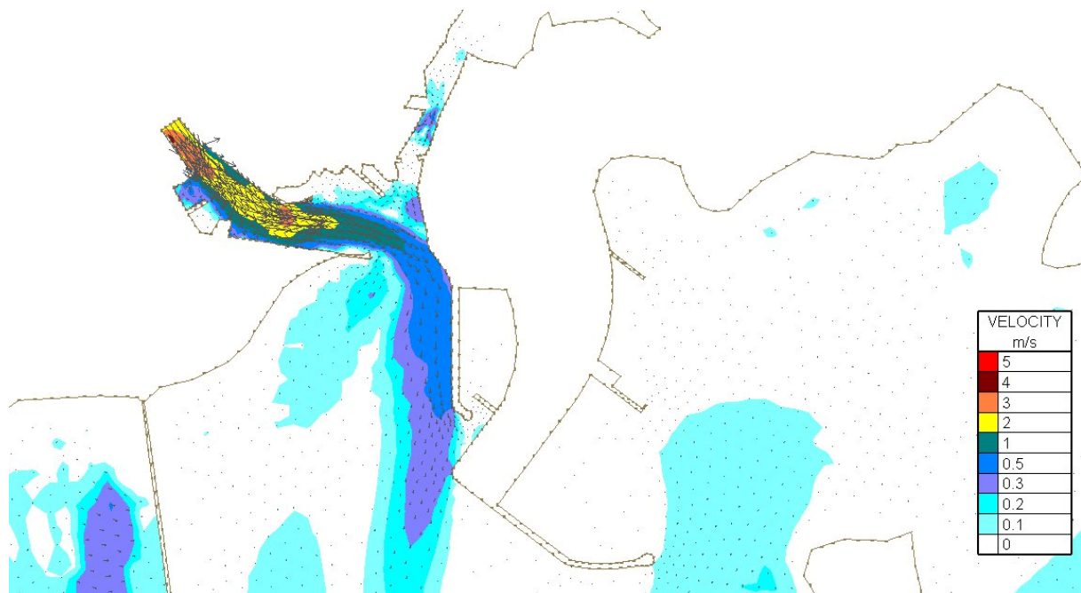
Figure Error! No text of specified style in document..158 Velocity Magnitudes at Mid Flood (3.1hrs before highwater Tide) for Flood Simulation 1 – 100 year river flow and mean spring tide – Proposed Harbour Extension Case
