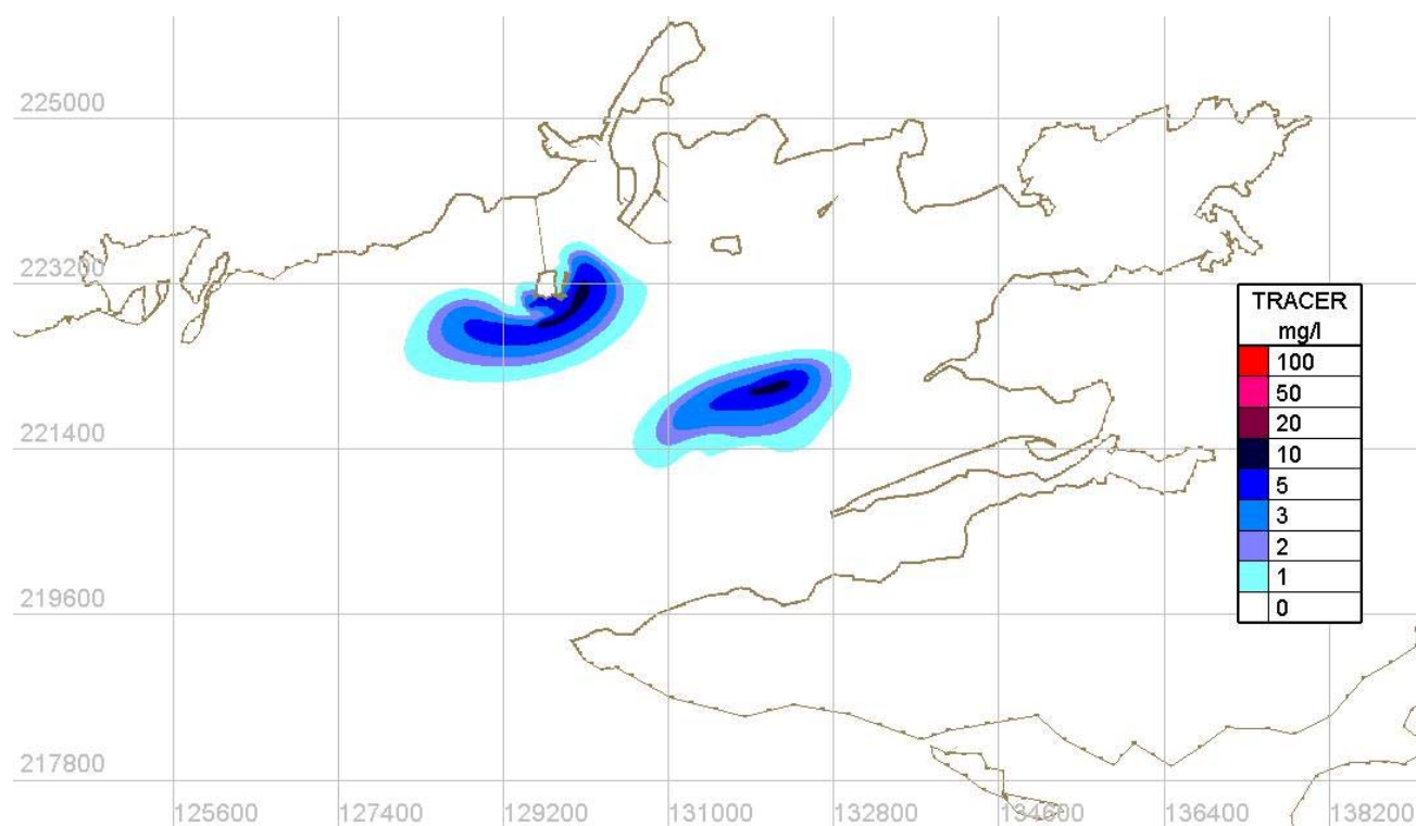
Figure Error! No text of specified style in document..105 Mid Flood - Proposed Case - Neap tides
