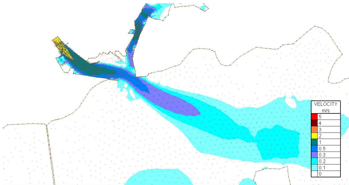
Figure Error! No text of specified style in document..165 Velocity Magnitudes at Mid Flood (3.1hrs before highwater Tide) for Flood Simulation 2 – 100 year river flow and a 3.49m tide – Existing Case
