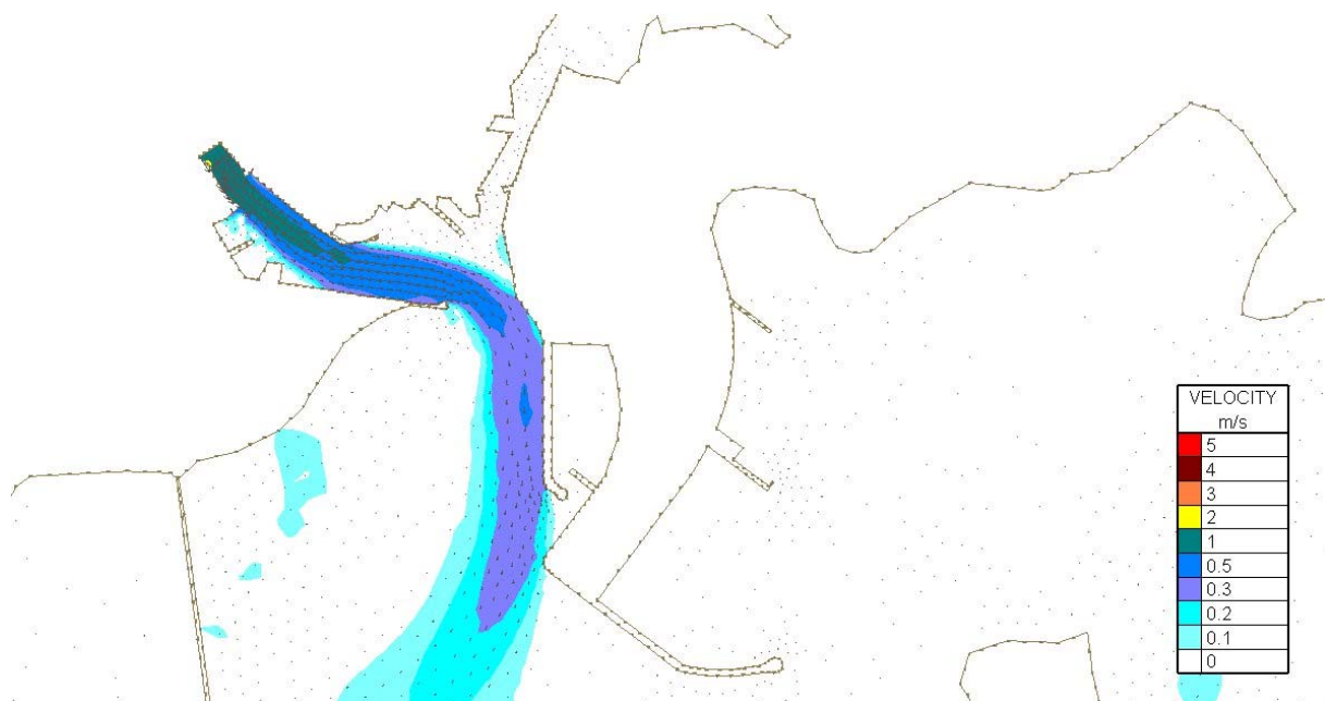
Figure Error! No text of specified style in document..168 Velocity Magnitudes at highwater for Flood Simulation 2– 100 year river flow and a 3.49m tide – Proposed Harbour Extension Case
