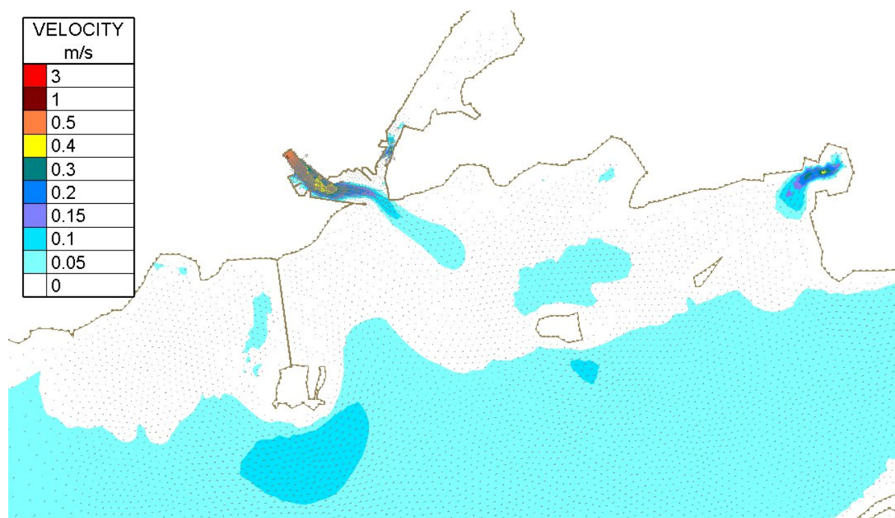
Figure Error! No text of specified style in document..11 - Depth averaged velocities Mid-Flood Neap tide Median Corrib Flow
