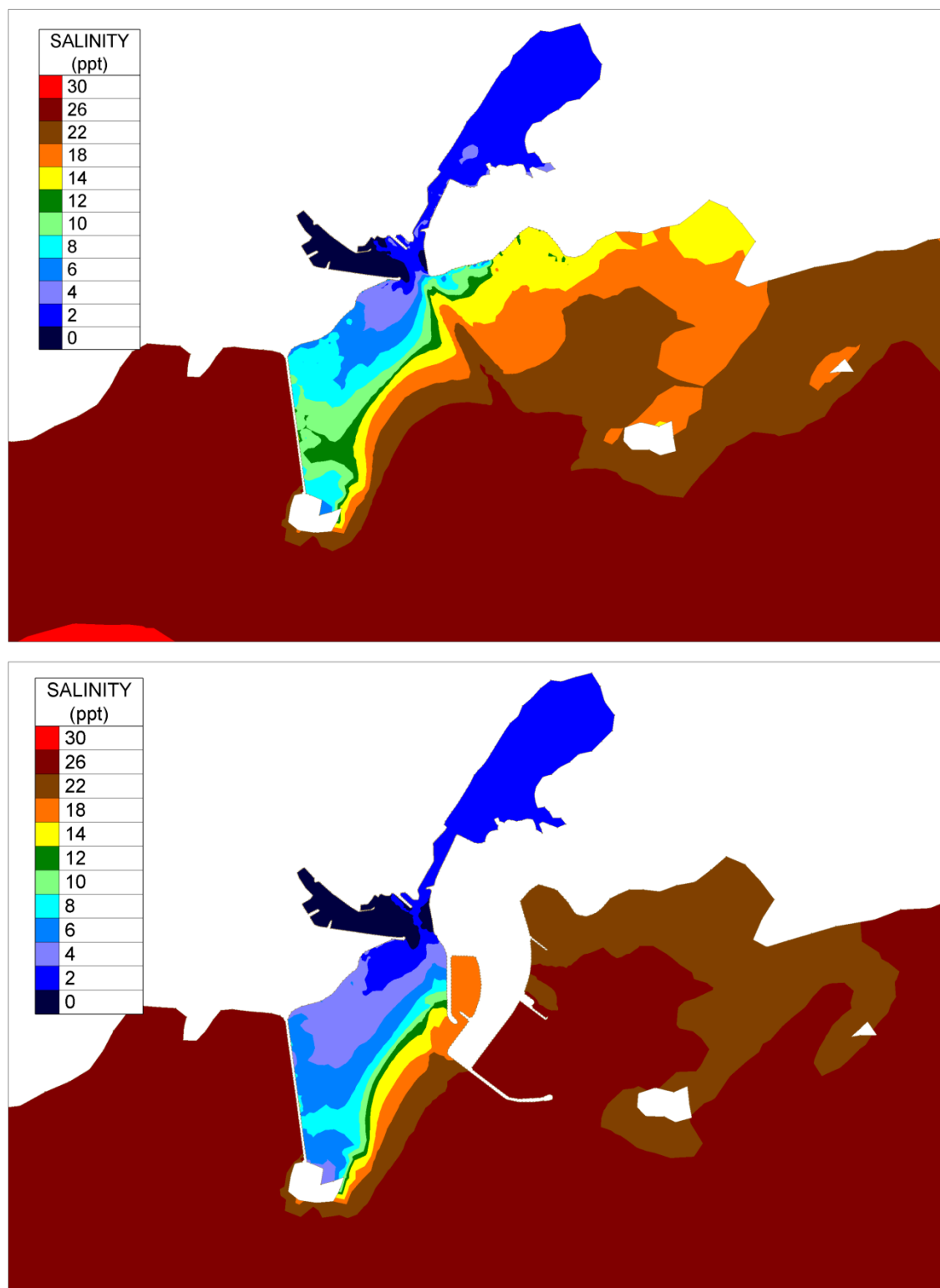
Figure Error! No text of specified style in document..87 Mean Salinity concentration in mid-depth layer for existing and proposed cases under 10-percentile Corrib Flow (200cumec)
