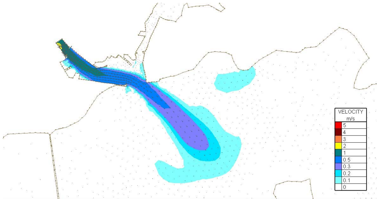
Figure Error! No text of specified style in document..175 Velocity Magnitudes at highwater for Flood Simulation 3 – river plus 20% climate change and a 3.49m tide – Existing Case
