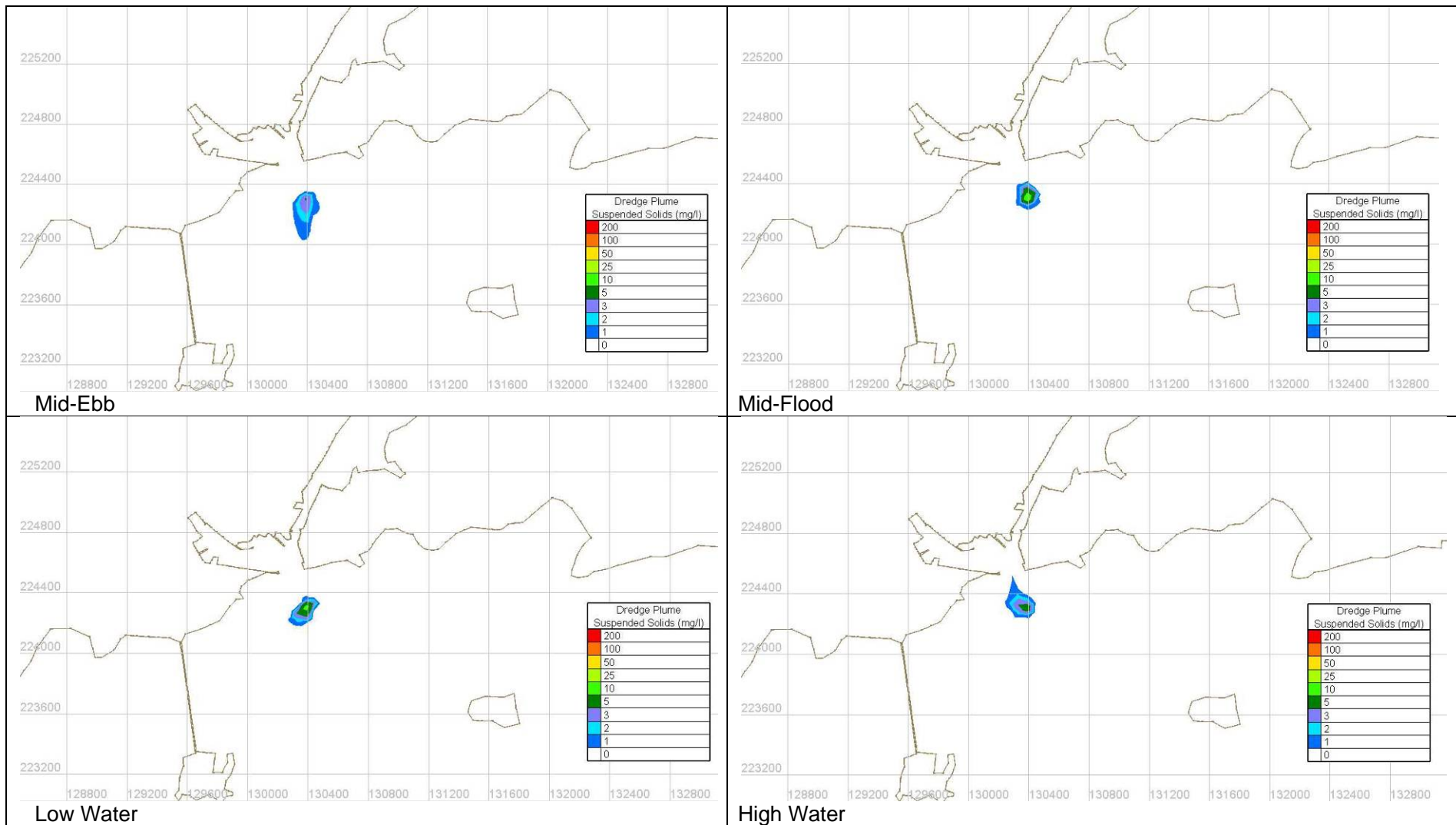
Figure Error! No text of specified style in document..43- Coarse silt suspended sediment plume simulation at dredge location 1 – Spring tide and Corrib Summer low flow
