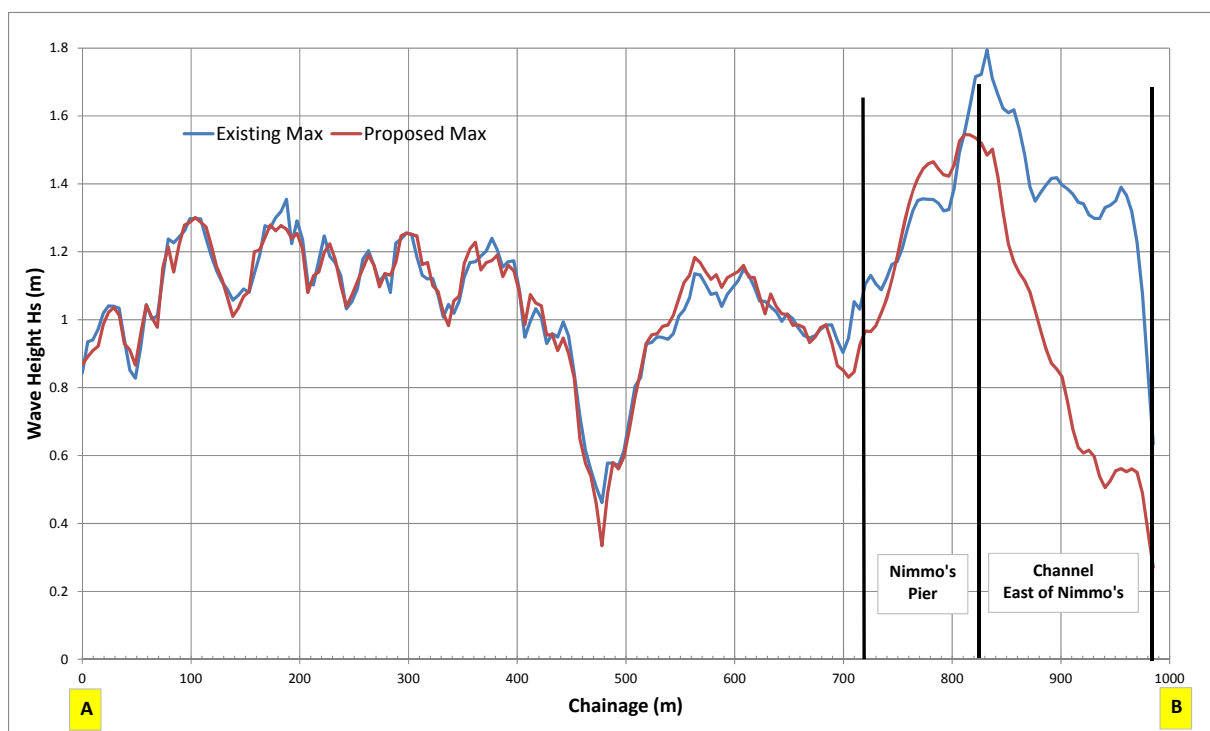
Figure Error! No text of specified style in document..142 Computed maximum wave heights H_s for all onshore directions from WSW to ESE along Section A-B for Existing and Proposed Cases.
