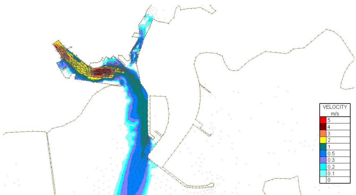
Figure Error! No text of specified style in document..156 Velocity Magnitudes at Low Water (6.2hrs after highwater Tide) for Flood Simulation 1- 100 year river flow and mean spring tide – Proposed Harbour Extension Case
