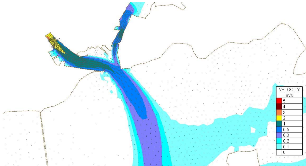
Figure Error! No text of specified style in document..177 Velocity Magnitudes at Mid-ebb (3.1hrs after highwater ) for Flood Simulation 4 – 100 year river flow and a tide of 4.146m (200 year tide) – Existing Case
