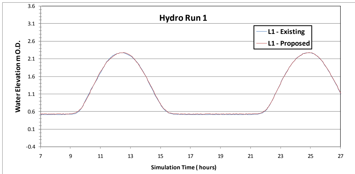
Figure Error! No text of specified style in document..186 Flood level comparison between existing and proposed for Hydrodynamic Simulation No. 1 at reference site 1 in Claddagh Basin adjacent to Spanish Arch
