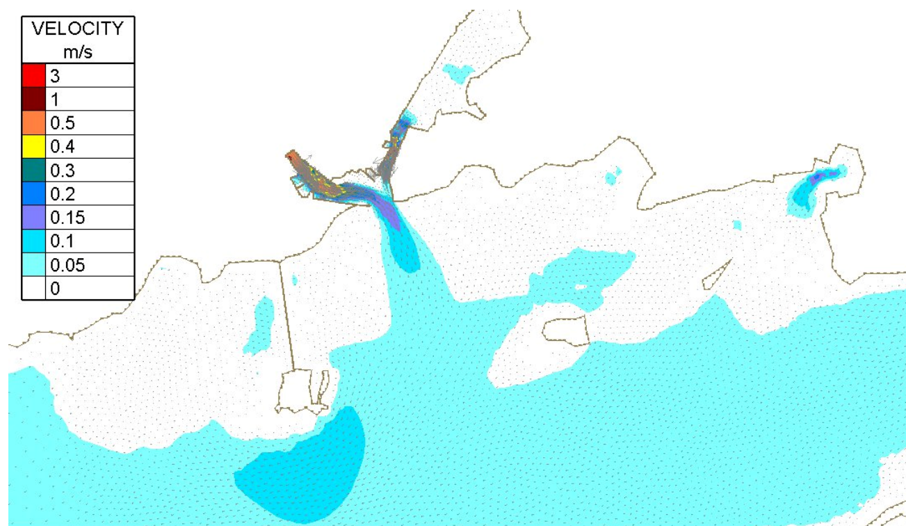
Figure Error! No text of specified style in document..9 - Depth averaged velocities Mid-ebb Neap tide Median Corrib Flow
