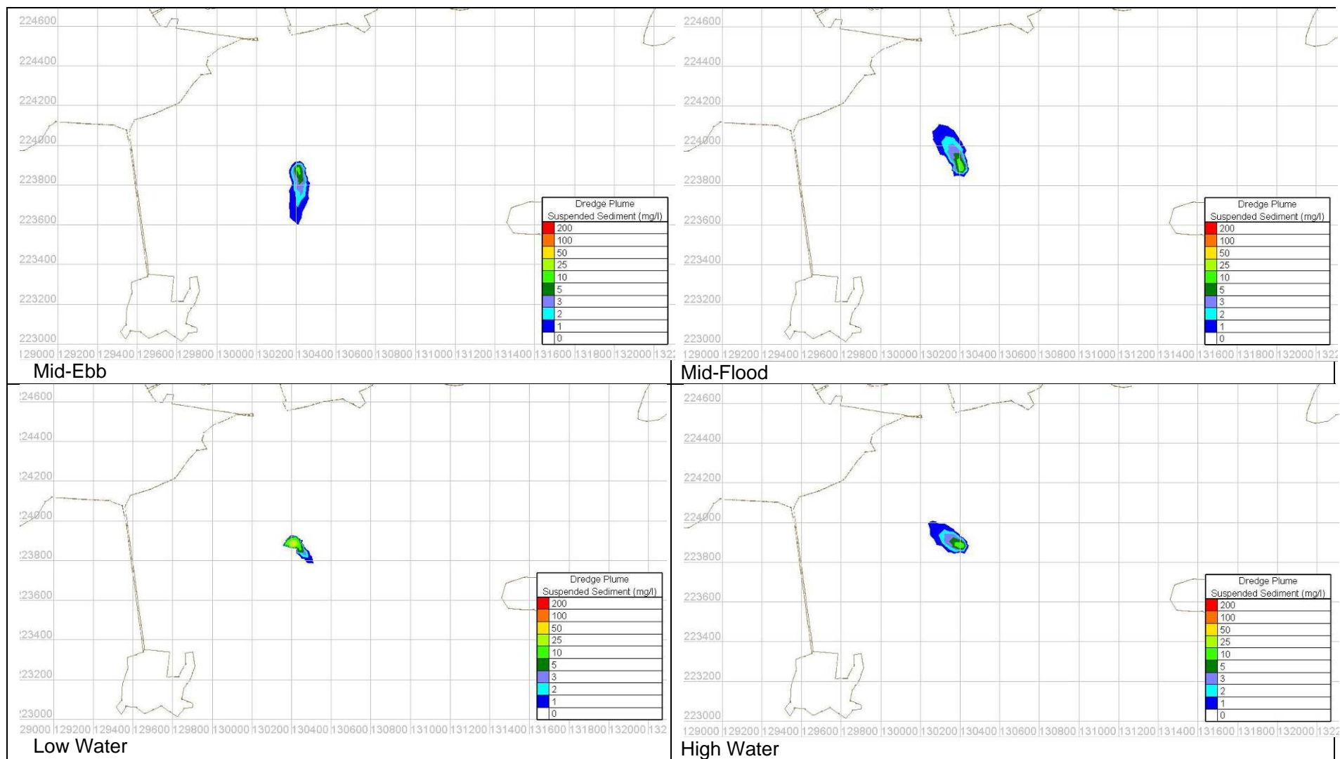
Figure Error! No text of specified style in document..45 Coarse silt suspended sediment plume simulation at dredge location 2 – Spring tide and Corrib Summer low flow
