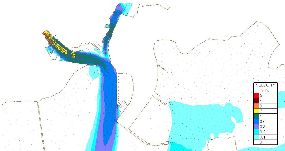
Figure Error! No text of specified style in document..170 Velocity Magnitudes at Mid-ebb (3.1hrs after highwater ) for Flood Simulation 3- river plus 20% climate change and a 3.49m tide – Proposed Harbour Extension Case
