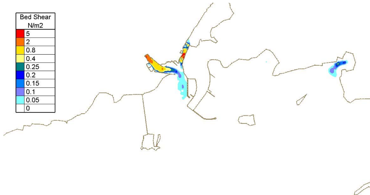
Figure Error! No text of specified style in document..26 - Computed bed shear at mid-ebb with new harbour extension development – Neap Tide and Median River Corrib Flow (82 m 3 /s)
