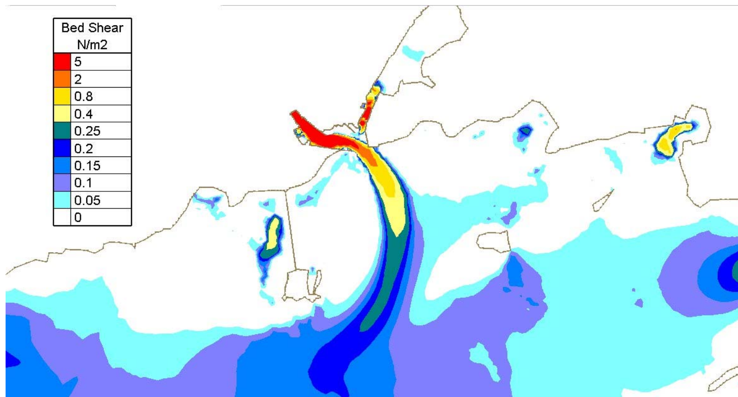
Figure Error! No text of specified style in document..33 - Computed bed shear at mid-ebb Spring Tide with 100 year Corrib Flood Flow for existing case
