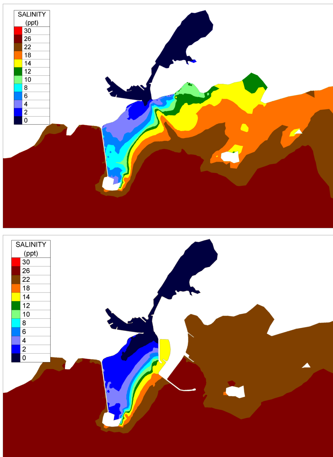
Figure Error! No text of specified style in document..90 Mean Salinity concentration in mid-depth layer for existing and proposed cases under 1-percentile Corrib Flood Flow (272cumec)
