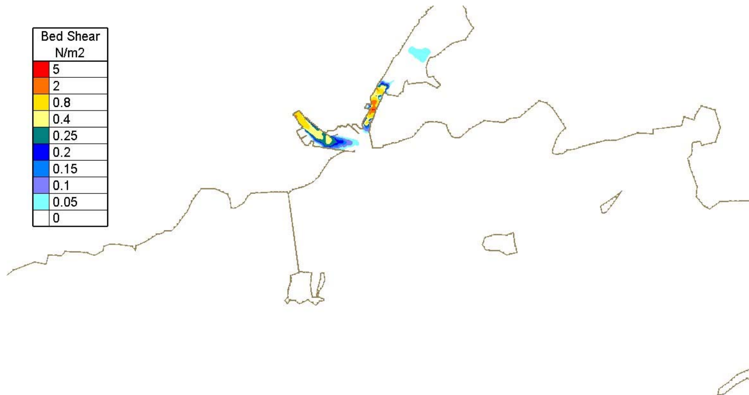
Figure Error! No text of specified style in document..31 - Computed bed shear at mid flood high tide for existing case without development – Neap Tide and Median River Corrib Flow (82 m 3 /s)
