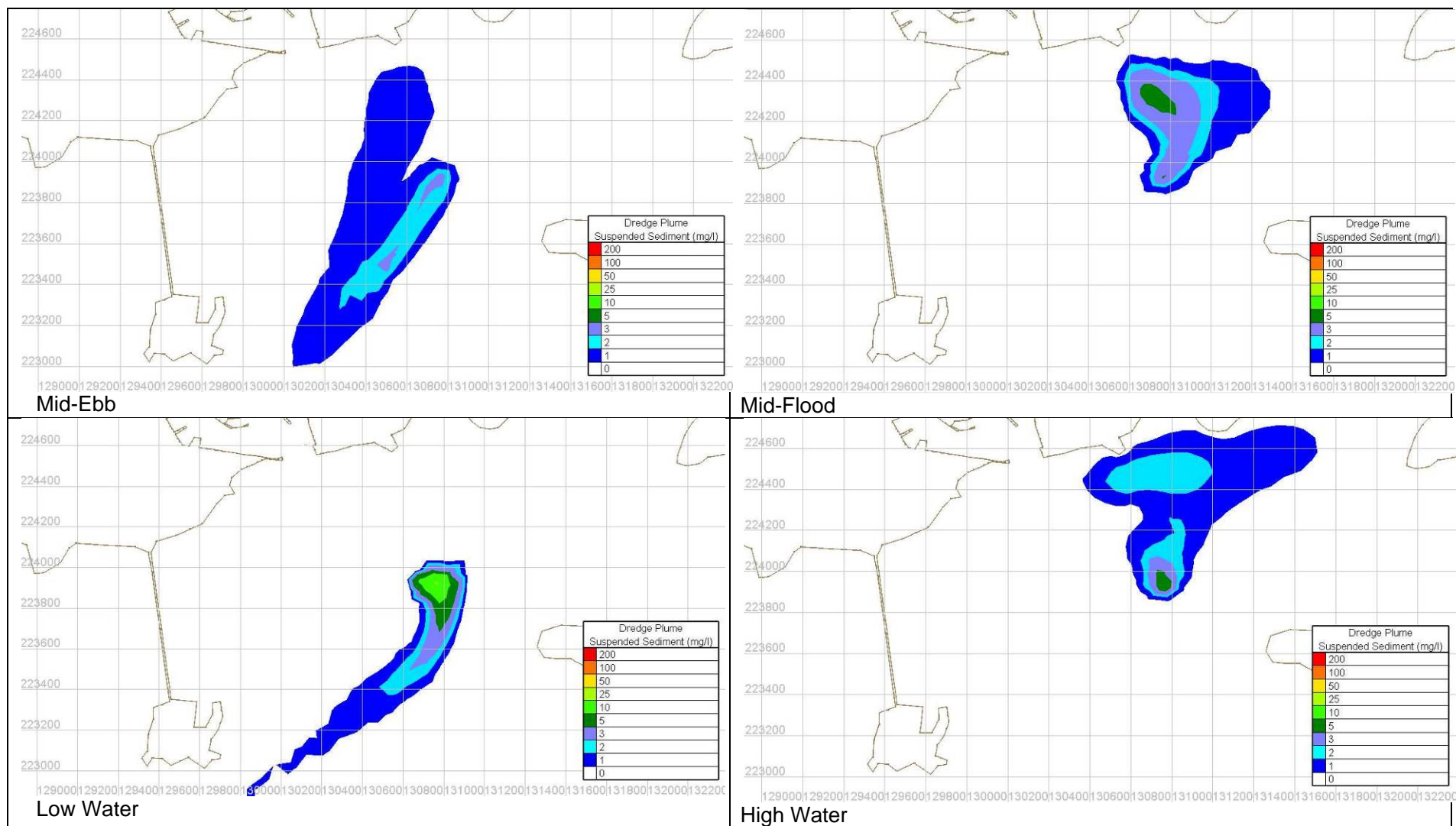
Figure Error! No text of specified style in document..48 Fine silt suspended sediment plume simulation at dredge location 3 – Spring tide and Corrib Summer low flow
