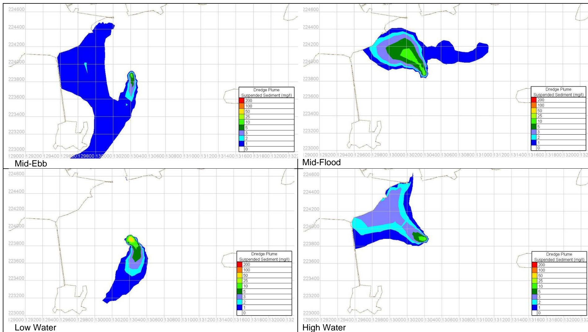
Figure Error! No text of specified style in document..46 Fine silt suspended sediment plume simulation at dredge location 2 – Spring tide and Corrib Summer low flow
