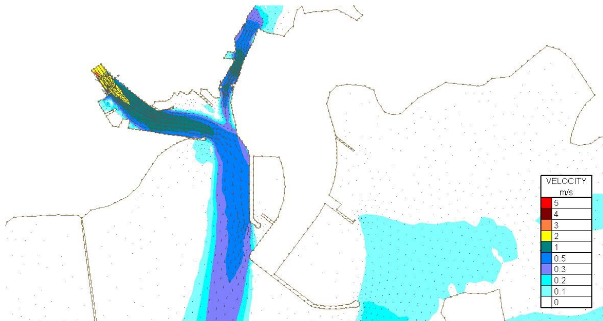
Figure Error! No text of specified style in document..162 Velocity Magnitudes at Mid-ebb (3.1hrs after highwater ) for Flood Simulation 2- 100 year river flow and a 3.44m tide – Proposed Harbour Extension Case
