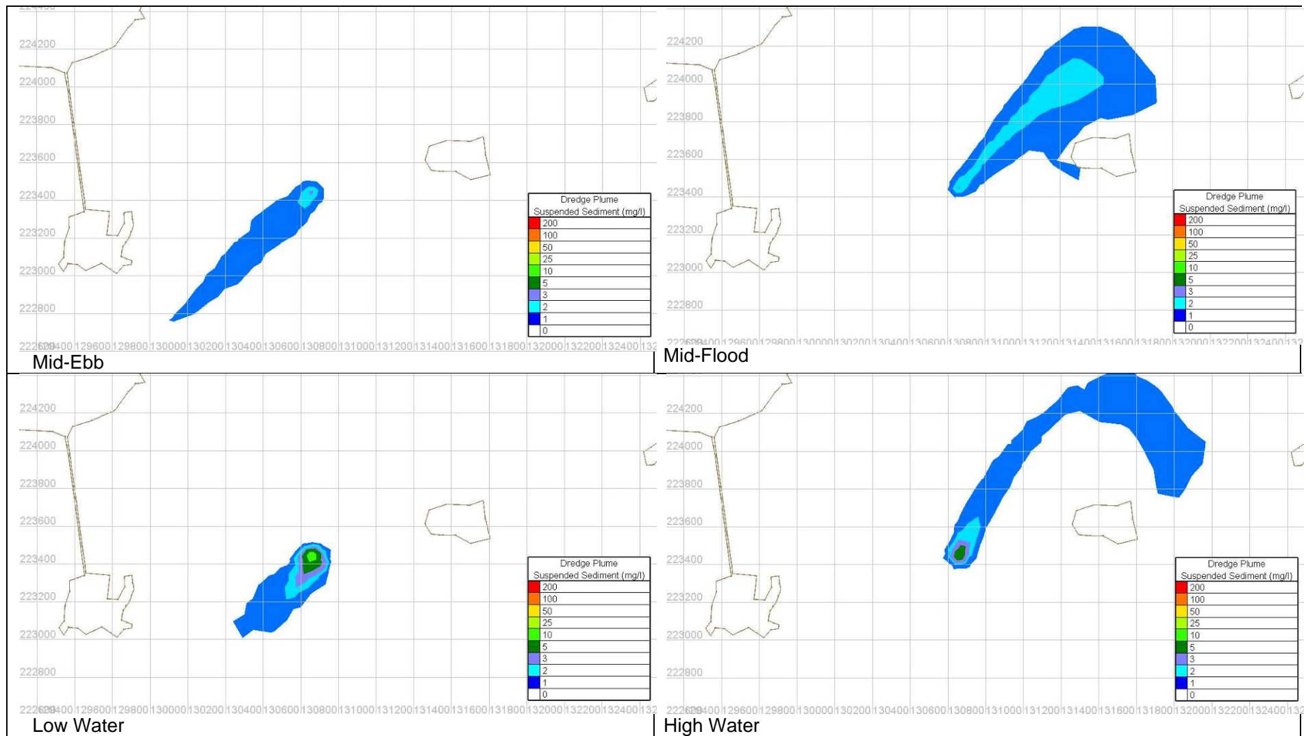
Figure Error! No text of specified style in document...50 Fine silt suspended sediment plume simulation at dredge location 4 – Spring tide and Corrib Summer low flow
