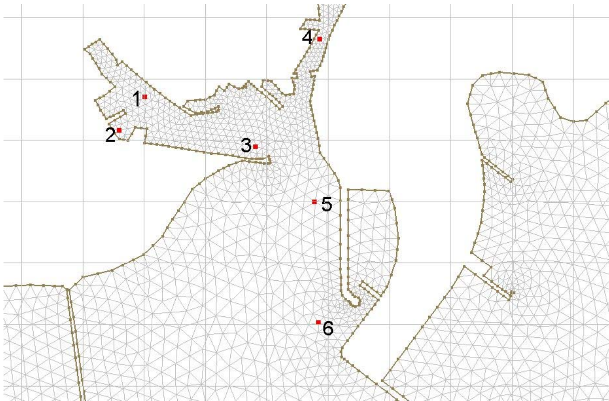
Figure Error! No text of specified style in document..185 Reference sites for time series output of water elevations for analysis runs with and without proposed development
