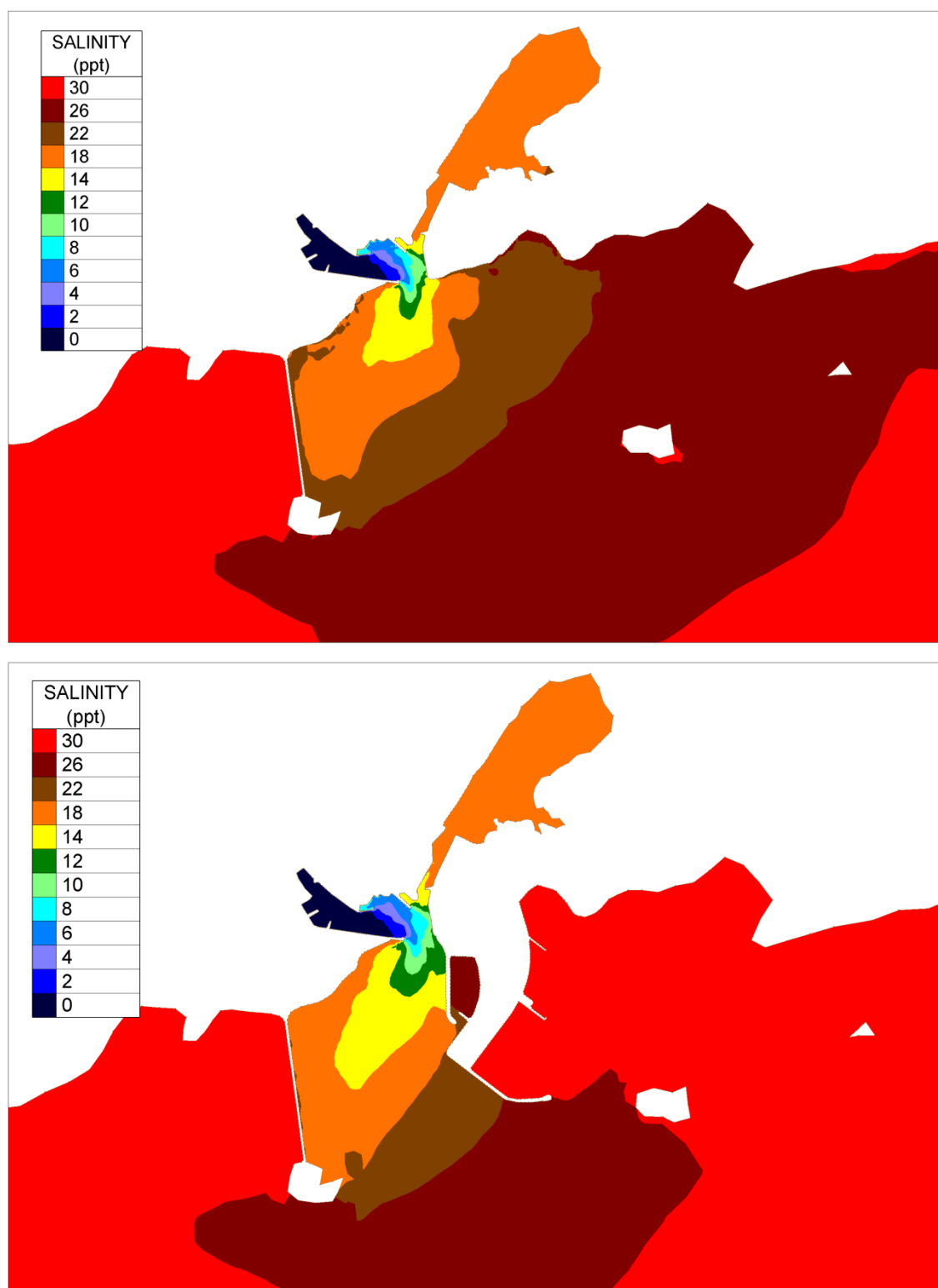
Figure Error! No text of specified style in document..82 Mean Salinity concentration in surface layer for existing and proposed cases under 90-percentile Corrib Flow (28.5cumec)
