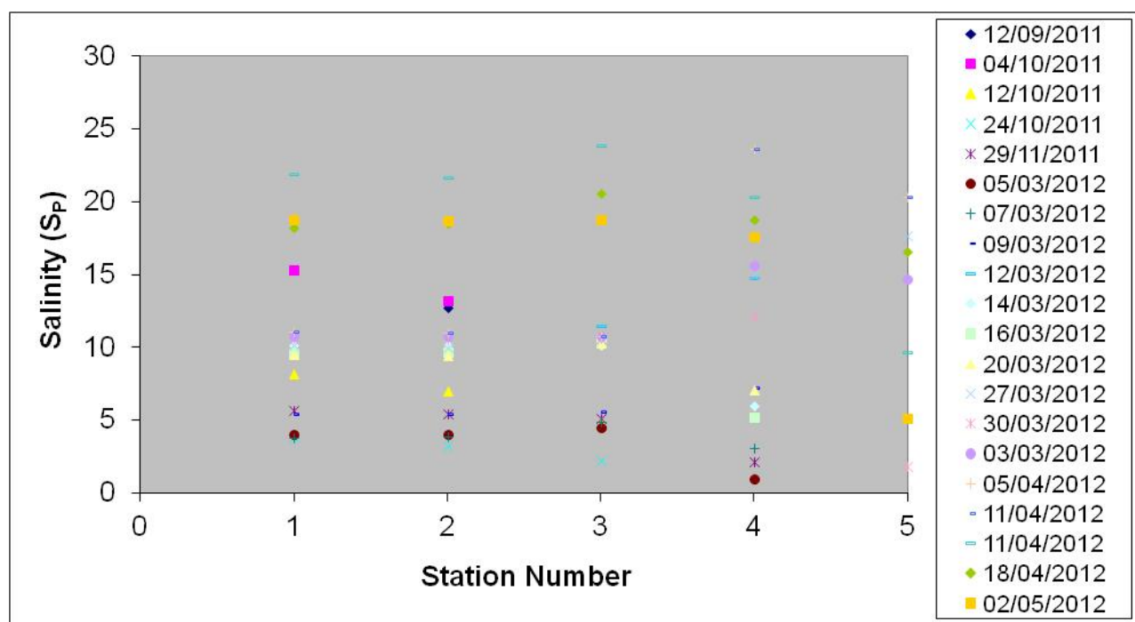
Figure Error! No text of specified style in document..69 Salinities measured over a series of dates at three stations in Renmore lagoon and two stations on Lough Atalia
