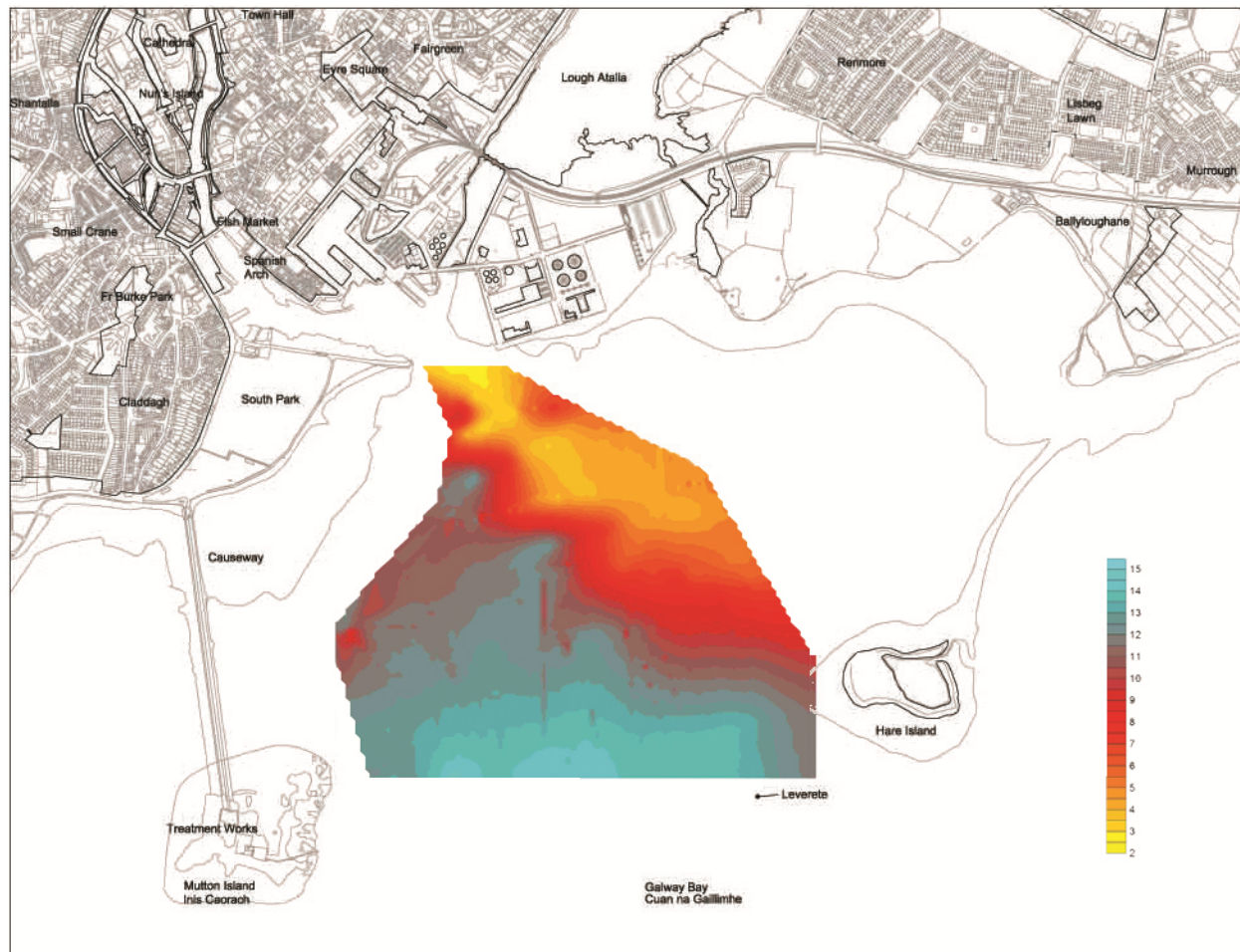
Figure Error! No text of specified style in document..64 Surface salinity contours
