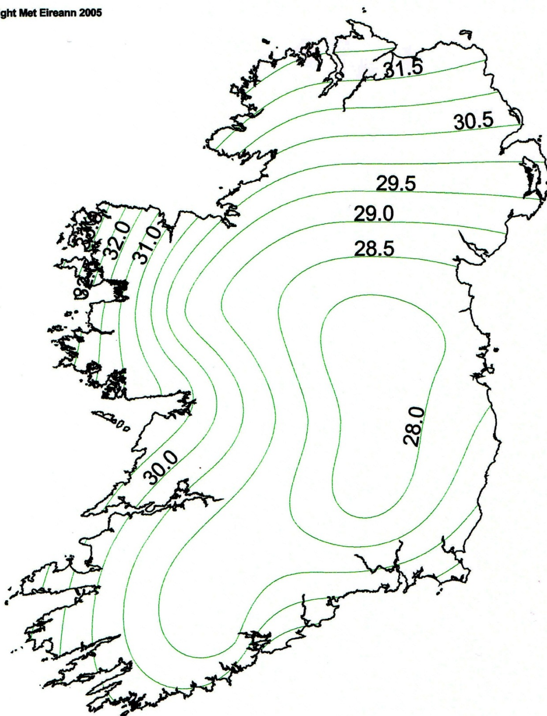
Figure Error! No text of specified style in document..126 10minute mean wind speed of 50year return period (Met Eireann 2005)
