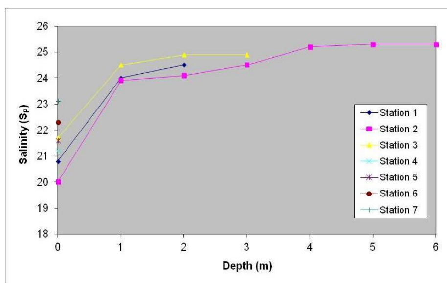
Figure Error! No text of specified style in document..68 L. Atalia salinity profiles at 7 stations in August 2011
