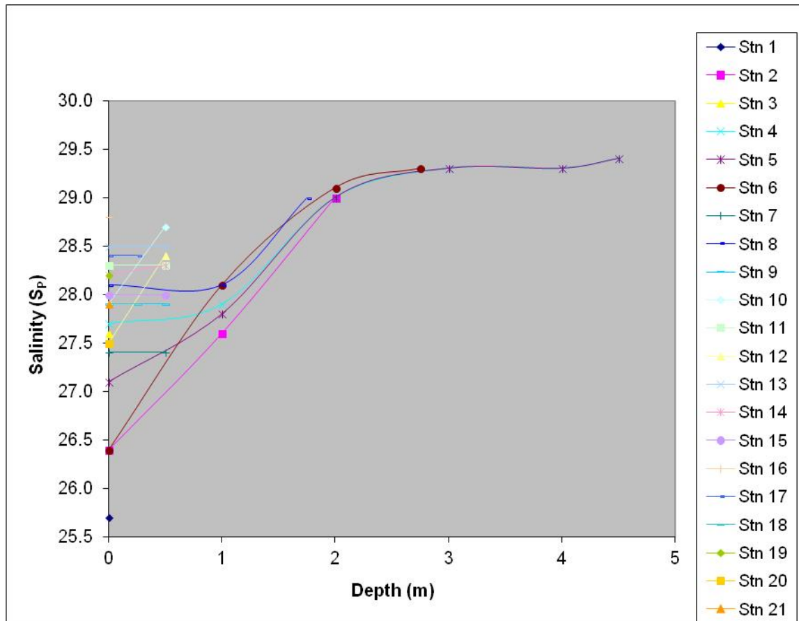
Figure Error! No text of specified style in document..74 Salinity profiles of Lough Atalia 04/05/2012 (carried out during 1.5 hours directly after low water, two days before the peak of a Spring tide)
