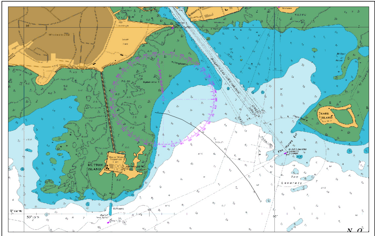
Figure Error! No text of specified style in document..66 The black line indicates a portion of a saltwater/freshwater front recorded at the Corrib estuary in 1984
