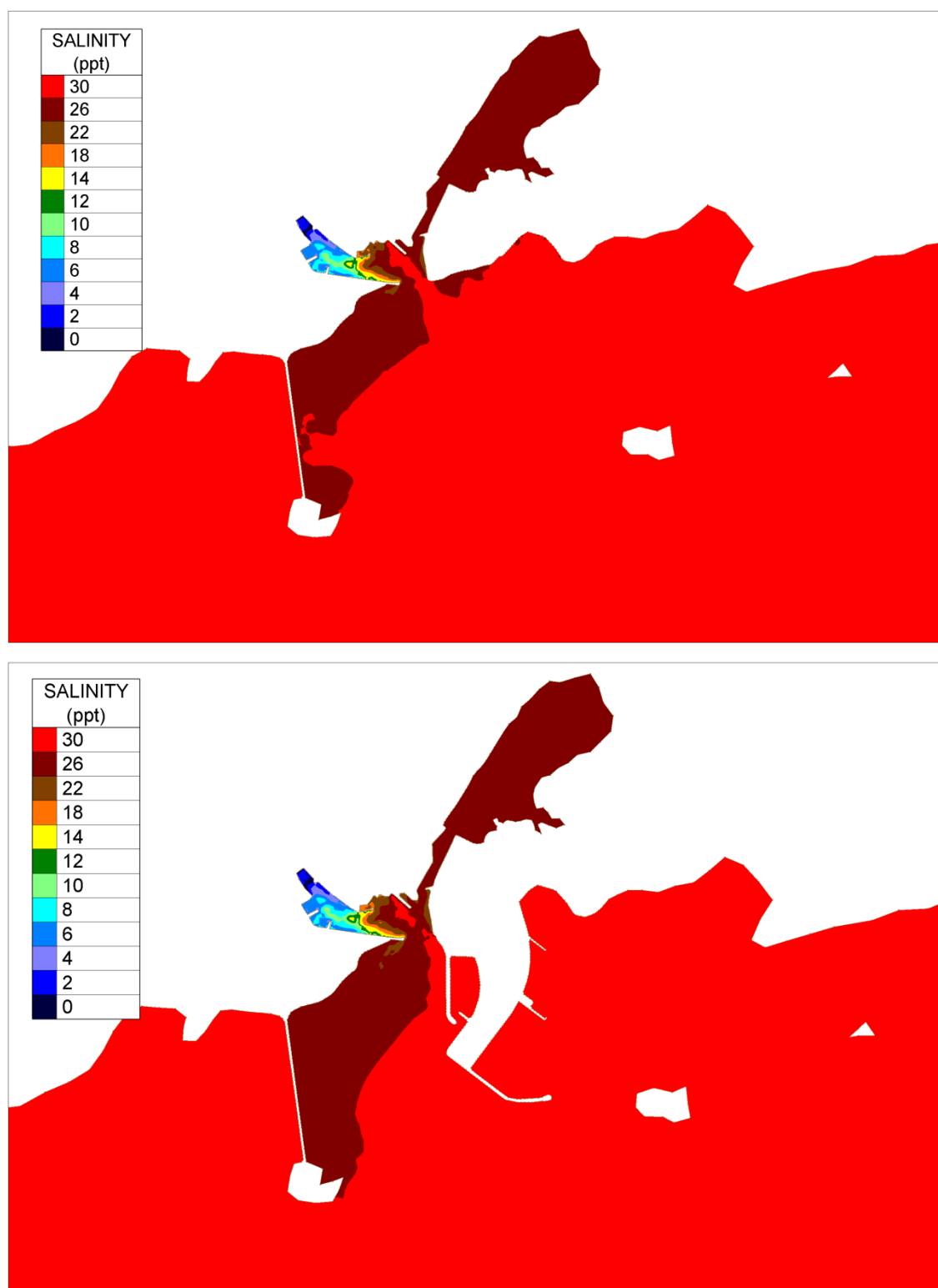
Figure Error! No text of specified style in document..78 Mean Salinity concentration in mid-depth layer for existing and proposed cases under 99-percentile Corrib Low Flow (9.1 cumec)
