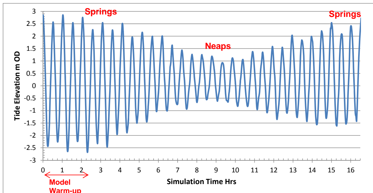
Figure Error! No text of specified style in document..75 Open Sea Tidal conditions used in salinity simulations
