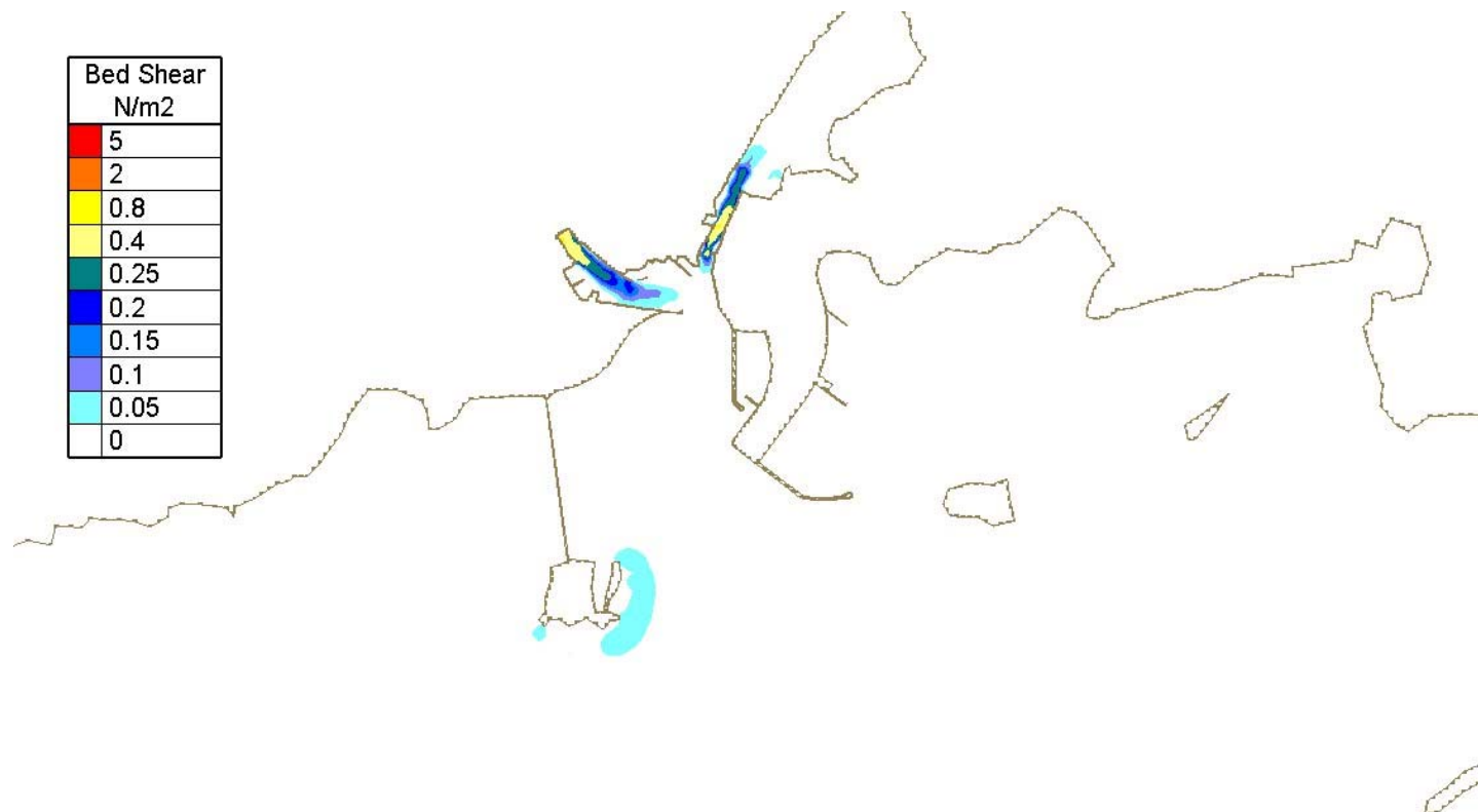
Figure Error! No text of specified style in document..24 - Computed bed shear at Highwater with new harbour extension – Spring Tide and Median River Corrib Flow (82 m 3 /s)
