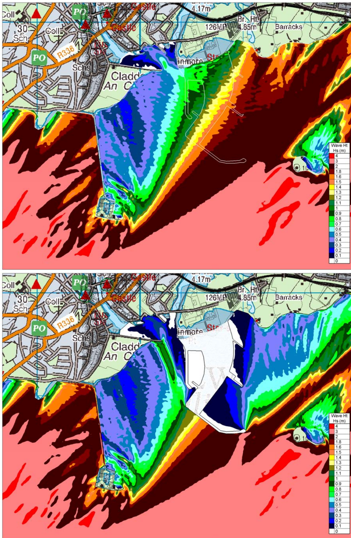
Figure Error! No text of specified style in document..134 ARTEMIS Significant Wave Heights for Atlantic Storm from the South-West for Existing and Proposed Case
