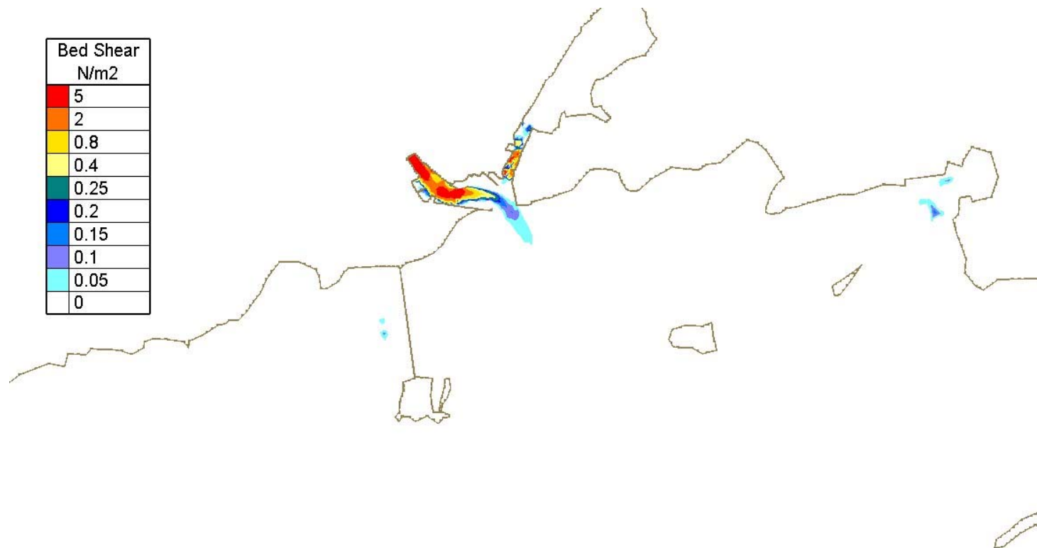
Figure Error! No text of specified style in document..27 - Computed bed shear at low water existing case without new harbour extension development – Neap Tide and Median River Corrib Flow (82 m 3 /s)
