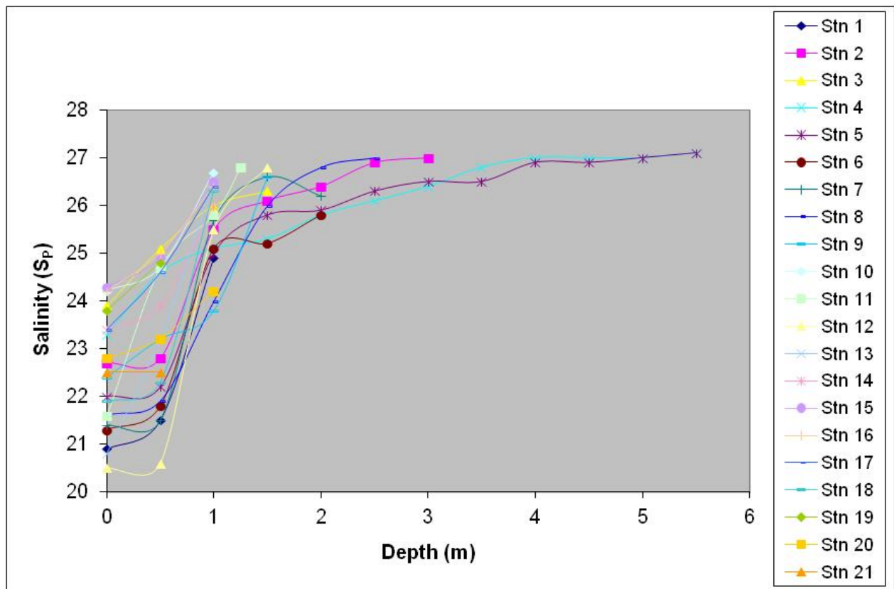
Figure Error! No text of specified style in document..71 Salinity profiles of Lough Atalia 10/04/2012 (carried out on an ebbing tide, from approximately 2 to three hours after high water, on a diminishing Spring tide i.e. four days after a full moon)
