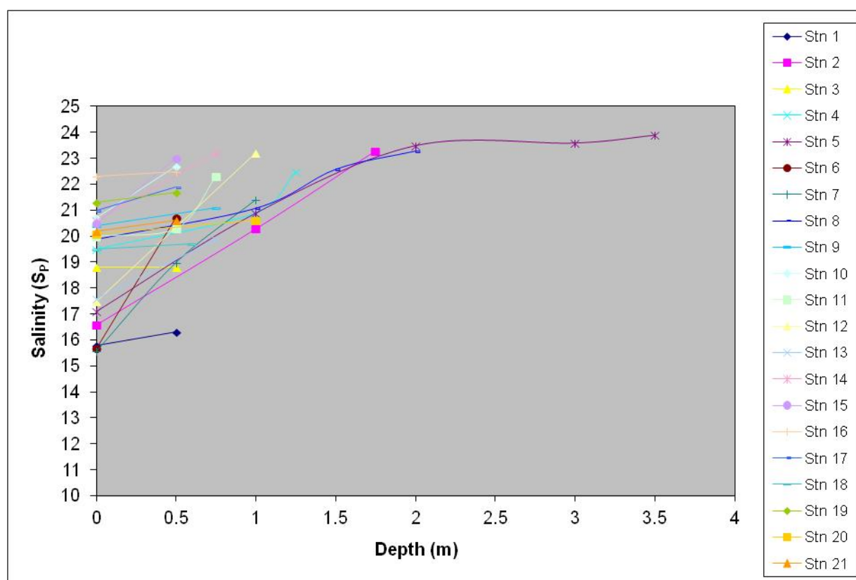
Figure Error! No text of specified style in document..73 Salinity profiles of Lough Atalia 19/04/2012 (was carried out approximately 15 minutes before to 40 minutes after low tide, two days before the peak of a Spring tide)
