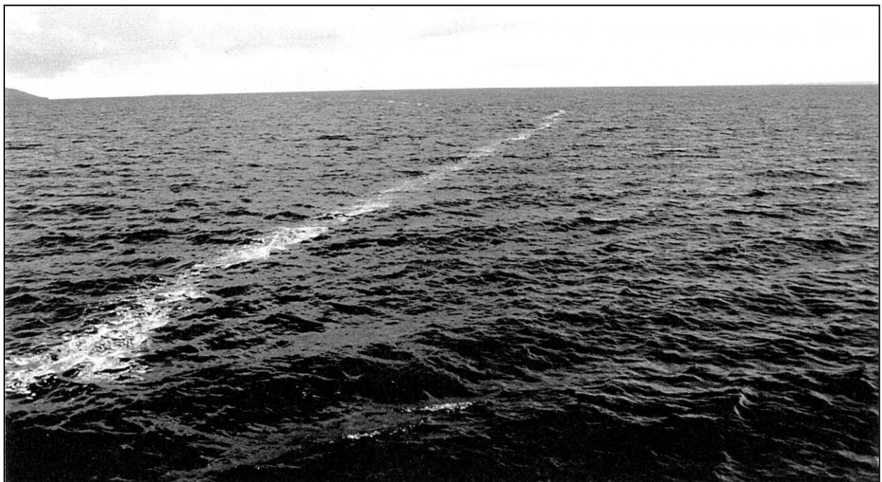
Figure Error! No text of specified style in document..65 Saltwater / Freshwater Front (halocline) observed in Galway Bay
