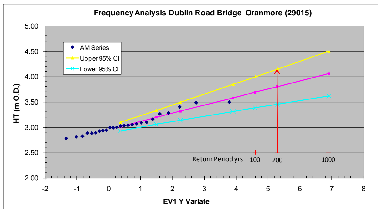
Figure Error! No text of specified style in document..147 EV1 Fit of the Oranmore AM highwater tidal series showing the statistical upper and lower 95-percentile confidence interval of the fit
