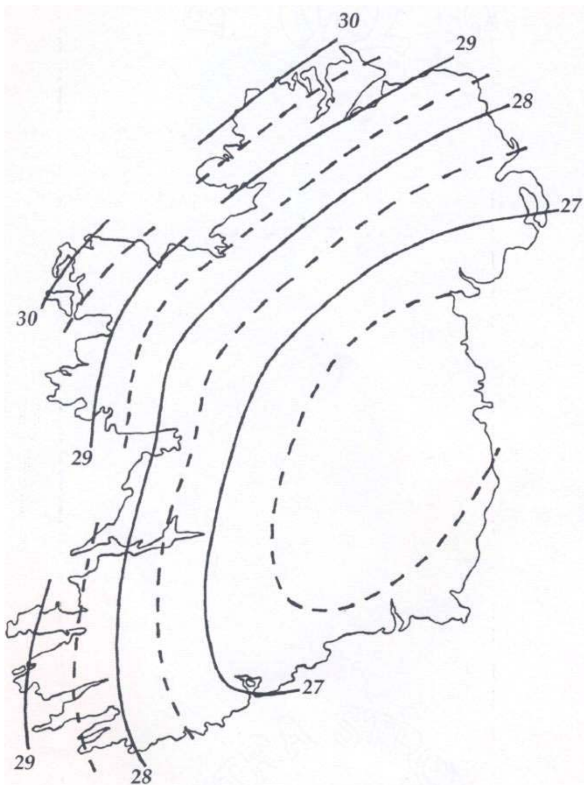
Figure Error! No text of specified style in document..125 Met Eireann 1 hour mean wind speed of 50year return period
