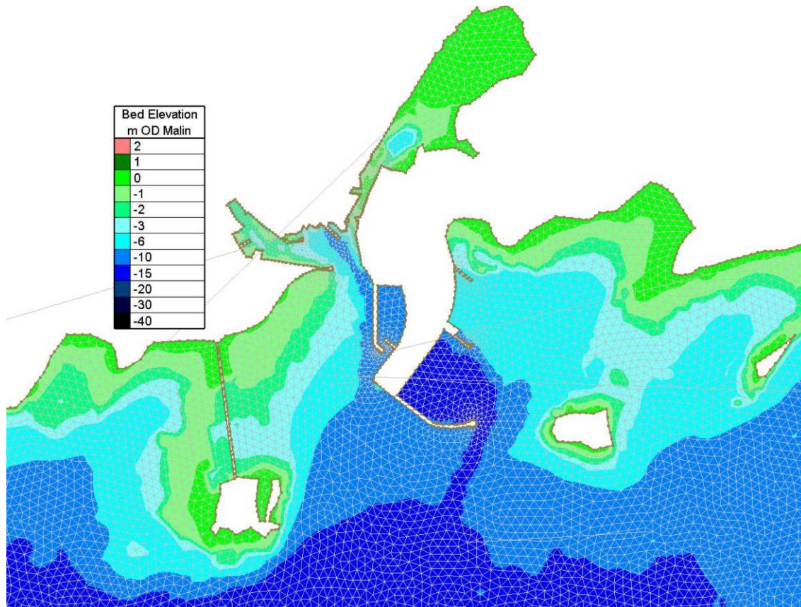
Figure Error! No text of specified style in document..151 Close-up view of model refinement in the vicinity of the proposed harbour development
