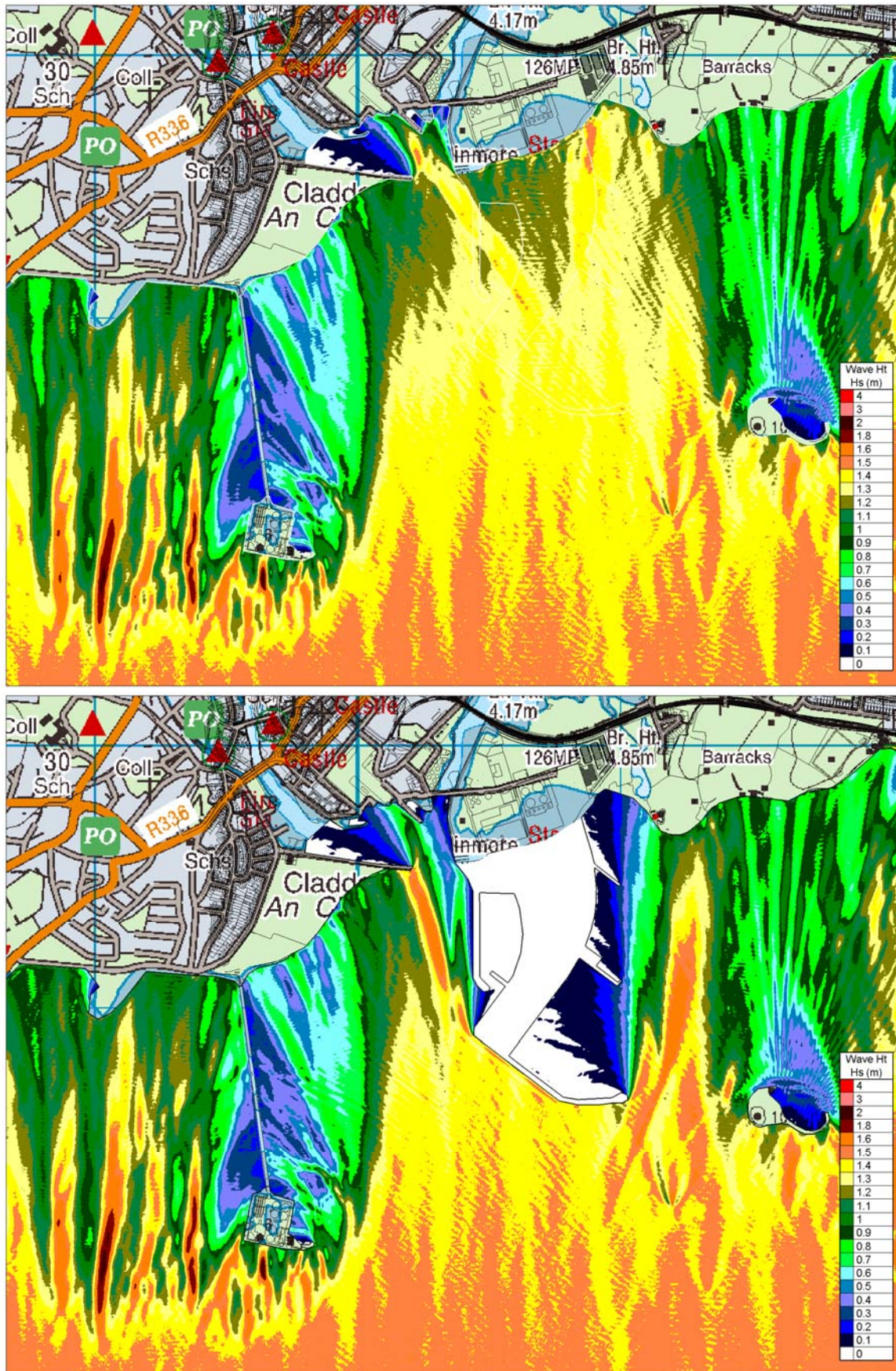
Figure Error! No text of specified style in document..136 ARTEMIS Significant Wave Heights for local Design Storm Waves from the South for Existing and Proposed Case
