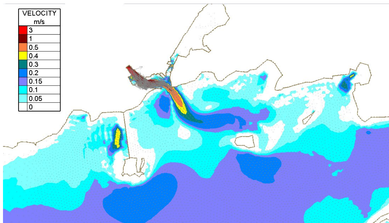
Figure Error! No text of specified style in document..15 - Depth averaged velocities Mid-Flood Spring tide and 100 year Corrib Flow
