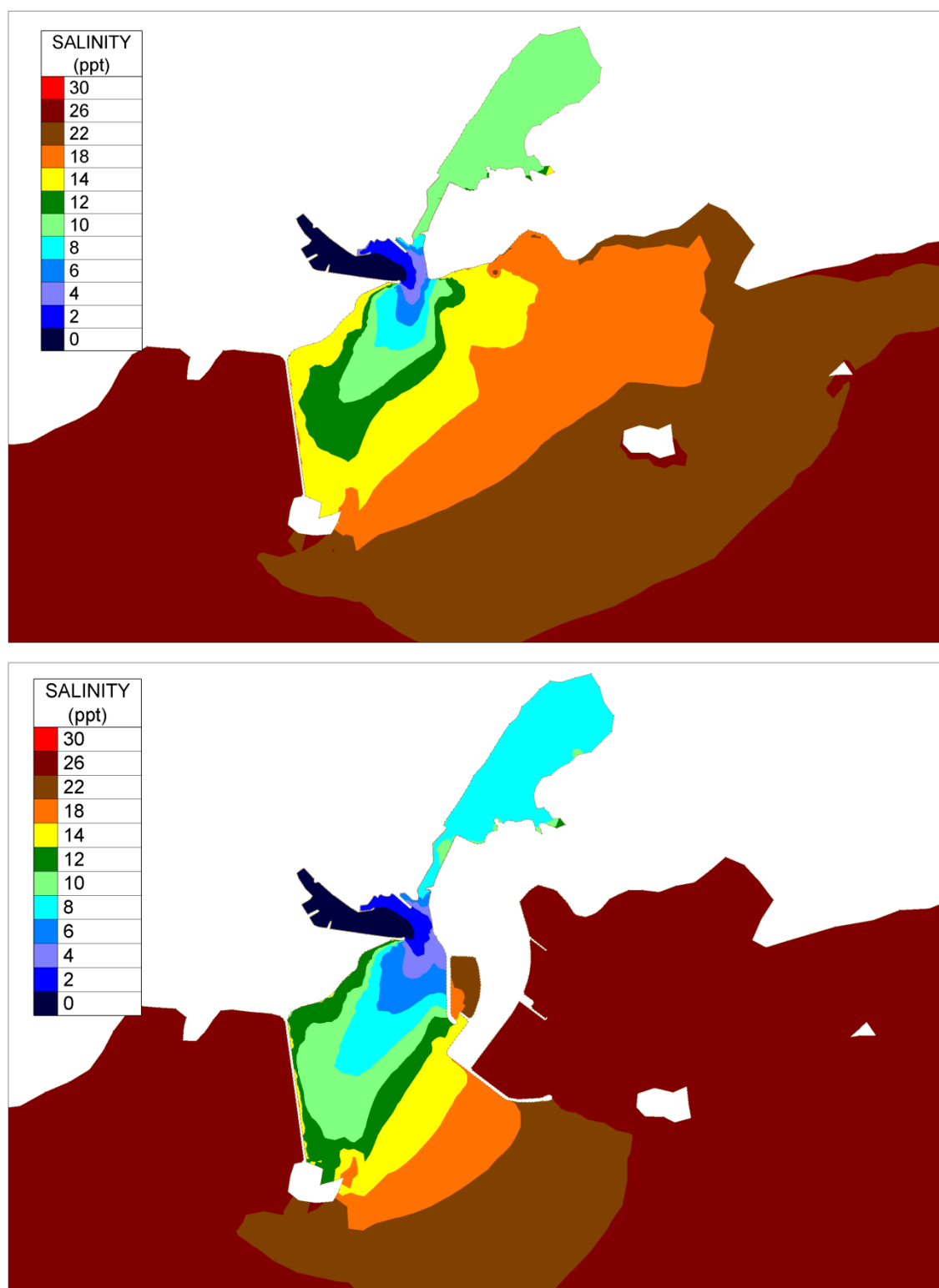
Figure Error! No text of specified style in document..85 Mean Salinity concentration in surface layer for existing and proposed cases under 50-percentile Corrib Flow (82cume)
