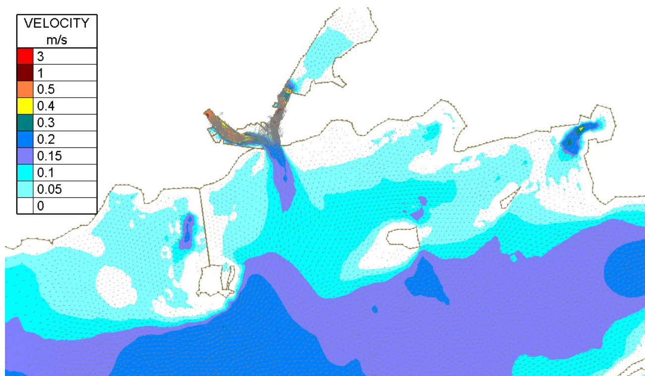
Figure Error! No text of specified style in document..5 - Depth averaged velocities Mid-ebb Spring tide Median Corrib Flow
