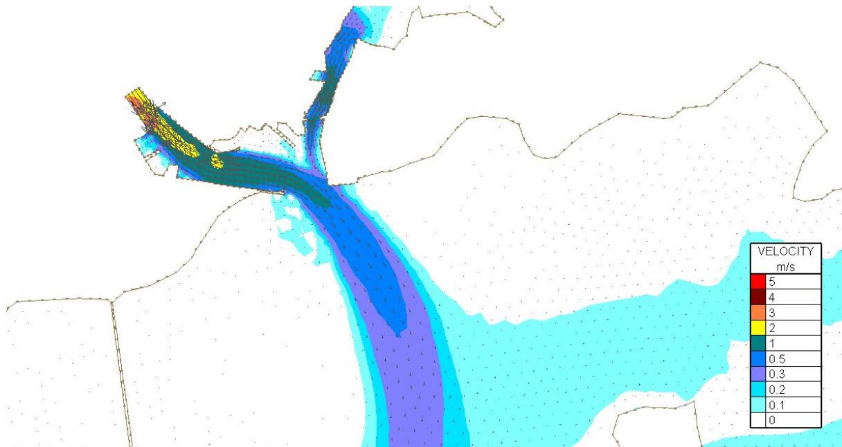
Figure Error! No text of specified style in document..169 Velocity Magnitudes at Mid-ebb (3.1hrs after highwater ) for Flood Simulation 3 - river plus 20% climate change and a 3.49m tide – Existing Case
