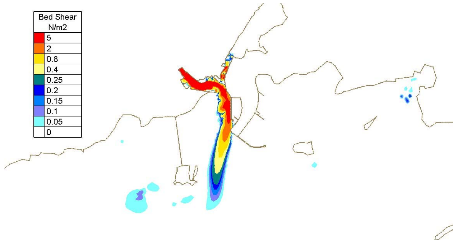
Figure Error! No text of specified style in document..36 - Computed bed shear at Low Water Spring Tide with 100 year Corrib Flood Flow with new harbour extension development
