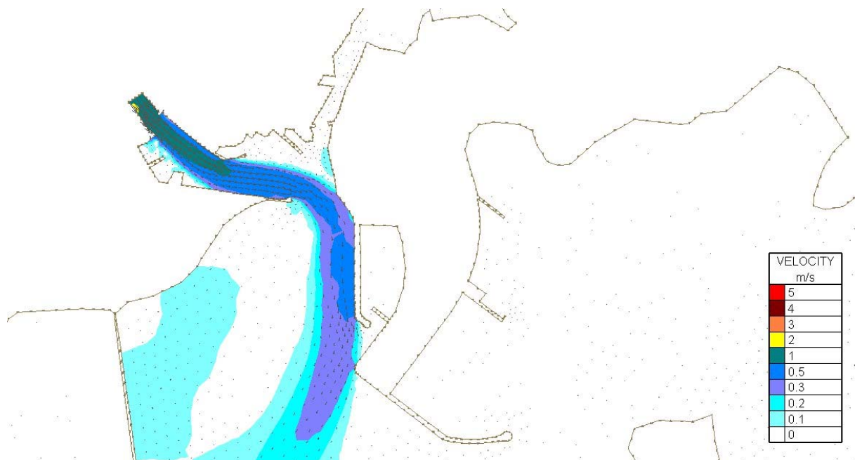
Figure Error! No text of specified style in document..184 Velocity Magnitudes at highwater for Flood Simulation 4 for Flood Simulation 1 – 100 year river flow and a tide of 4.146m (200 year tide) – Proposed Harbour Extension Case
