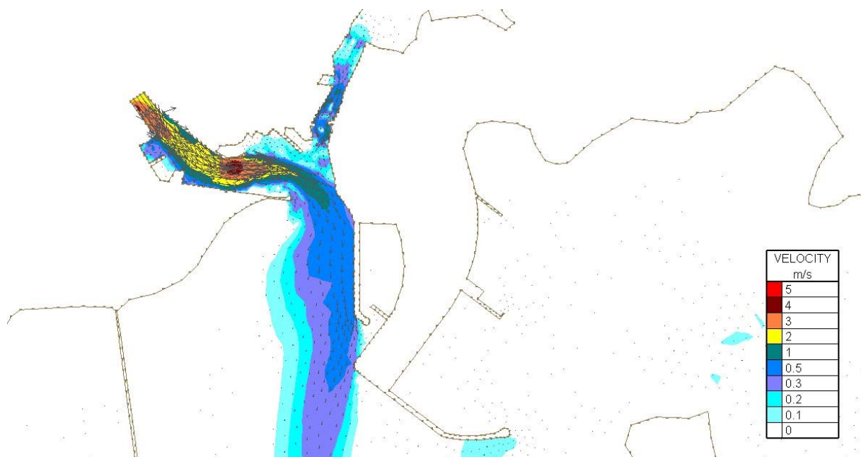
Figure Error! No text of specified style in document..164 Velocity Magnitudes at Low Water (6.2hrs after highwater Tide) for Flood Simulation 2 - 100 year river flow and a 3.49m tide – Proposed Harbour Extension Case
