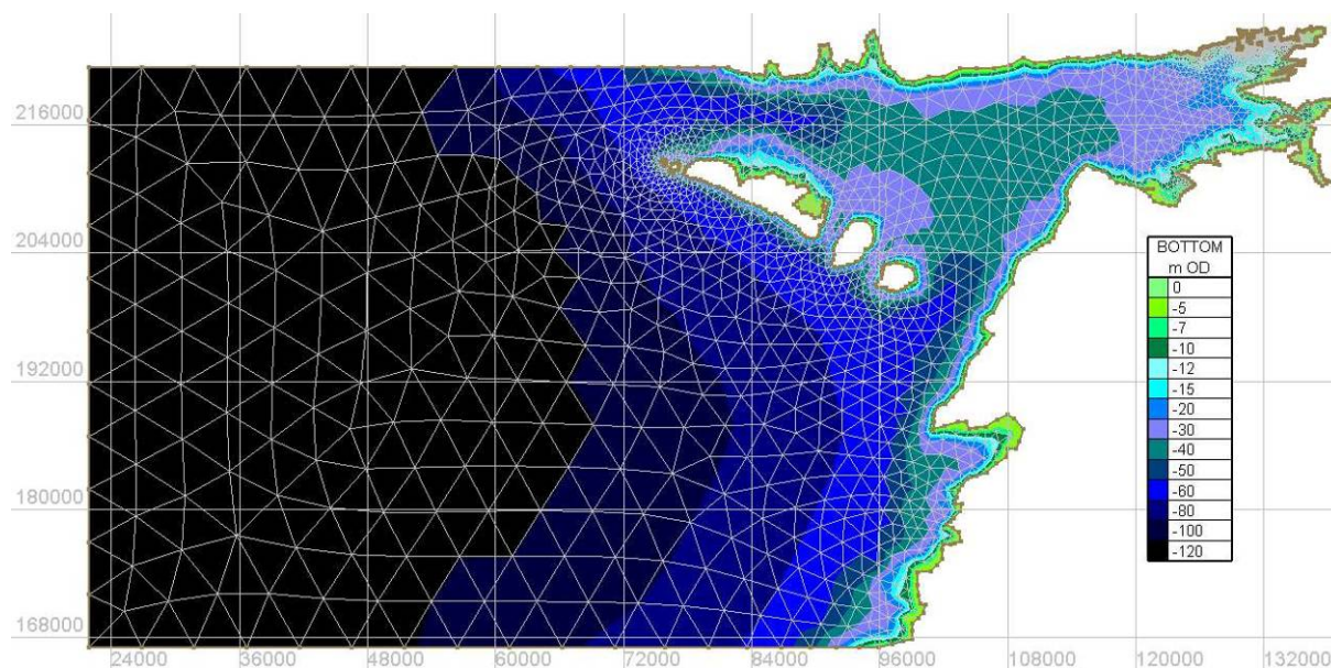
Figure Error! No text of specified style in document..127 TOMAWAC Spectral Wave Model Domain
