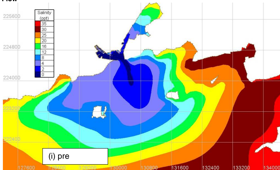
Figure Error! No text of specified style in document..122 Tidal Average Salinity –Neap Tides –Corrib Low Flow
