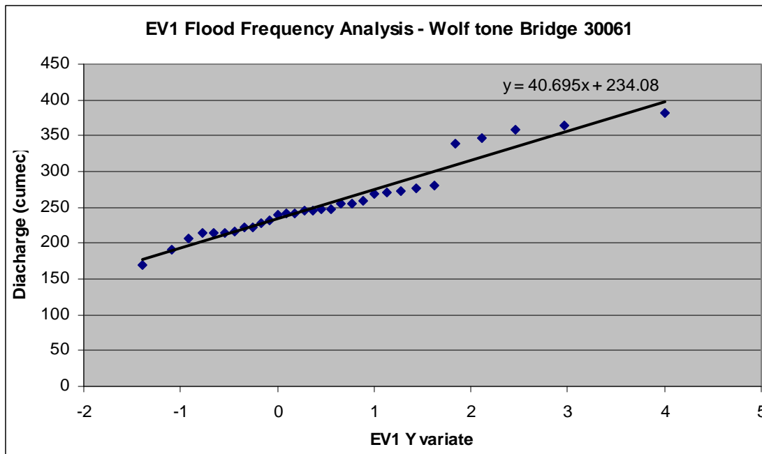
Figure Error! No text of specified style in document..149 Flood Flow Frequency Analysis – River Corrib at Wolf Tone Bridge Gauge
