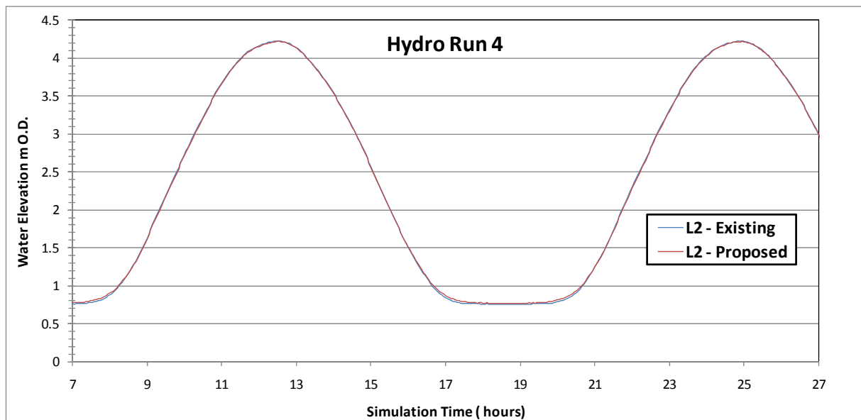
Figure Error! No text of specified style in document..205 Flood level comparison between existing and proposed for Hydrodynamic Simulation No. 4 at reference site 2 in Claddagh Basin
