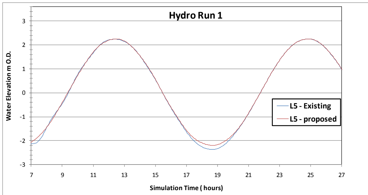
Figure Error! No text of specified style in document..190 Flood level comparison between existing and proposed for Hydrodynamic Simulation No. 1 at reference site 5 – new dredge channel at Marina Breakwater
