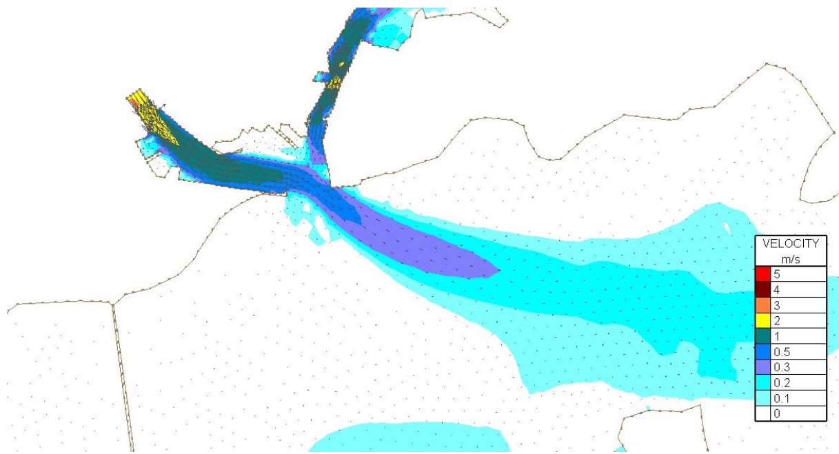
Figure Error! No text of specified style in document..181 Velocity Magnitudes at Mid Flood (3.1hrs before highwater Tide) for Flood Simulation 4 – 100 year river flow and a tide of 4.146m (200 year tide) – Existing Case
