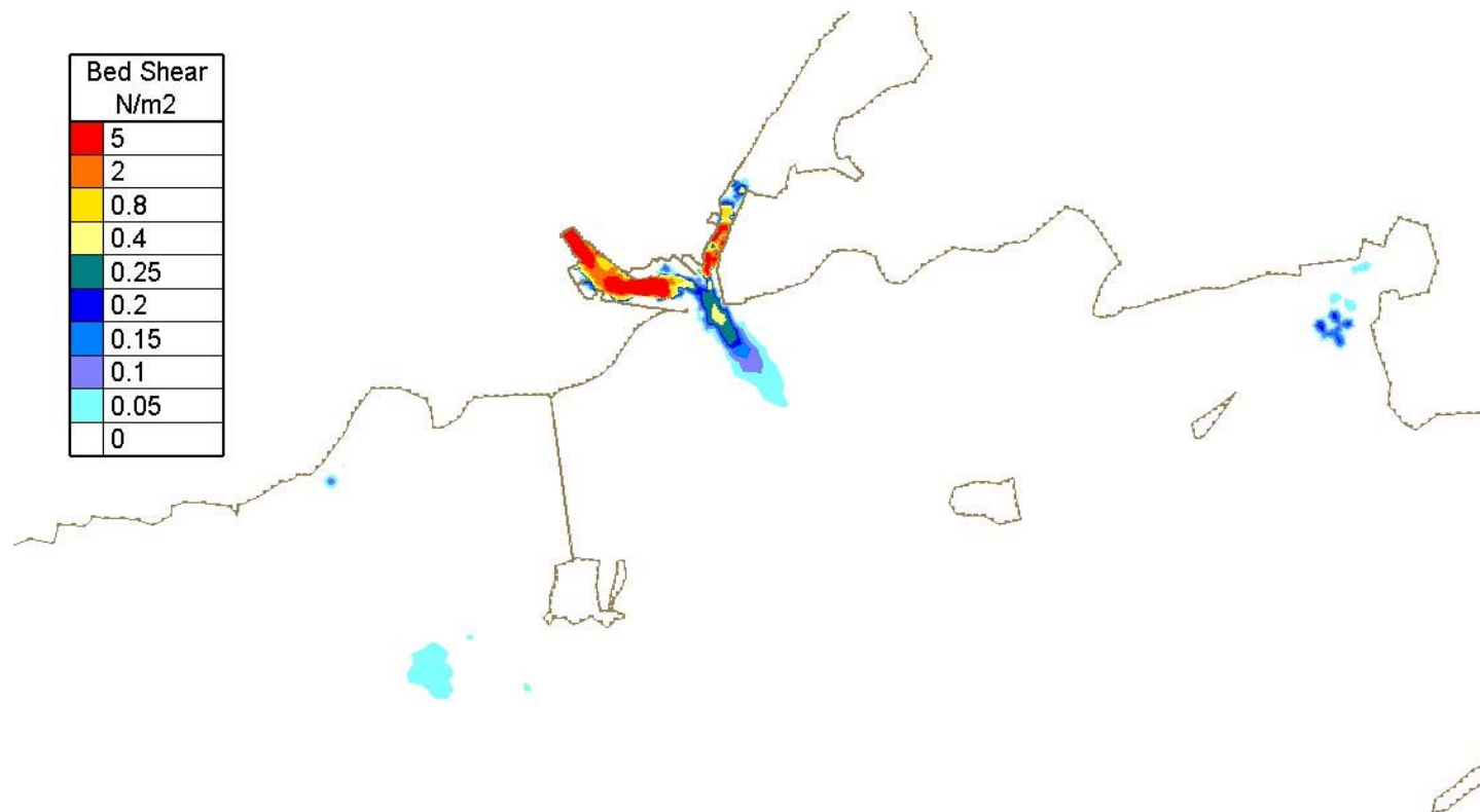
Figure Error! No text of specified style in document..19 - Computed bed shear at low water for existing case – Spring Tide and Median River Corrib Flow (82 m³/s)
