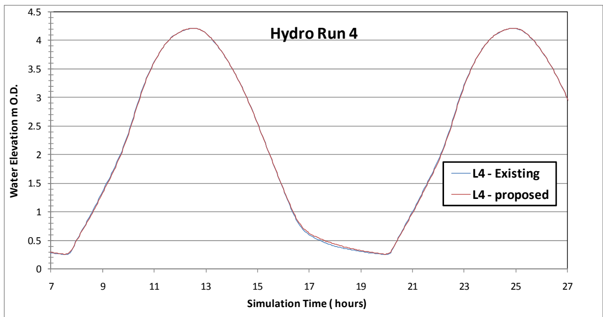
Figure Error! No text of specified style in document..207 Flood level comparison between existing and proposed for Hydrodynamic Simulation No. 4 at reference site 4 – entrance channel to Lough Atalia
