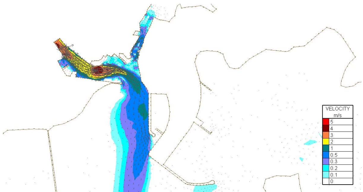
Figure Error! No text of specified style in document..172 Velocity Magnitudes at Low Water (6.2hrs after highwater Tide) for Flood Simulation 3- river plus 20% climate change and a 3.49m tide – Proposed Harbour Extension Case
