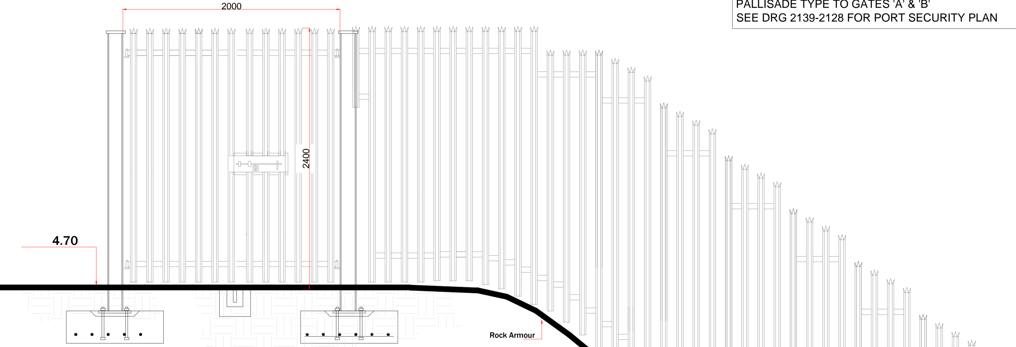
ELEVATION OF SECURITY FENCE & GATE 'A' & 'B'
