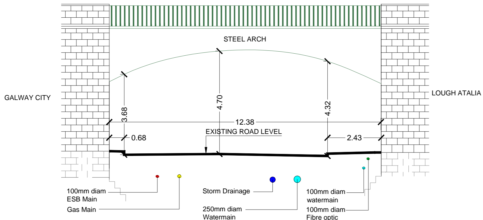
SOUTH WEST ELEVATION Scale @ A1 1:100 A3 1:200
