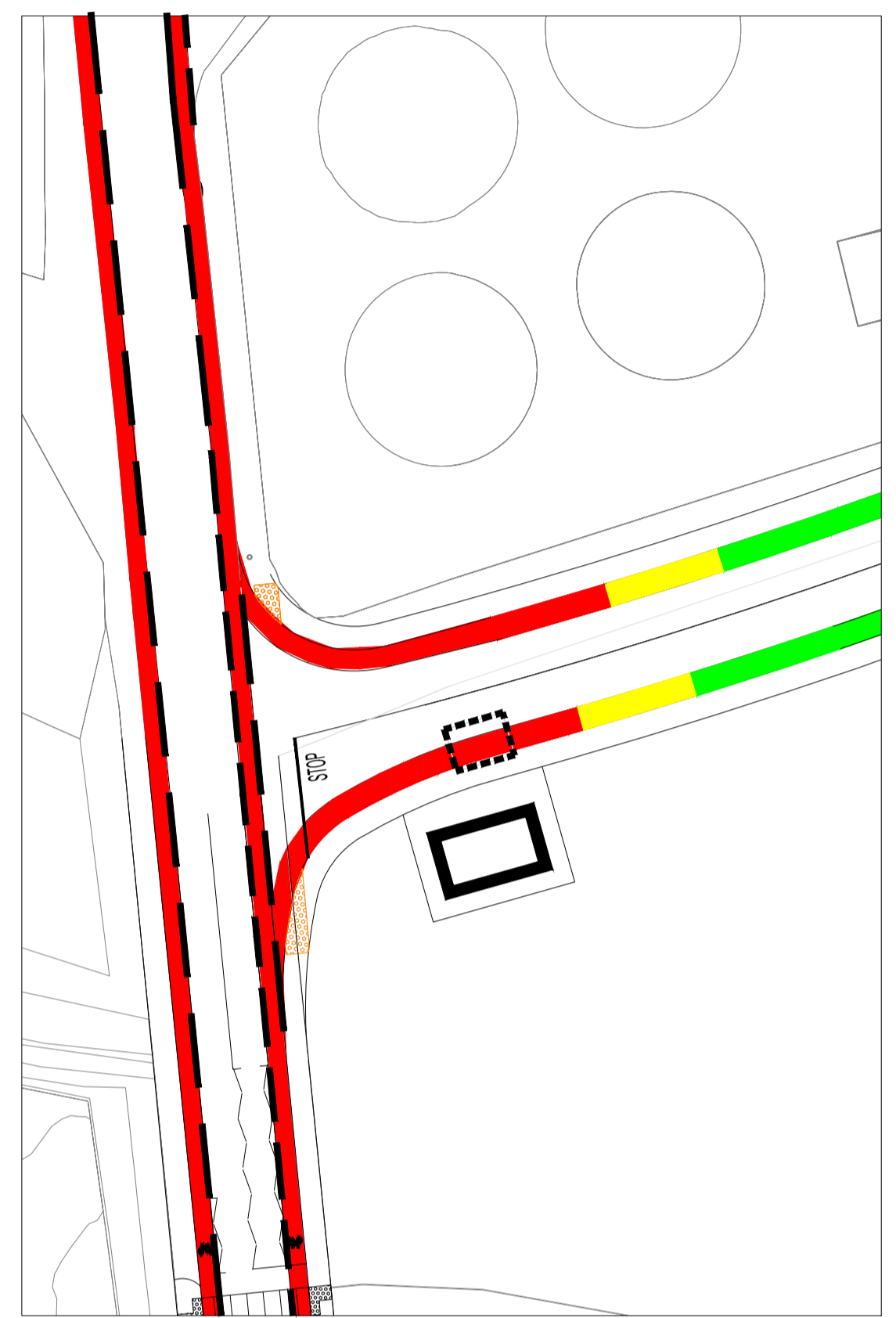
CYCLE LANE JUNCTION DETAIL Scale A1 1/250 A3 1/500
